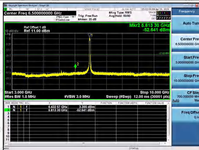
11AX40SISO-Ant1-6445-3000~10000-PASS
