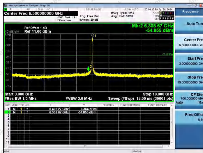
11AX40SISO-Ant1-6485-3000~10000-PASS
