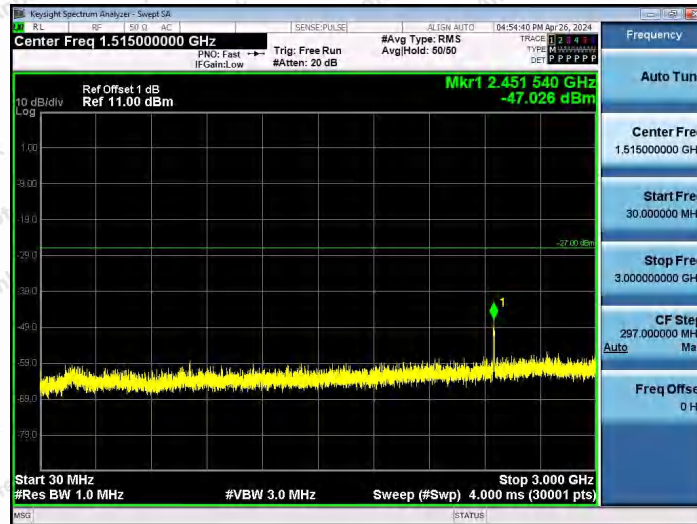
11AX40SISO-Ant1-5965-30~3000-PASS
