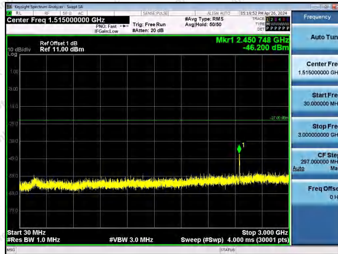
11AX40SISO-Ant1-7085-30~3000-PASS
