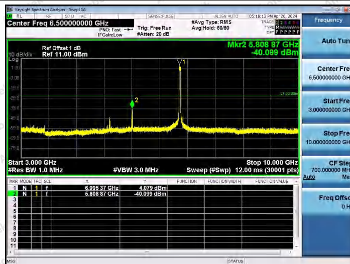
11AX40SISO-Ant1-7005-3000~10000-PASS
