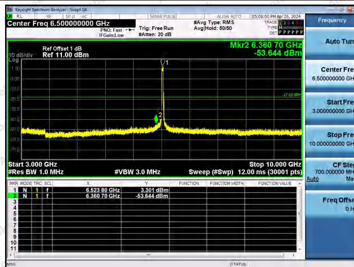
11AX40SISO-Ant1-6525-3000~10000-PASS
