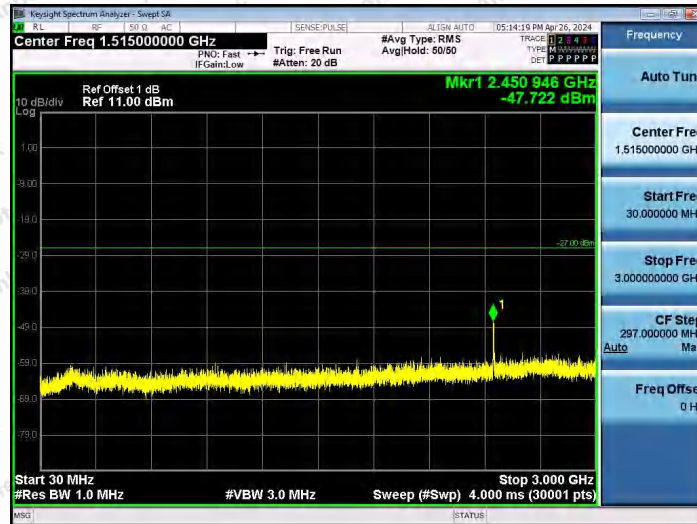
11AX40SISO-Ant1-6845-30~3000-PASS
