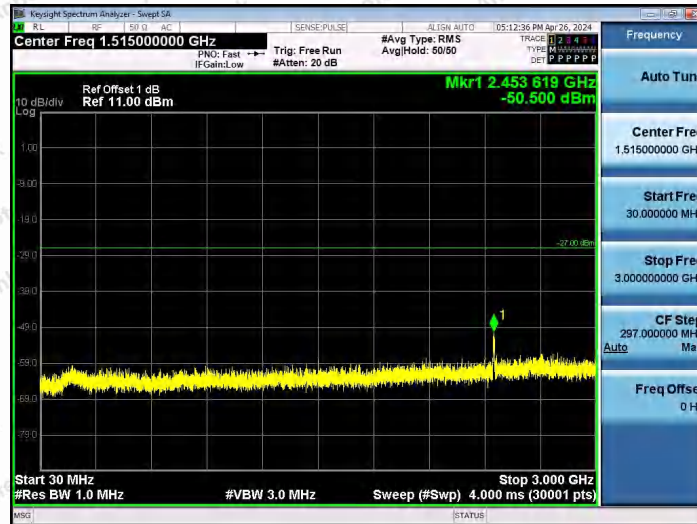
11AX40SISO-Ant1-6685-30~3000-PASS
