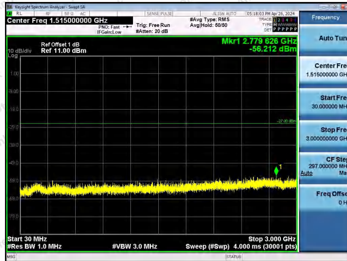
11AX40SISO-Ant1-7005-30~3000-PASS
