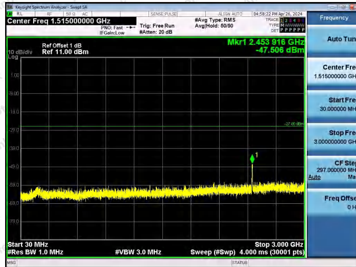
11AX40SISO-Ant1-6165-30~3000-PASS
