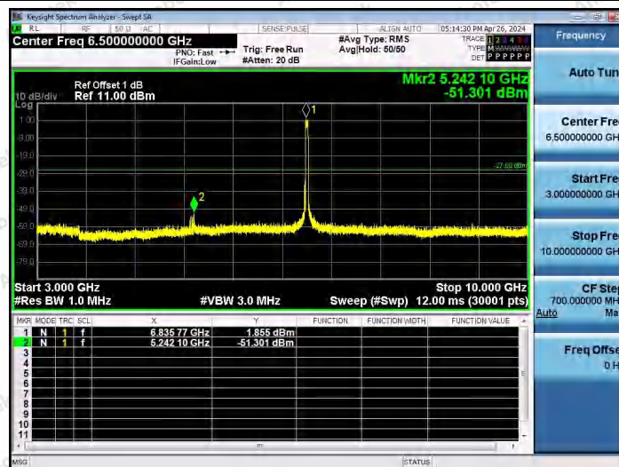
11AX40SISO-Ant1-6845-3000~10000-PASS
