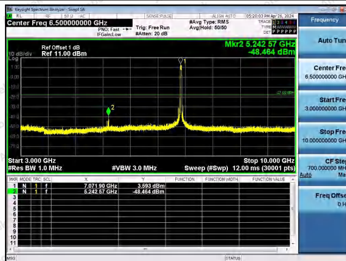
11AX40SISO-Ant1-7085-3000~10000-PASS
