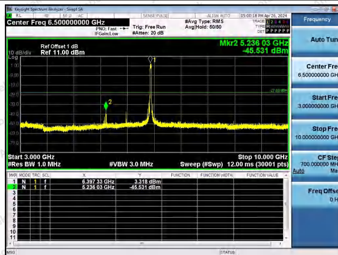
11AX40SISO-Ant1-6405-3000~10000-PASS
