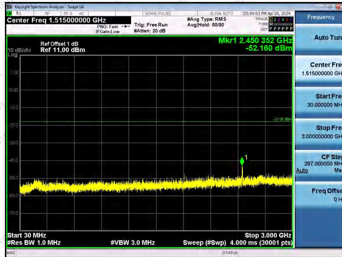
11AX40SISO-Ant1-6485-30~3000-PASS
