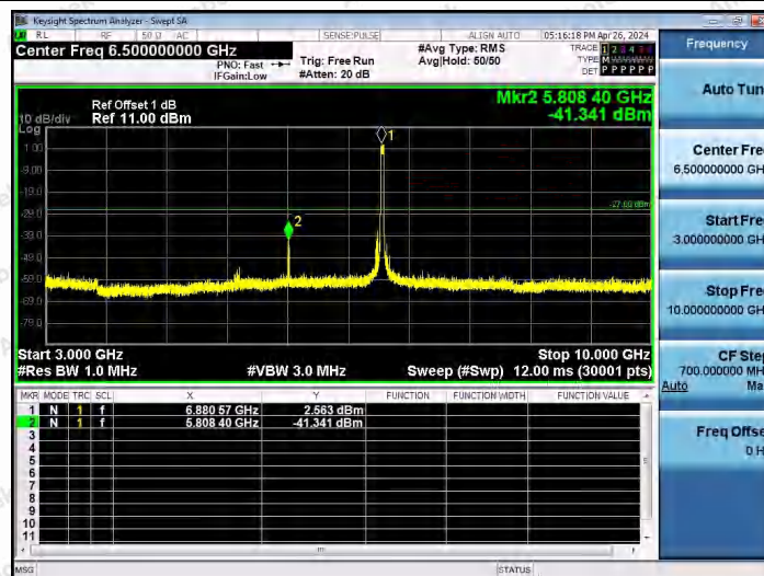
11AX40SISO-Ant1-6885-3000~10000-PASS
