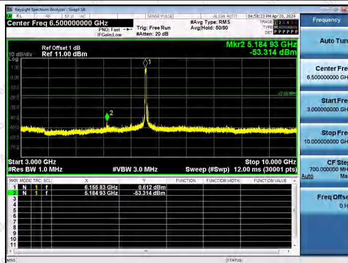
11AX40SISO-Ant1-6165-3000~10000-PASS
