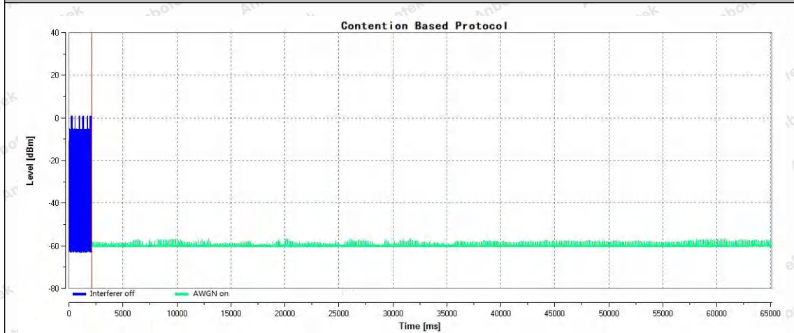
11AX20SISO-Ant1-6895-6895-PASS
