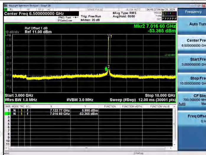
11AX20SISO-Ant1-7115-3000~10000-PASS
