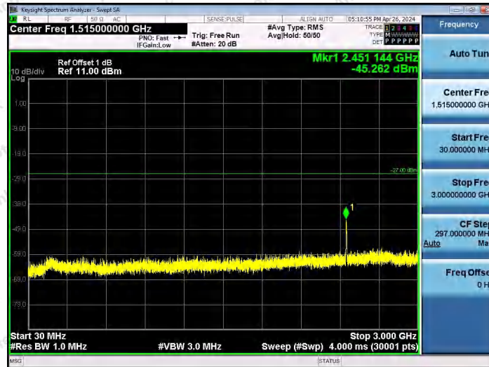
11AX40SISO-Ant1-6565-30~3000-PASS
