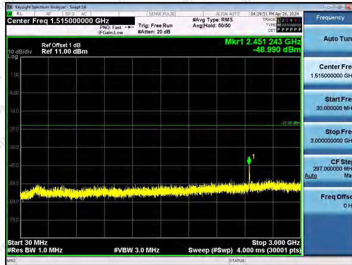
11AX20SISO-Ant1-6875-30~3000-PASS
