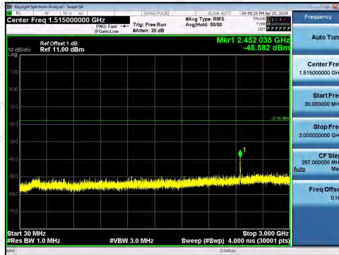
11AX20SISO-Ant1-7115-30~3000-PASS
