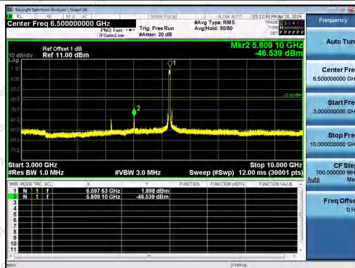
11AX40SISO-Ant1-6685-3000~10000-PASS
