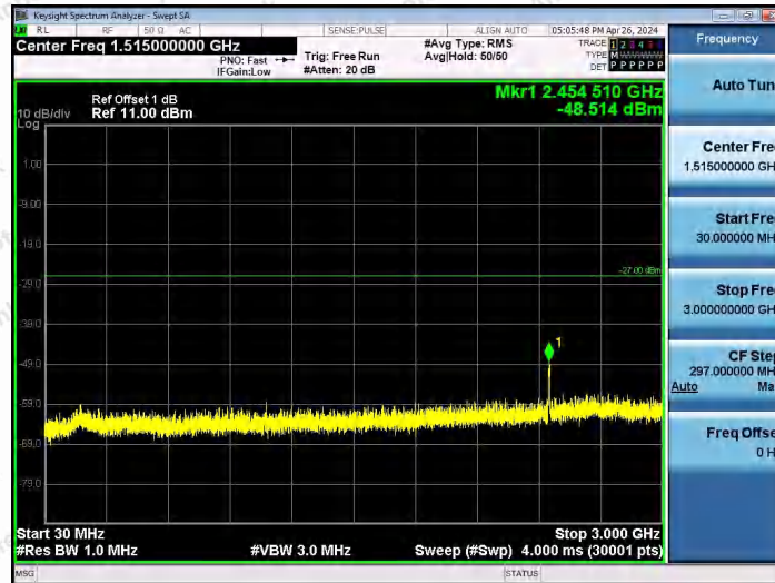
11AX40SISO-Ant1-6525-30~3000-PASS
