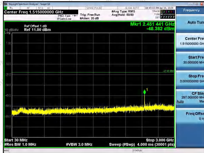
11AX20SISO-Ant1-7015-30~3000-PASS
