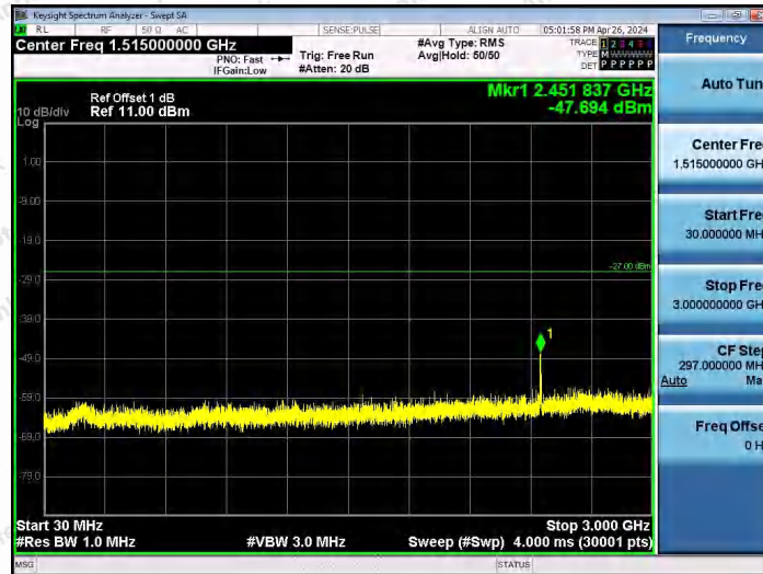
11AX40SISO-Ant1-6445-30~3000-PASS
