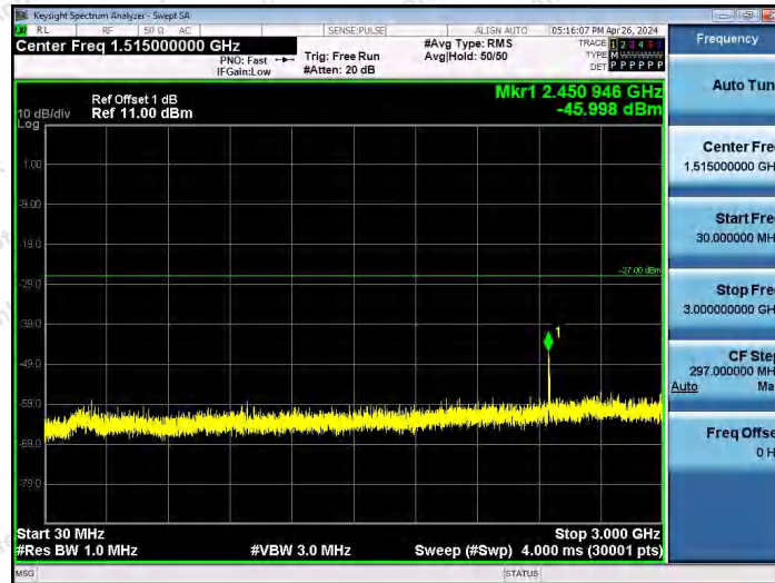
11AX40SISO-Ant1-6885-30~3000-PASS
