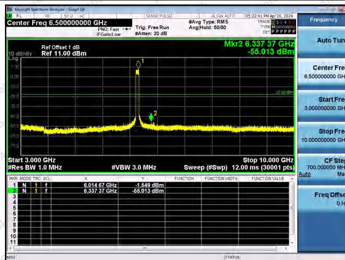
11AX80SISO-Ant1-5985-3000~10000-PASS
