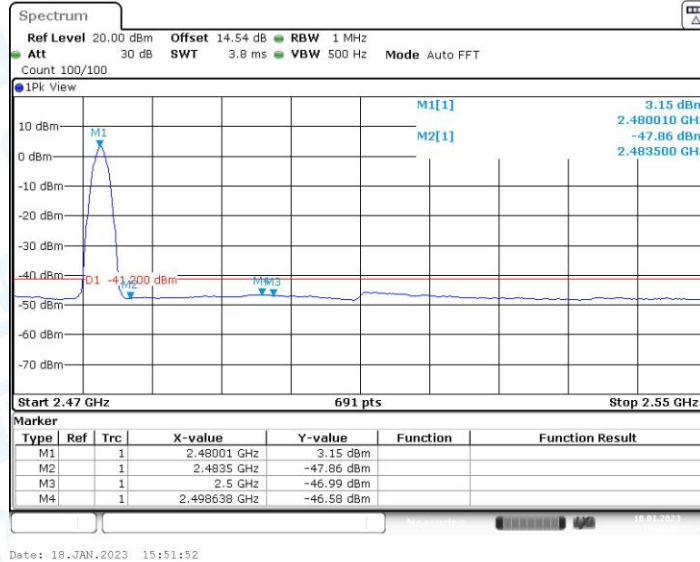
2DH5_Ant1_High_2480_Peak
