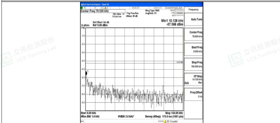
Band2-1.4MHz-16QAM-18607-1RB#0-0.009~0.15-PASS
