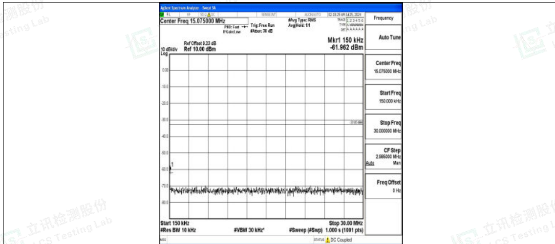
Band2-1.4MHz-QPSK-19193-1RB#0-0.15~30-PASS
