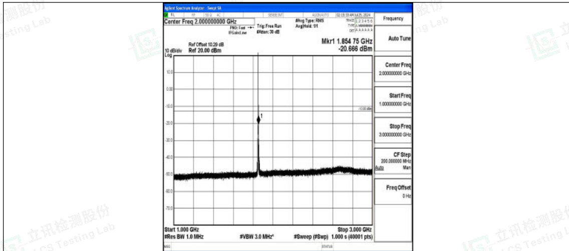
Band2-1.4MHz-QPSK-18607-1RB#0-1000~3000-PASS
