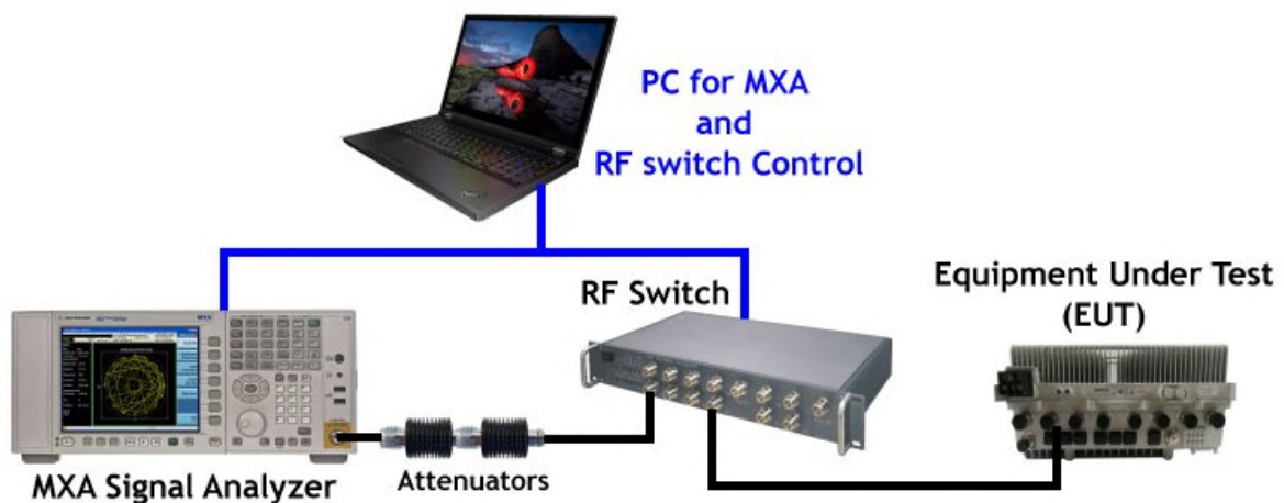
Figure 1. Setup Diagrams of Conducted Test
