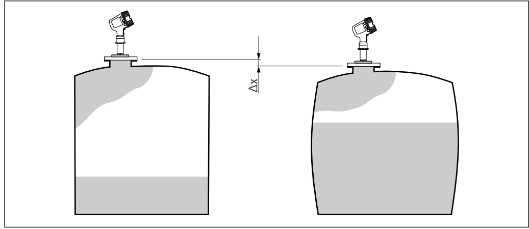
15 Movement \Delta x of the Gauge Reference Height due to the bulging of the tank shell caused by hydrostatic pressure
