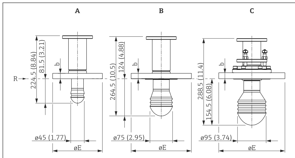
10 Antenna size; unit of measurement: mm (in)
