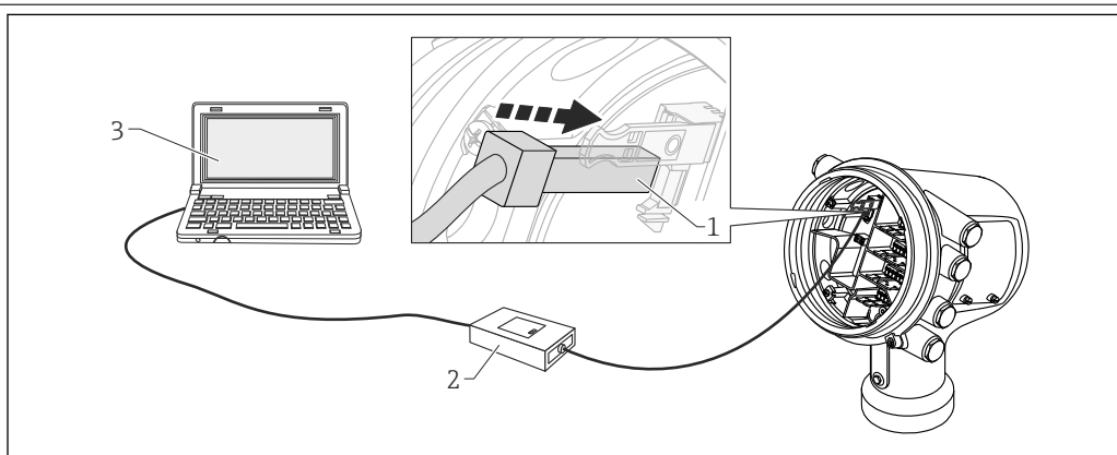
14 Operation via service interface
