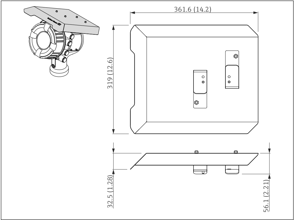
16 Weather protection cover; dimensions: mm (in)
