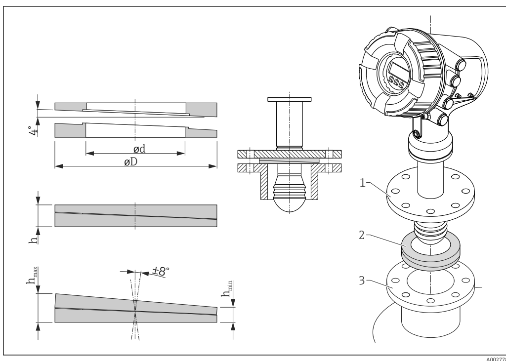
17 Adjustable seal used to align the device by \pm 8^\circ
