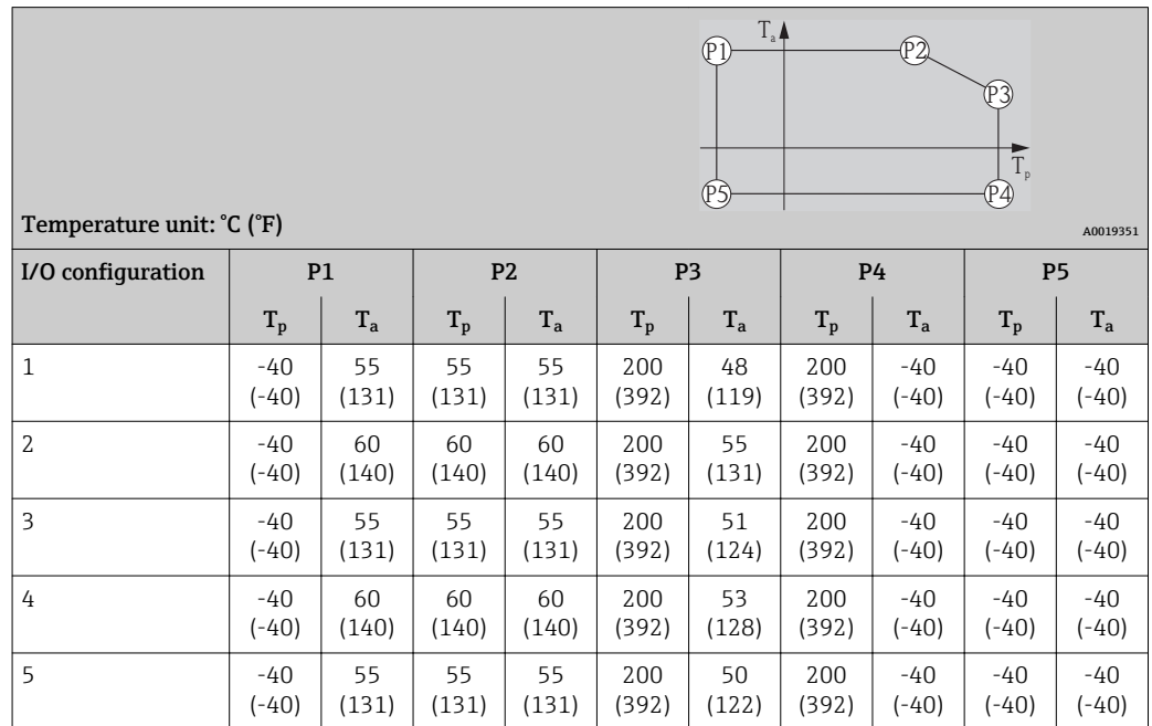
Ambient temperature limits for NMR81
