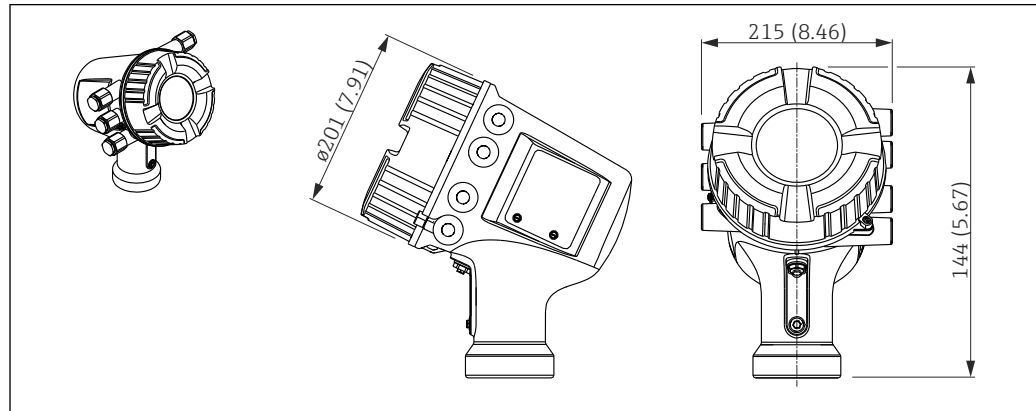
9 Dimensions of the electronics housing; unit of measurement: mm (in); adapters for cable entries are not taken into account in this drawing.
