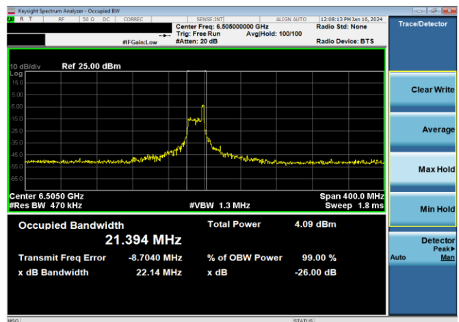
Plot 7-30. 26dB & 99% Bandwidth Plot Antenna WF5B (160MHz 802.11ax RU26 (UNII Band 6) – Ch. 111)
