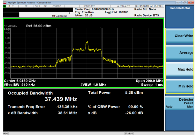
Plot 7-58. 26dB & 99% Bandwidth Plot Antenna WF5B (80MHz 802.11ax RU26 (UNII Band 8) - Ch. 199)
