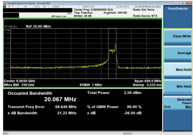
Plot 7-47. 26dB & 99% Bandwidth Plot Antenna WF5B (160MHz 802.11ax RU26 (UNII Band 7) – Ch. 143)
