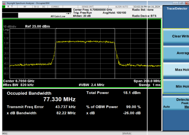
Plot 7-44. 26dB & 99% Bandwidth Plot Antenna WF5B (80MHz 802.11ax RU996 (UNII Band 7) – Ch. 151)
