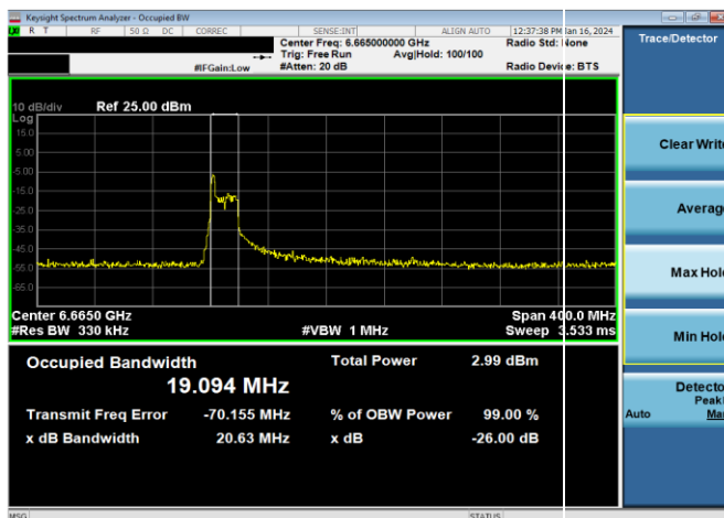
Plot 7-45. 26dB & 99% Bandwidth Plot Antenna WF5B (160MHz 802.11ax RU26 (UNII Band 7) – Ch. 143)
