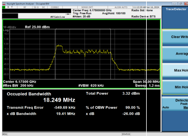
Plot 7-1. 26dB & 99% Bandwidth Plot Antenna WF5B (20MHz 802.11ax RU26 (UNII Band 5) – Ch. 45)
