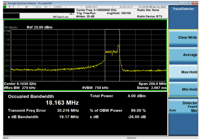
Plot 7-11. 26dB & 99% Bandwidth Plot Antenna WF5B (80MHz 802.11ax RU26 (UNII Band 5) – Ch. 39)
