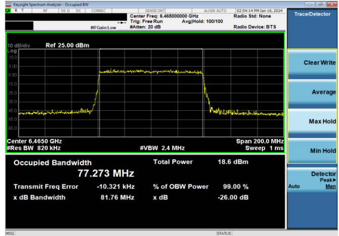
Plot 7-28. 26dB & 99% Bandwidth Plot Antenna WF5B (80MHz 802.11ax RU996 (UNII Band 6) – Ch. 103)
