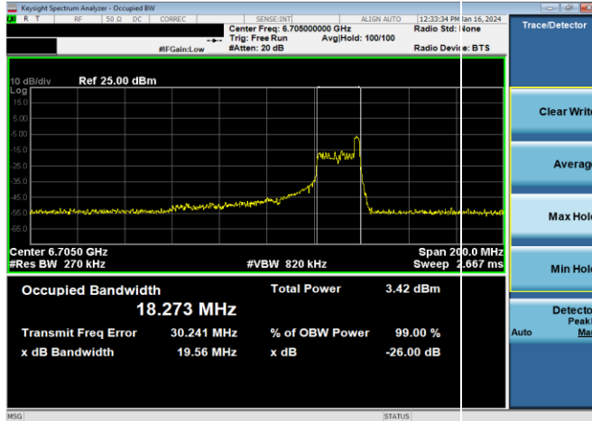
Plot 7-43. 26dB & 99% Bandwidth Plot Antenna WF5B (80MHz 802.11ax RU26 (UNII Band 7) – Ch. 151)
