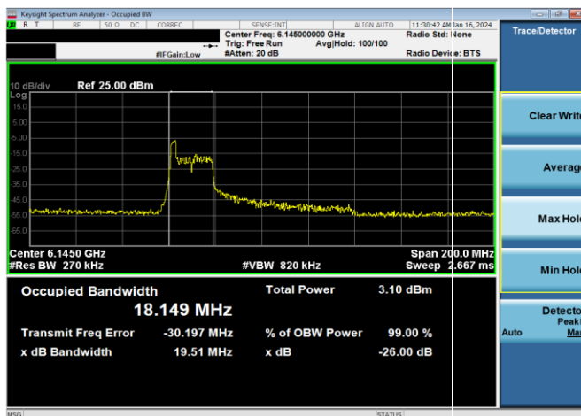
Plot 7-9. 26dB & 99% Bandwidth Plot Antenna WF5B (80MHz 802.11ax RU26 (UNII Band 5) – Ch. 39)
