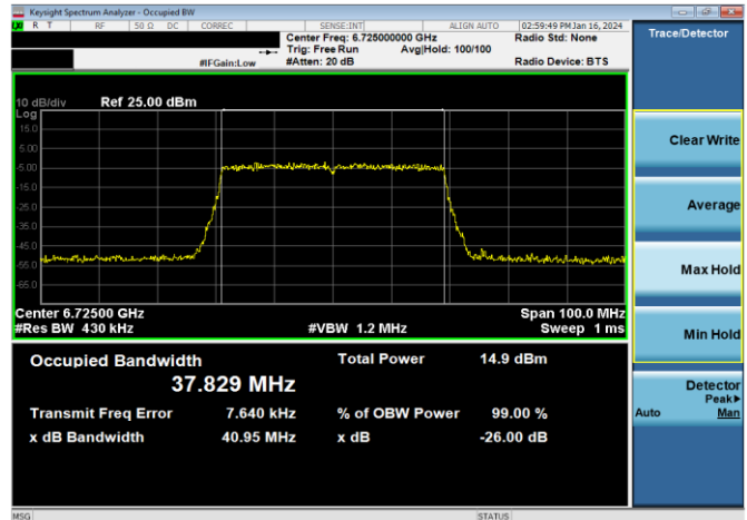
Plot 7-40. 26dB & 99% Bandwidth Plot Antenna WF5B (40MHz 802.11ax RU484 (UNII Band 7) – Ch. 155)
