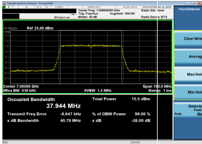
Plot 7-56. 26dB & 99% Bandwidth Plot Antenna WF5B (40MHz 802.11ax RU484 (UNII Band 8) - Ch. 211)
