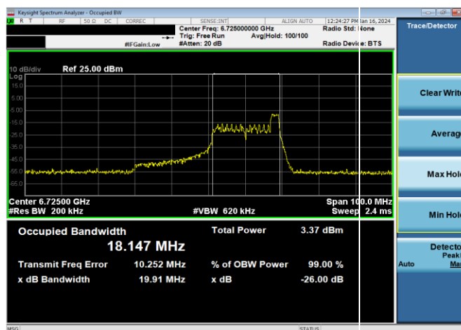
Plot 7-39. 26dB & 99% Bandwidth Plot Antenna WF5B (40MHz 802.11ax RU26 (UNII Band 7) – Ch. 155)
