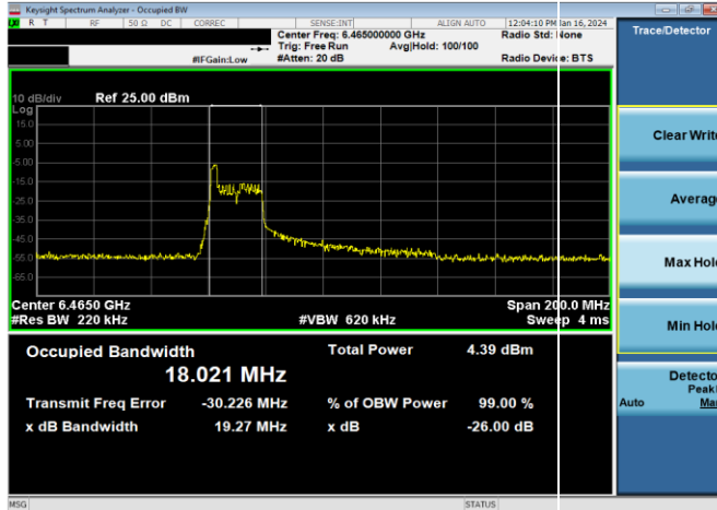
Plot 7-25. 26dB & 99% Bandwidth Plot Antenna WF5B (80MHz 802.11ax RU26 (UNII Band 6) – Ch. 103)
