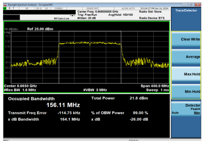
Plot 7-48. 26dB & 99% Bandwidth Plot Antenna WF5B (160MHz 802.11ax RU996x2 (UNII Band 7) – Ch. 143)
