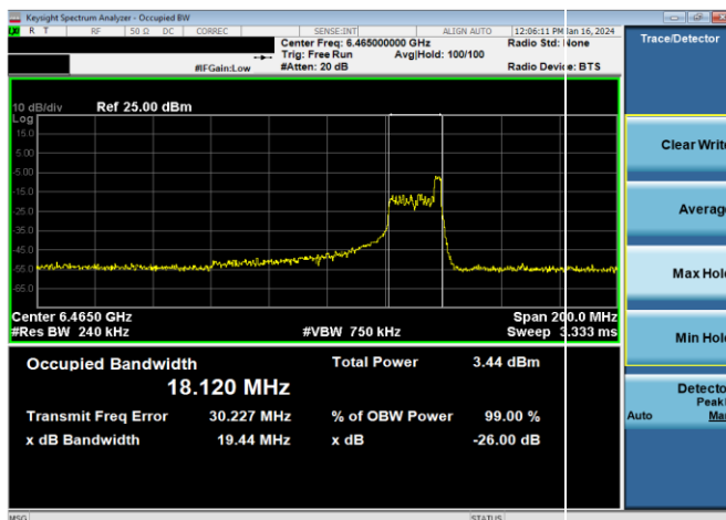
Plot 7-27. 26dB & 99% Bandwidth Plot Antenna WF5B (80MHz 802.11ax RU26 (UNII Band 6) – Ch. 103)
