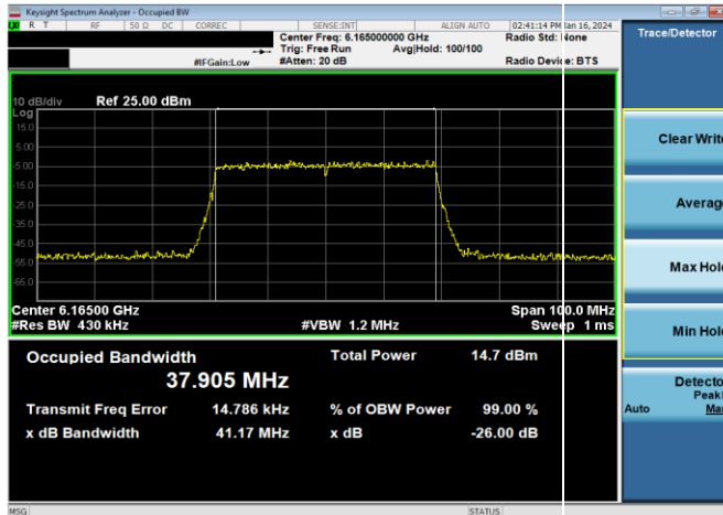
Plot 7-8. 26dB & 99% Bandwidth Plot Antenna WF5B (40MHz 802.11ax RU484 (UNII Band 5) – Ch. 43)
