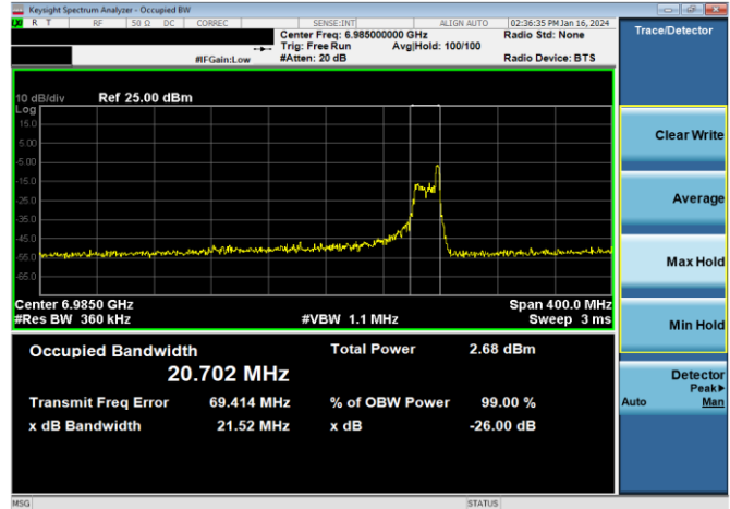
Plot 7-63. 26dB & 99% Bandwidth Plot Antenna WF5B (160MHz 802.11ax RU26 (UNII Band 8) – Ch. 207)
