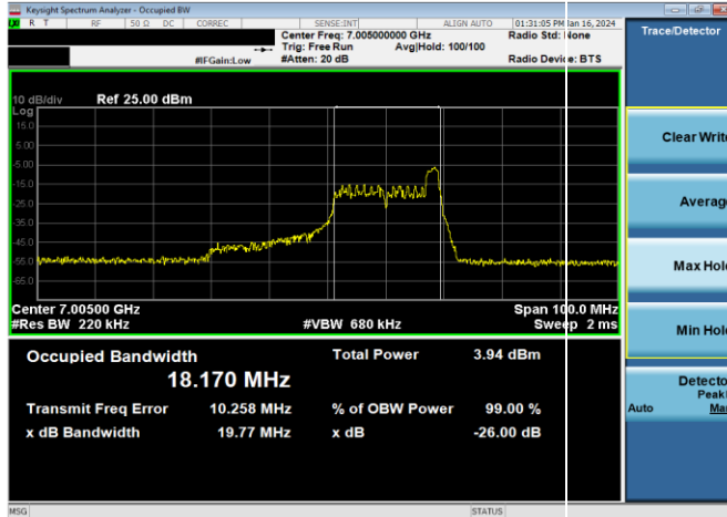
Plot 7-55. 26dB & 99% Bandwidth Plot Antenna WF5B (40MHz 802.11ax RU26 (UNII Band 8) - Ch. 211)
