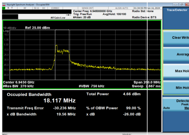
Plot 7-57. 26dB & 99% Bandwidth Plot Antenna WF5B (80MHz 802.11ax RU26 (UNII Band 8) - Ch. 199)
