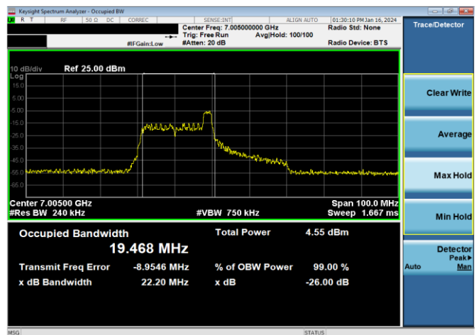
Plot 7-54. 26dB & 99% Bandwidth Plot Antenna WF5B (40MHz 802.11ax RU26 (UNII Band 8) - Ch. 211)
