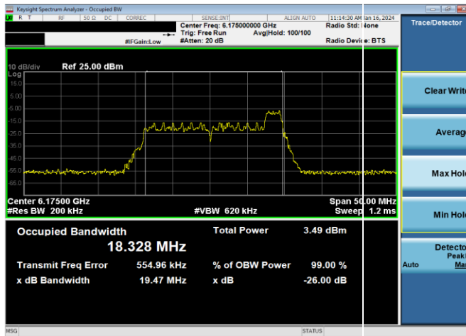
Plot 7-3. 26dB & 99% Bandwidth Plot Antenna WF5B (20MHz 802.11ax RU26 (UNII Band 5) – Ch. 45)
