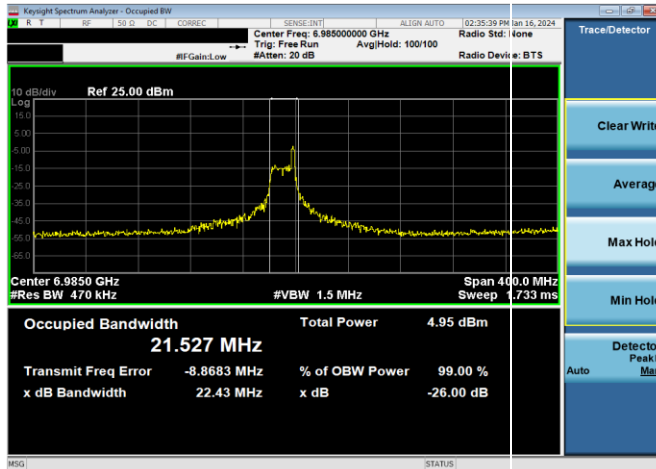
Plot 7-62. 26dB & 99% Bandwidth Plot Antenna WF5B (160MHz 802.11ax RU26 (UNII Band 8) – Ch. 207)
