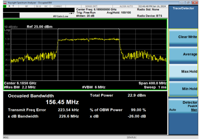
Plot 7-16. 26dB & 99% Bandwidth Plot Antenna WF5B (160MHz 802.11ax RU996x2 (UNII Band 5) – Ch. 47)
