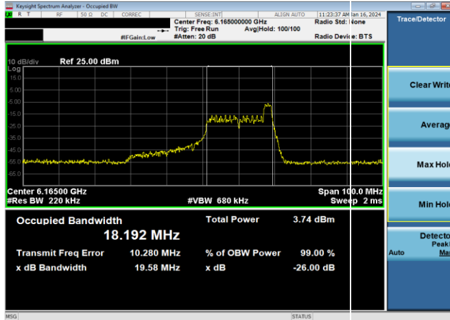
Plot 7-7. 26dB & 99% Bandwidth Plot Antenna WF5B (40MHz 802.11ax RU26 (UNII Band 5) – Ch. 43)
