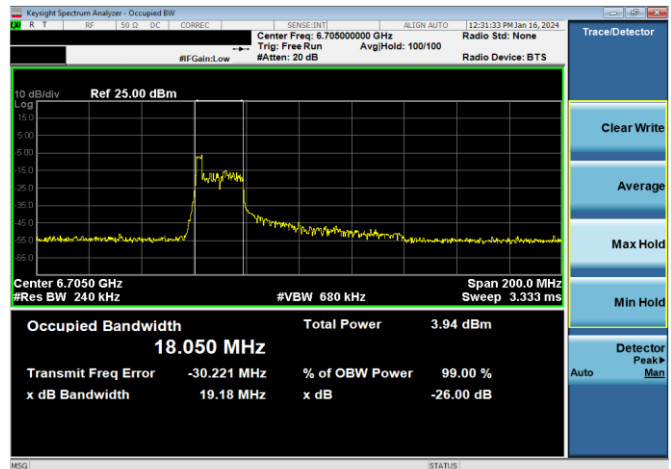
Plot 7-41. 26dB & 99% Bandwidth Plot Antenna WF5B (80MHz 802.11ax RU26 (UNII Band 7) – Ch. 151)
