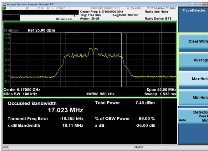
Plot 7-66. 26dB & 99% Bandwidth Plot Antenna WF8 (20MHz 802.11ax RU26 (UNII Band 5) – Ch. 45)
