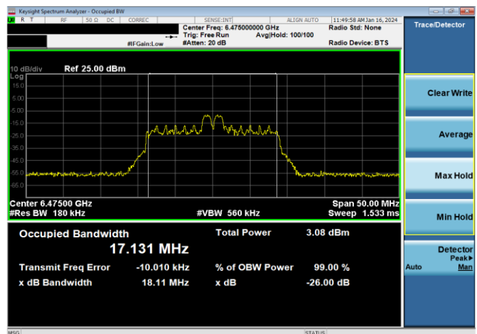
Plot 7-18. 26dB & 99% Bandwidth Plot Antenna WF5B (20MHz 802.11ax RU26 (UNII Band 6) – Ch. 105)
