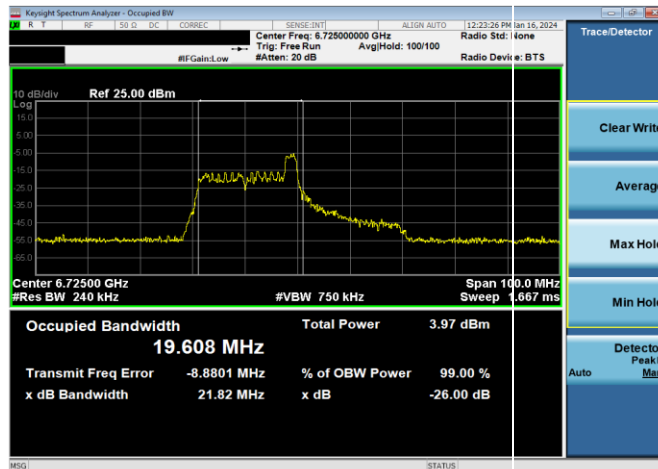
Plot 7-38. 26dB & 99% Bandwidth Plot Antenna WF5B (40MHz 802.11ax RU26 (UNII Band 7) – Ch. 155)
