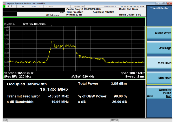
Plot 7-5. 26dB & 99% Bandwidth Plot Antenna WF5B (40MHz 802.11ax RU26 (UNII Band 5) – Ch. 43)
