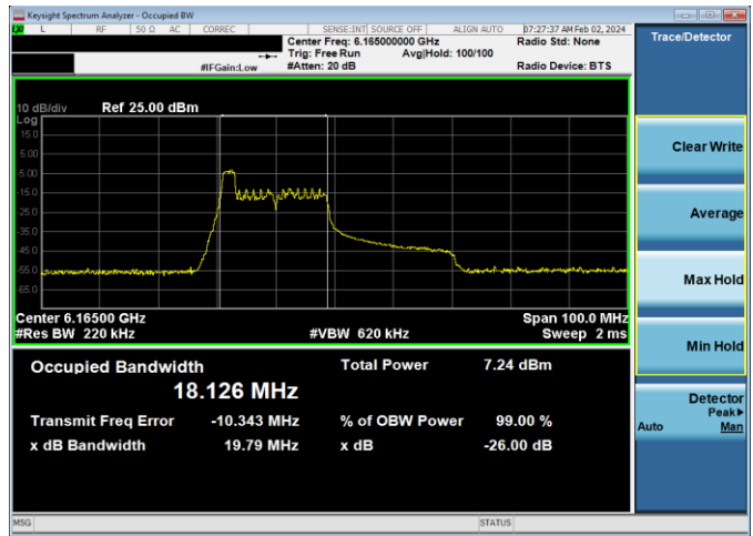
Plot 7-69. 26dB & 99% Bandwidth Plot Antenna WF8 (40MHz 802.11ax RU26 (UNII Band 5) – Ch. 43)
