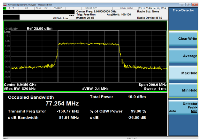
Plot 7-60. 26dB & 99% Bandwidth Plot Antenna WF5B (80MHz 802.11ax RU996 (UNII Band 8) - Ch. 199)
