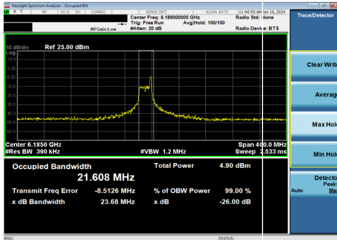
Plot 7-14. 26dB & 99% Bandwidth Plot Antenna WF5B (160MHz 802.11ax RU26 (UNII Band 5) – Ch. 47)
