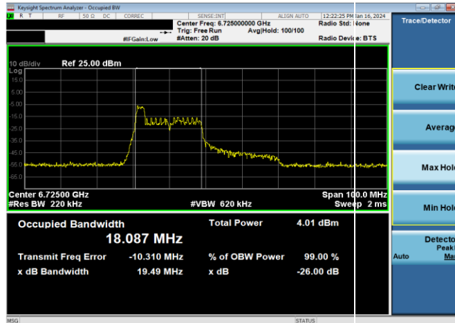
Plot 7-37. 26dB & 99% Bandwidth Plot Antenna WF5B (40MHz 802.11ax RU26 (UNII Band 7) – Ch. 155)
