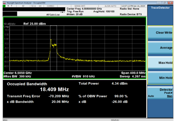
Plot 7-29. 26dB & 99% Bandwidth Plot Antenna WF5B (160MHz 802.11ax RU26 (UNII Band 6) – Ch. 111)
