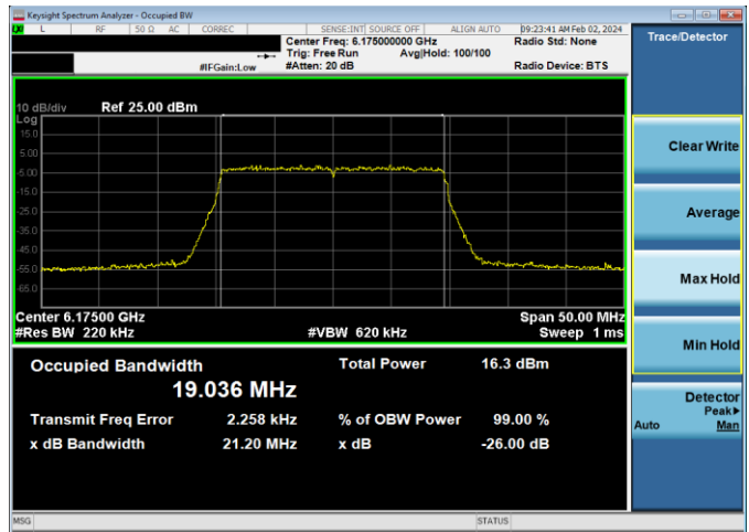
Plot 7-68. 26dB & 99% Bandwidth Plot Antenna WF8 (20MHz 802.11ax RU242 (UNII Band 5) – Ch. 45)
