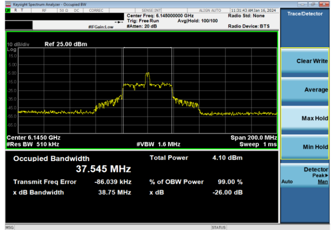
Plot 7-10. 26dB & 99% Bandwidth Plot Antenna WF5B (80MHz 802.11ax RU26 (UNII Band 5) – Ch. 39)
