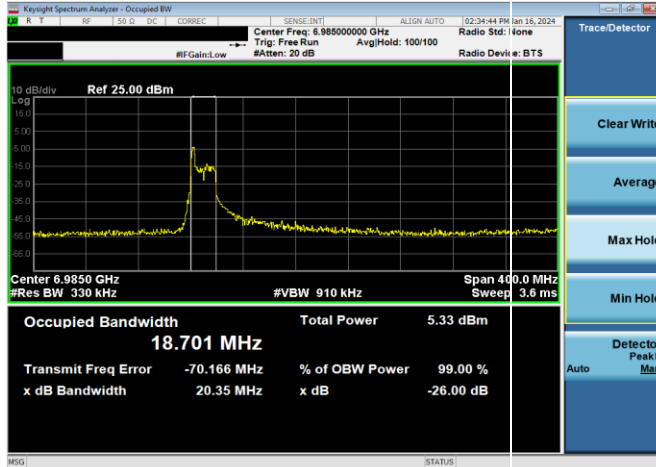
Plot 7-61. 26dB & 99% Bandwidth Plot Antenna WF5B (160MHz 802.11ax RU26 (UNII Band 8) – Ch. 207)
