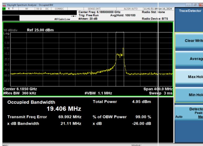
Plot 7-15. 26dB & 99% Bandwidth Plot Antenna WF5B (160MHz 802.11ax RU26 (UNII Band 5) – Ch. 47)
