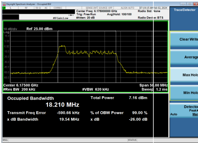
Plot 7-65. 26dB & 99% Bandwidth Plot Antenna WF8 (20MHz 802.11ax RU26 (UNII Band 5) – Ch. 45)
