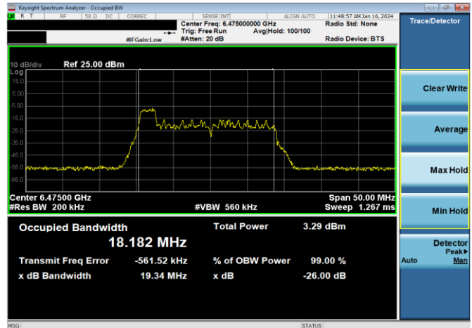
Plot 7-17. 26dB & 99% Bandwidth Plot Antenna WF5B (20MHz 802.11ax RU26 (UNII Band 6) – Ch. 105)
