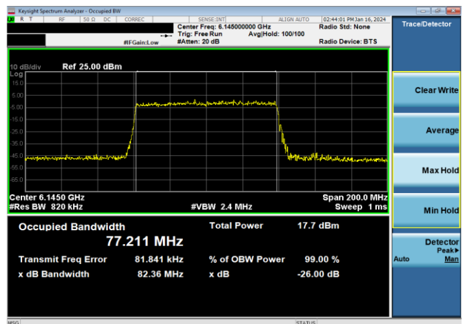
Plot 7-12. 26dB & 99% Bandwidth Plot Antenna WF5B (80MHz 802.11ax RU996 (UNII Band 5) – Ch. 39)
