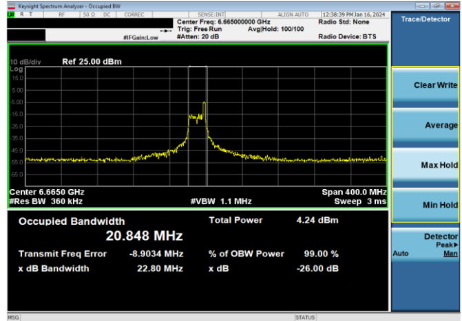
Plot 7-46. 26dB & 99% Bandwidth Plot Antenna WF5B (160MHz 802.11ax RU26 (UNII Band 7) – Ch. 143)
