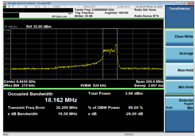
Plot 7-59. 26dB & 99% Bandwidth Plot Antenna WF5B (80MHz 802.11ax RU26 (UNII Band 8) - Ch. 199)
