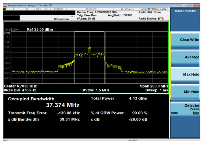
Plot 7-42. 26dB & 99% Bandwidth Plot Antenna WF5B (80MHz 802.11ax RU26 (UNII Band 7) – Ch. 151)
