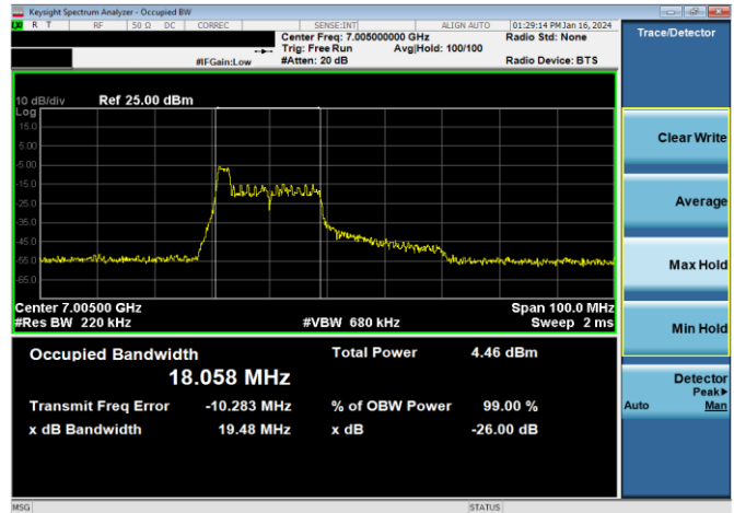
Plot 7-53. 26dB & 99% Bandwidth Plot Antenna WF5B (40MHz 802.11ax RU26 (UNII Band 8) - Ch. 211)
