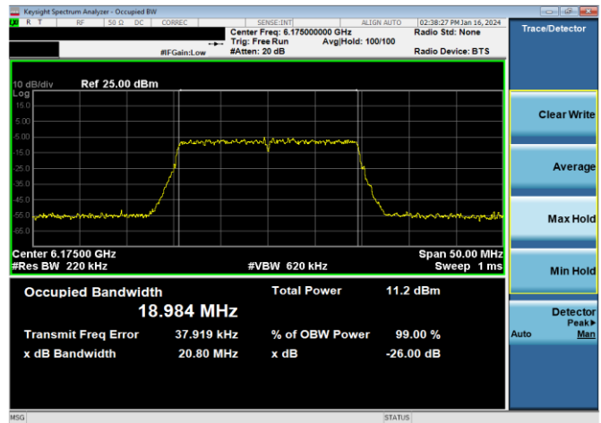
Plot 7-4. 26dB & 99% Bandwidth Plot Antenna WF5B (20MHz 802.11ax RU242 (UNII Band 5) – Ch. 45)
