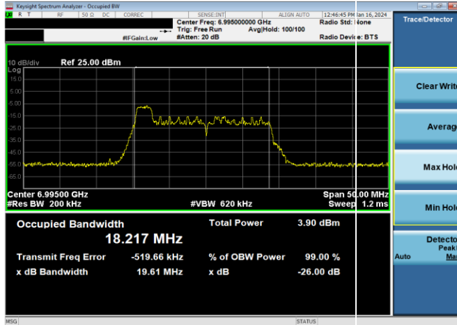
Plot 7-49. 26dB & 99% Bandwidth Plot Antenna WF5B (20MHz 802.11ax RU26 (UNII Band 8) - Ch. 209)
