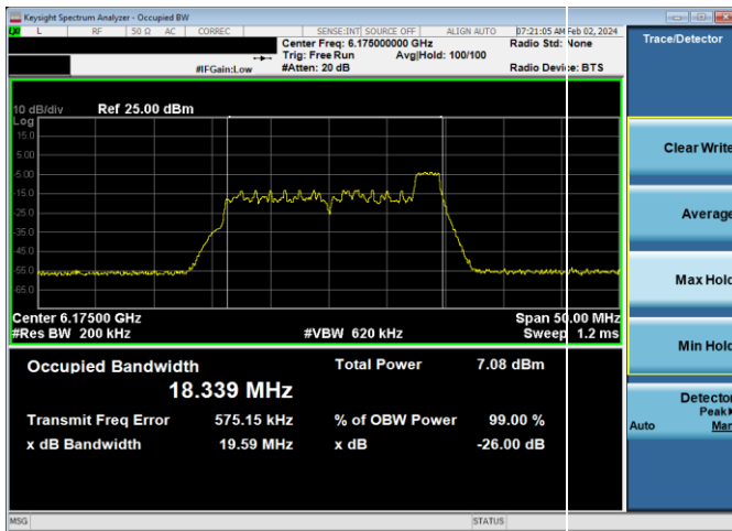
Plot 7-67. 26dB & 99% Bandwidth Plot Antenna WF8 (20MHz 802.11ax RU26 (UNII Band 5) – Ch. 45)
