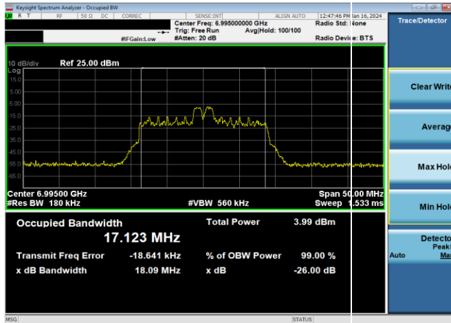
Plot 7-50. 26dB & 99% Bandwidth Plot Antenna WF5B (20MHz 802.11ax RU26 (UNII Band 8) - Ch. 209)
