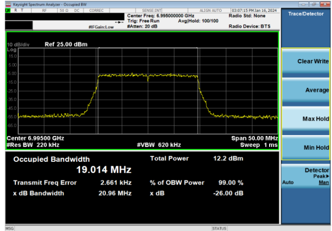
Plot 7-52. 26dB & 99% Bandwidth Plot Antenna WF5B (20MHz 802.11ax RU242 (UNII Band 8) - Ch. 209)
