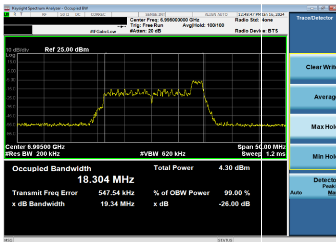
Plot 7-51. 26dB & 99% Bandwidth Plot Antenna WF5B (20MHz 802.11ax RU26 (UNII Band 8) - Ch. 209)
