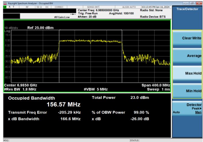
Plot 7-64. 26dB & 99% Bandwidth Plot Antenna WF5B (160MHz 802.11ax RU996x2 (UNII Band 8) – Ch. 207)
