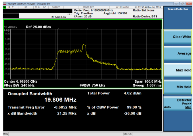
Plot 7-6. 26dB & 99% Bandwidth Plot Antenna WF5B (40MHz 802.11ax RU26 (UNII Band 5) – Ch. 43)
