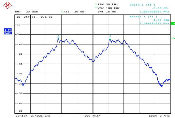
GFSK_Low 1.002 MHz
