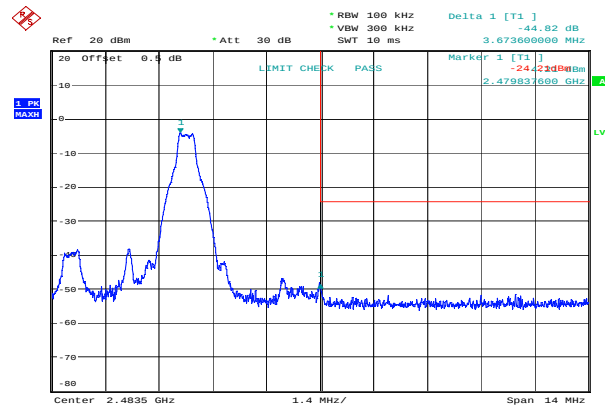
GFSK_High 44.82 dB
