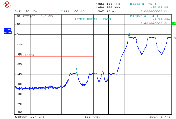
GFSK_Hopping_Lower 35.53 dB
