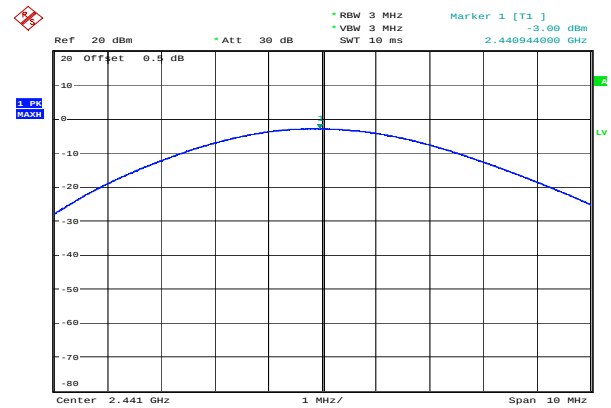
GFSK_Middle -3.00 dBm
