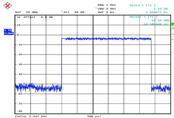
8DPSK_Hopping_3DH5 2.910ms
