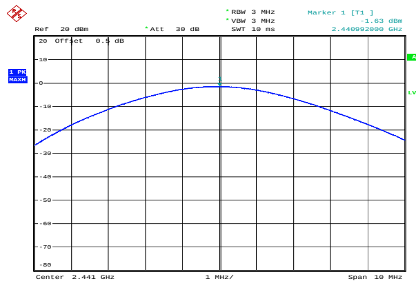
8DPSK_Middle -1.63 dBm
