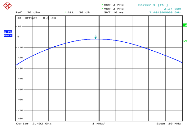
GFSK_Low -2.24 dBm
