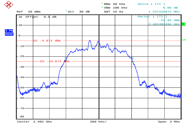
8DPSK_Low 1.237 MHz
