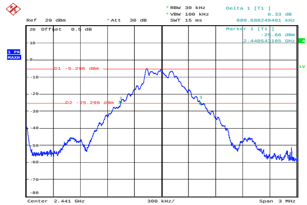
GFSK_Middle 0.890 MHz
