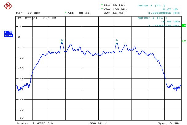
8DPSK_High 1.002 MHz
