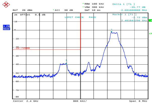
GFSK_Low 35.77 dB
