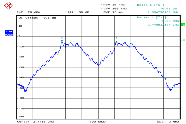
GFSK_Middle 1.005 MHz
