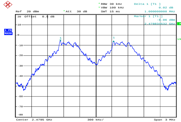
GFSK_High 1.000 MHz
