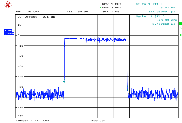
8DPSK_Hopping_3DH1 0.392ms
