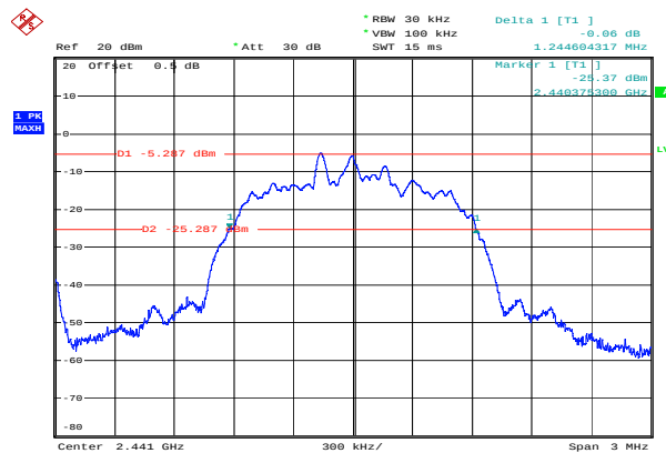
8DPSK_Middle 1.245 MHz
