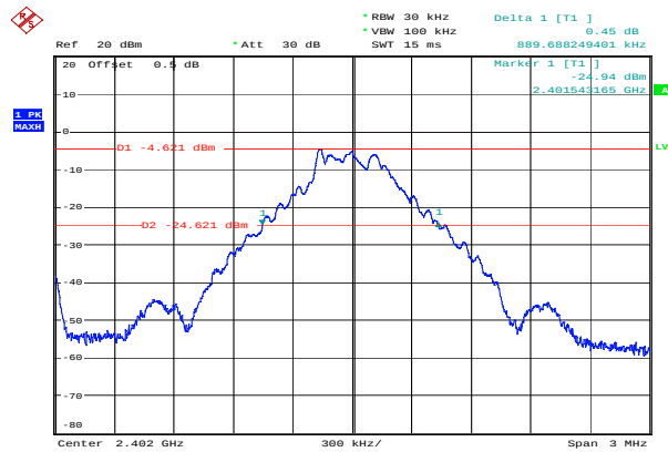
GFSK_Low 0.890 MHz
