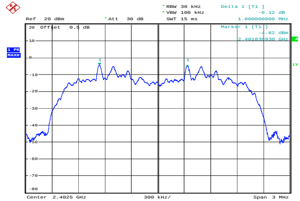
8DPSK_Low 1.000 MHz
