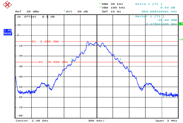
GFSK_High 0.890 MHz
