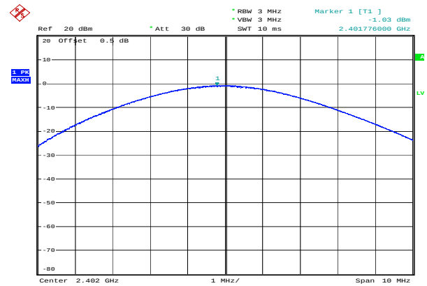
8DPSK_Low -1.03 dBm
