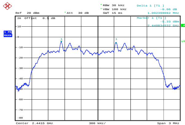
8DPSK_Middle 1.002 MHz
