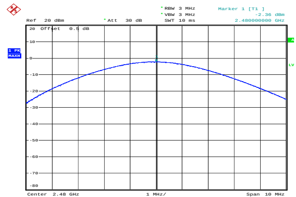
8DPSK_High -2.36 dBm
