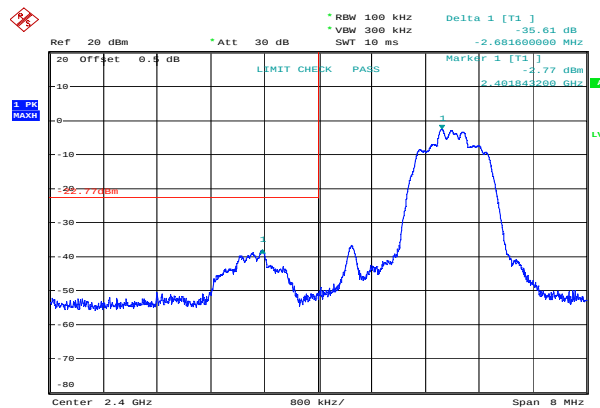
8DPSK_Low 35.61 dB
