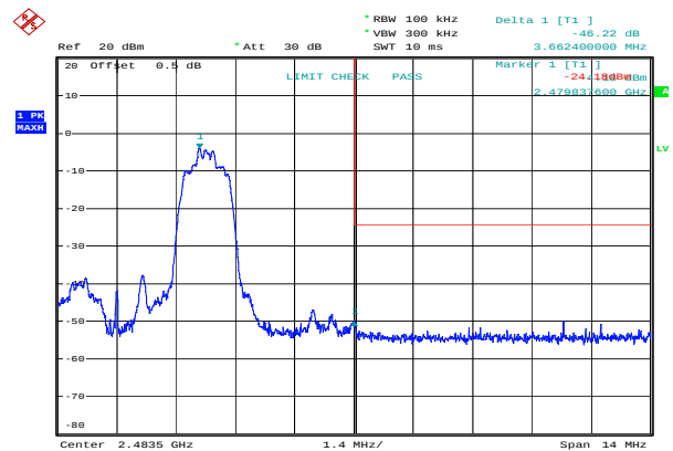
8DPSK_High 46.22 dB
