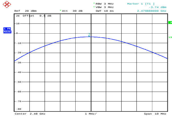
GFSK_High -3.74 dBm
