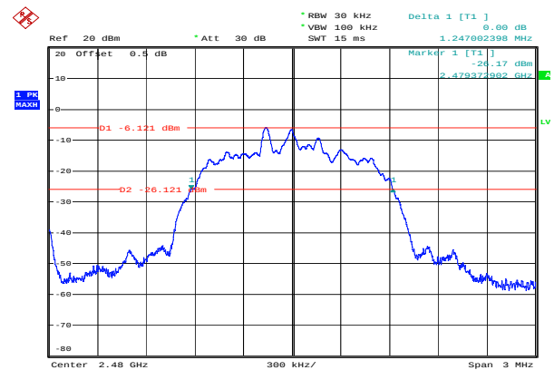
8DPSK_High 1.247 MHz
