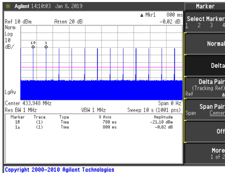
Periodic operation for the radiated emission measurements
