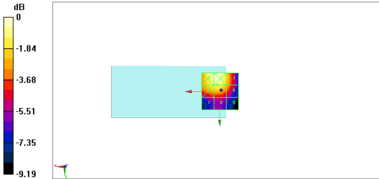
Fig B.4 HAC RF E-Field LTE Band41 PC3 64QAM CH41055
