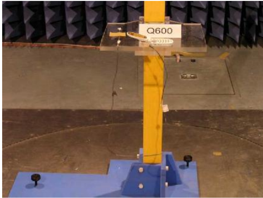
Photo 1: Radiated Spurious set-up photo
