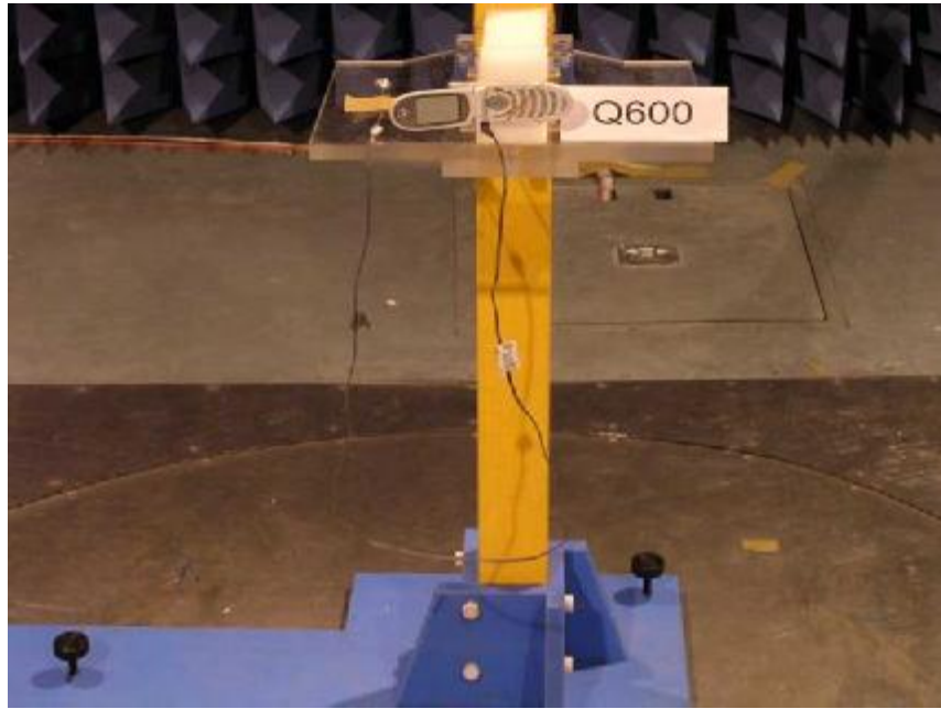
Photo 2: Radiated Spurious set-up photo
