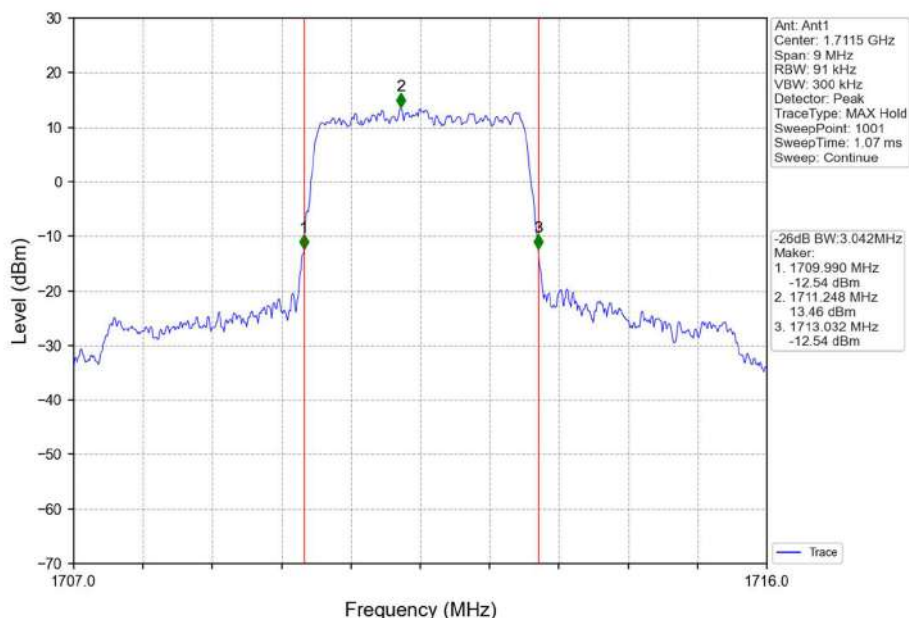
Band66_3MHz_QPSK_LCH_1711.5MHz_RB_15_0_NTNV
