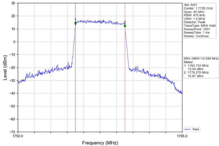
Band66_15MHz_16QAM_HCH_1772.5MHz_RB_75_0_NTNV
