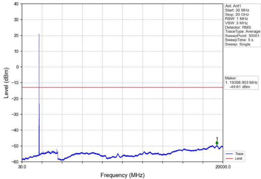
Band66_10MHz_16QAM_MCH_1745MHz_RB_1_0_NTNV
