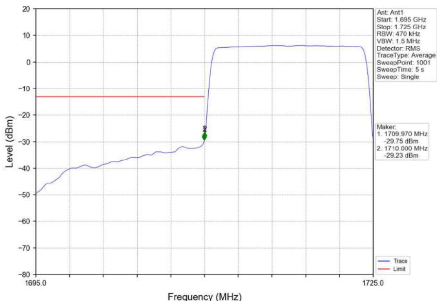
Band66_15MHz_16QAM_LCH_1717.5MHz_RB_75_0_NTNV
