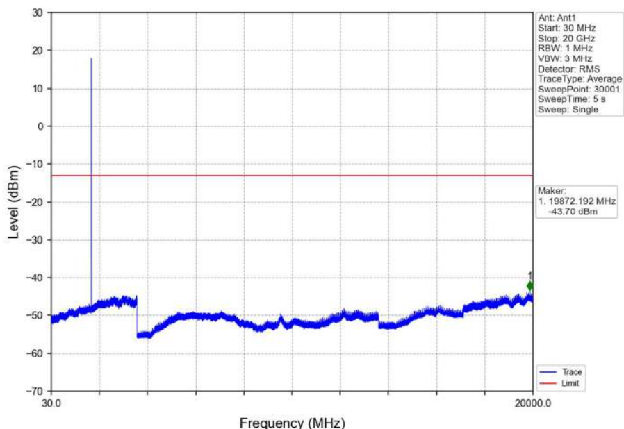
Band66_1.4MHz_QPSK_LCH_1710.7MHz_RB_1_0_NTNV
