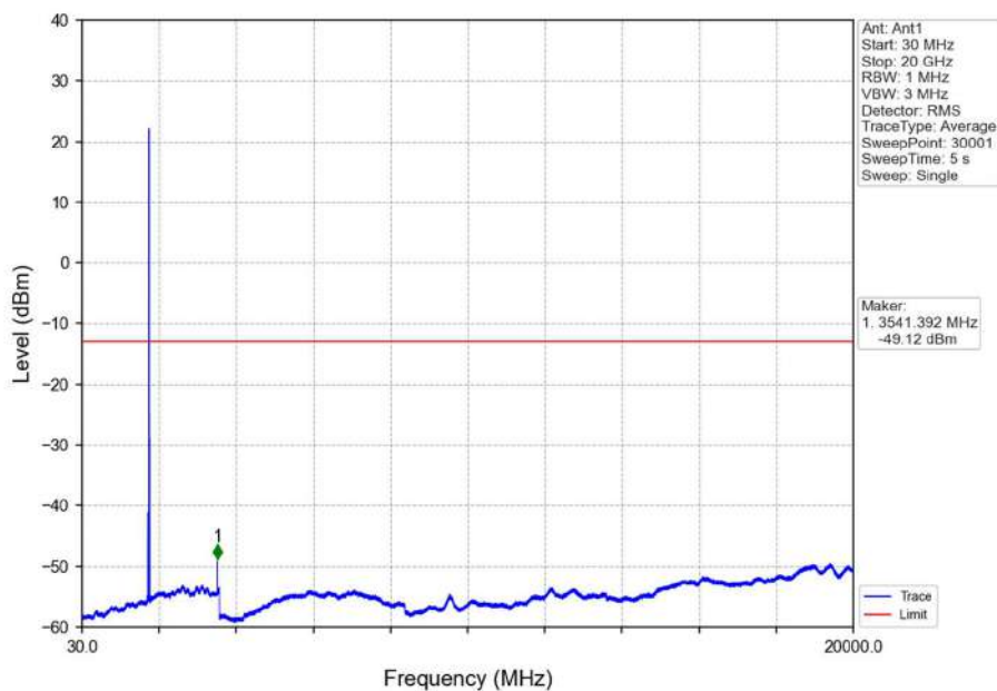
Band66_10MHz_QPSK_HCH_1775MHz_RB_1_0_NTNV
