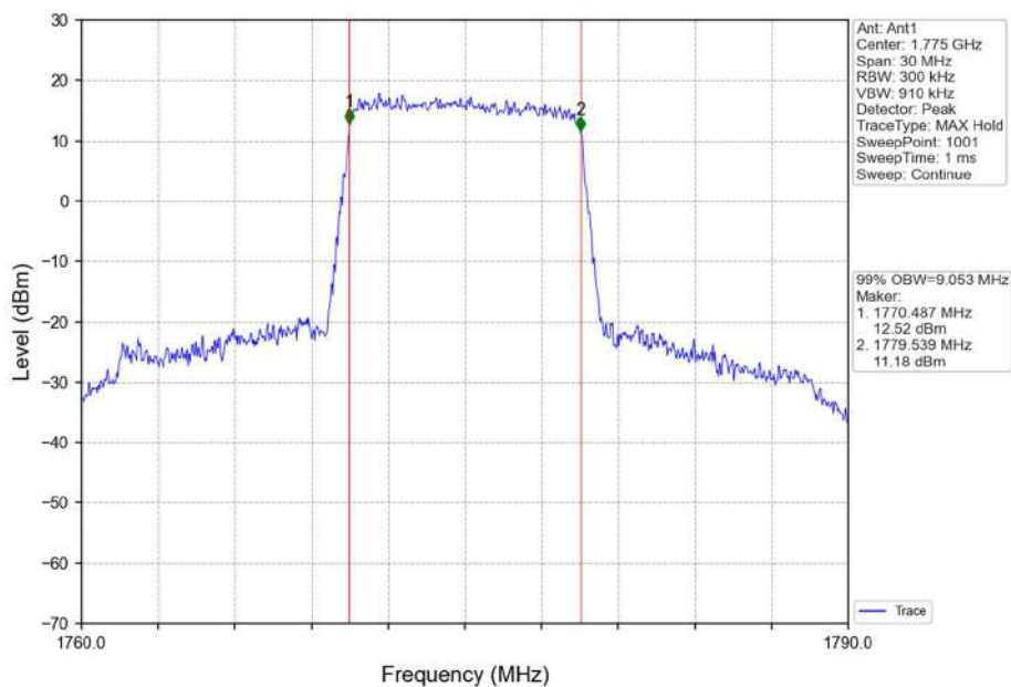
Band66_10MHz_QPSK_HCH_1775MHz_RB_50_0_NTNV
