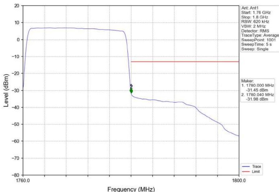
Band66_20MHz_16QAM_HCH_1770MHz_RB_100_0_NTNV
