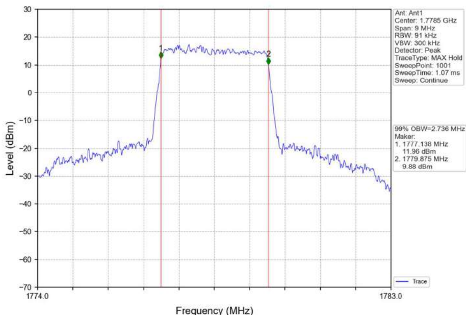
Band66_3MHz_16QAM_HCH_1778.5MHz_RB_15_0_NTNV
