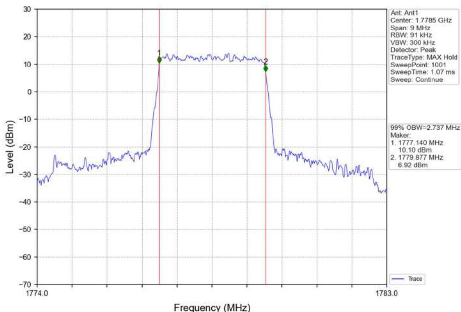
Band66_3MHz_QPSK_HCH_1778.5MHz_RB_15_0_NTNV
