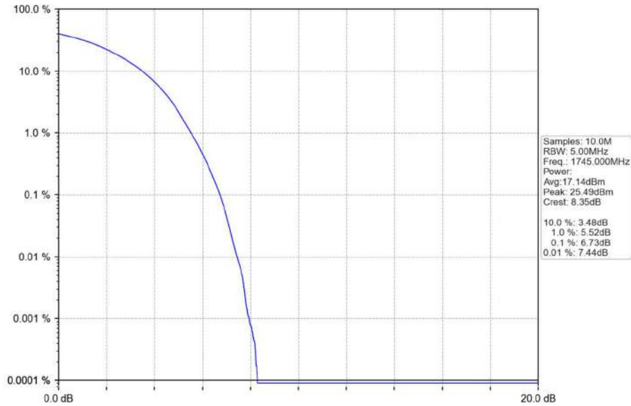
Band66_15MHz_QPSK_MCH_1745MHz_RB_75_0_NTNV
