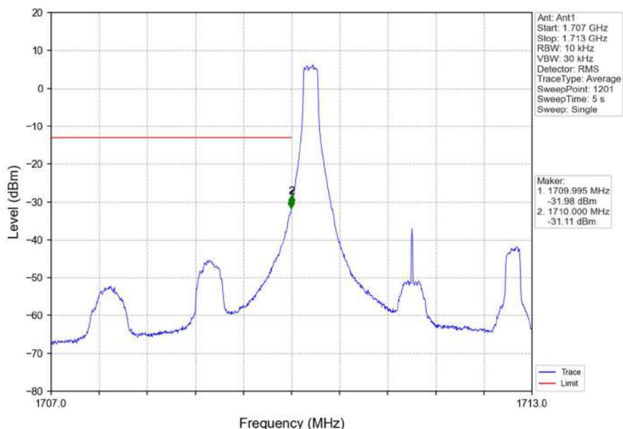
Band66_3MHz_16QAM_LCH_1711.5MHz_RB_1_0_NTNV
