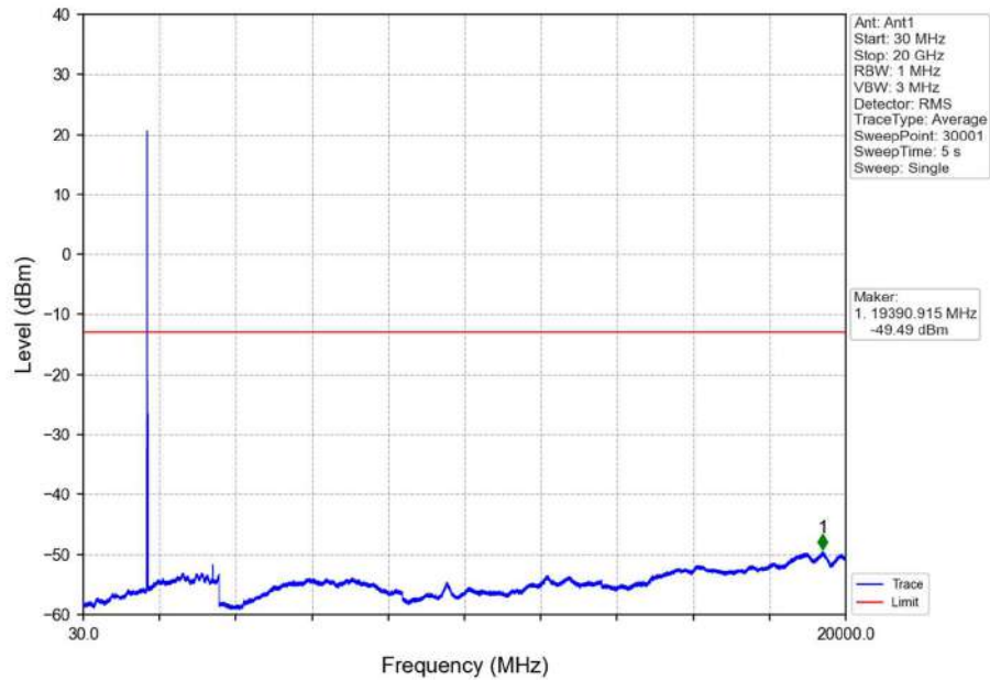
Band66_10MHz_16QAM_LCH_1715MHz_RB_1_0_NTNV
