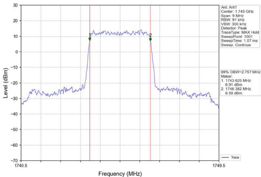
Band66_3MHz_QPSK_MCH_1745MHz_RB_15_0_NTNV
