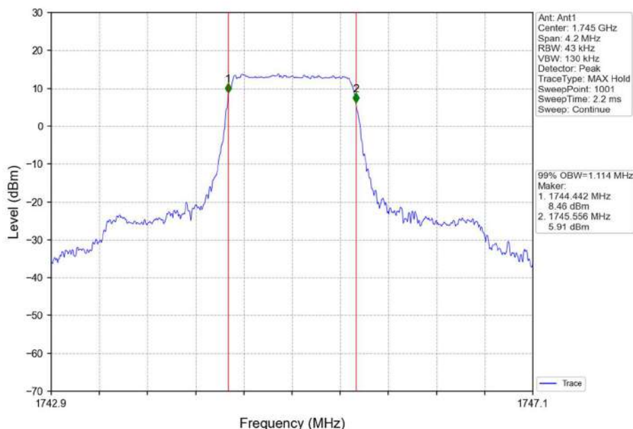
Band66_1.4MHz_QPSK_MCH_1745MHz_RB_6_0_NTNV
