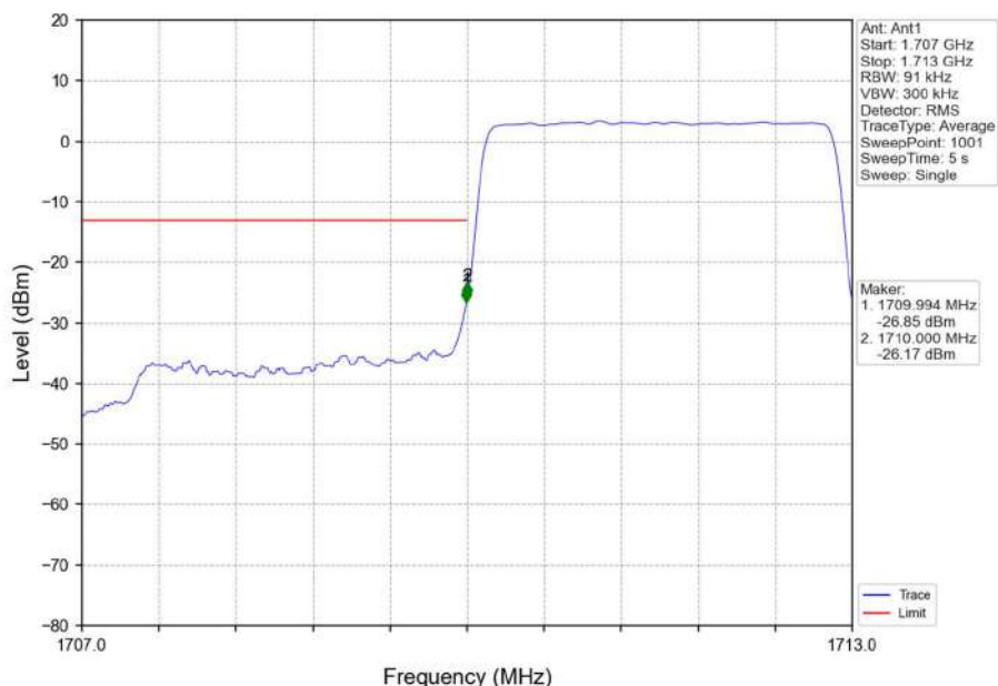
Band66_3MHz_QPSK_LCH_1711.5MHz_RB_15_0_NTNV
