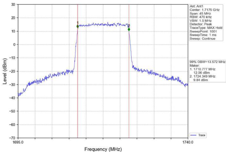
Band66_15MHz_16QAM_LCH_1717.5MHz_RB_75_0_NTNV
