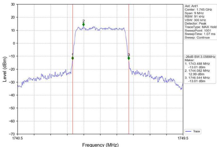
Band66_3MHz_16QAM_MCH_1745MHz_RB_15_0_NTNV
