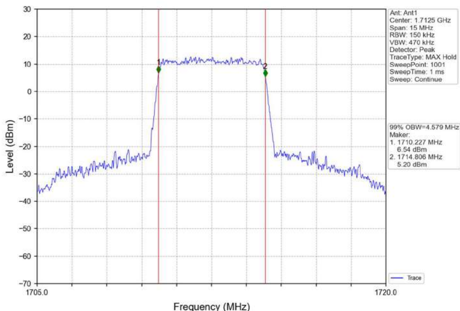
Band66_5MHz_16QAM_LCH_1712.5MHz_RB_25_0_NTNV
