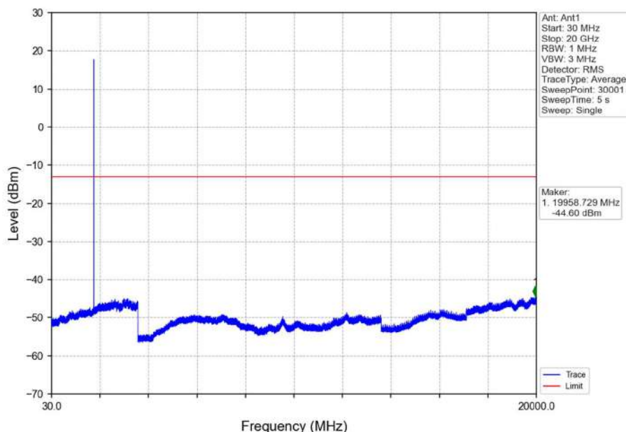
Band66_1.4MHz_16QAM_HCH_1779.3MHz_RB_1_0_NTNV
