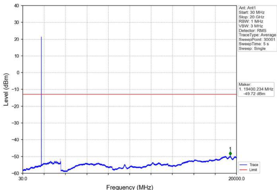
Band66_5MHz_16QAM_HCH_1777.5MHz_RB_1_0_NTNV
