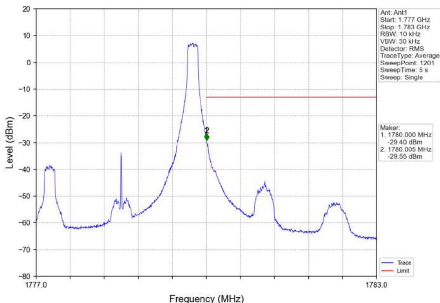
Band66_3MHz_QPSK_HCH_1778.5MHz_RB_1_14_NTNV
