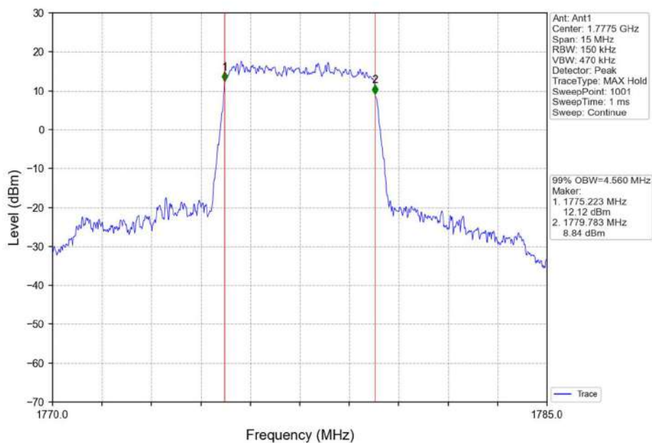
Band66_5MHz_QPSK_HCH_1777.5MHz_RB_25_0_NTNV
