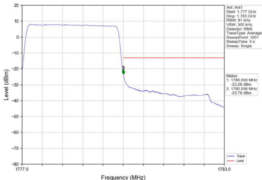
Band66_3MHz_QPSK_HCH_1778.5MHz_RB_15_0_NTNV
