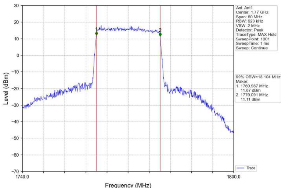
Band66_20MHz_16QAM_HCH_1770MHz_RB_100_0_NTNV
