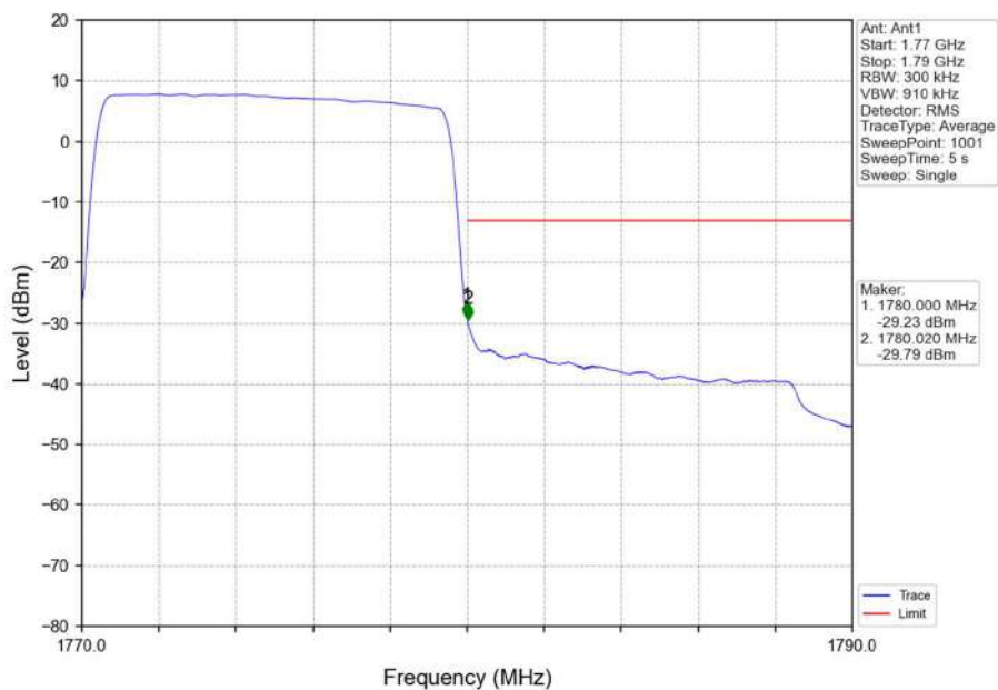
Band66_10MHz_QPSK_HCH_1775MHz_RB_50_0_NTNV
