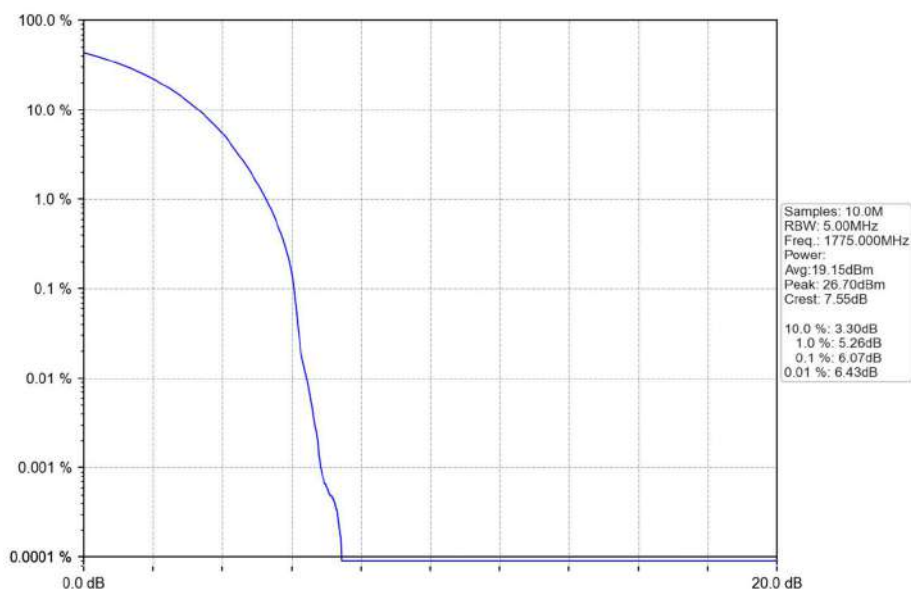
Band66_10MHz_QPSK_HCH_1775MHz_RB_50_0_NTNV
