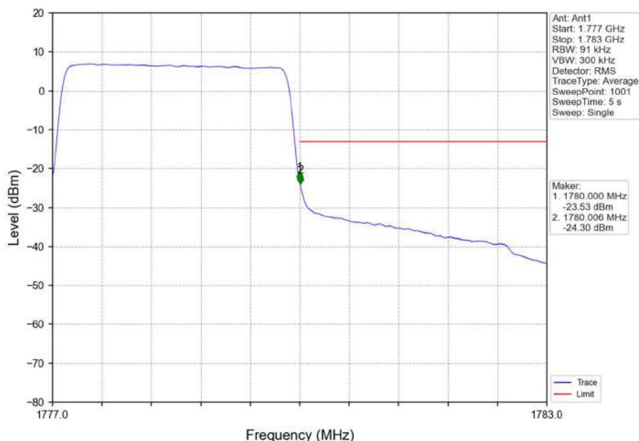
Band66_3MHz_16QAM_HCH_1778.5MHz_RB_15_0_NTNV
