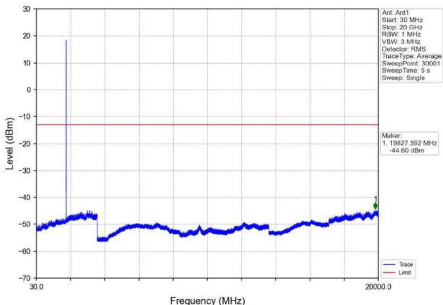
Band66_3MHz_QPSK_HCH_1778.5MHz_RB_1_0_NTNV
