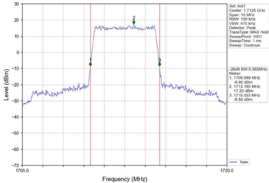
Band66_5MHz_QPSK_LCH_1712.5MHz_RB_25_0_NTNV
