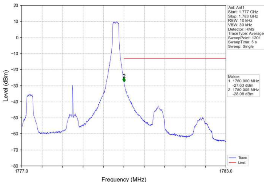
Band66_3MHz_16QAM_HCH_1778.5MHz_RB_1_14_NTNV
