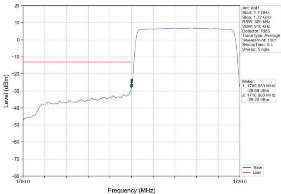
Band66_10MHz_QPSK_LCH_1715MHz_RB_50_0_NTNV
