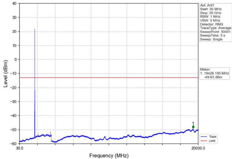
Band66_10MHz_QPSK_MCH_1745MHz_RB_1_0_NTNV
