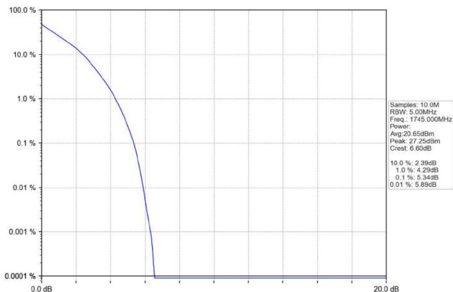
Band66_5MHz_QPSK_MCH_1745MHz_RB_25_0_NTNV
