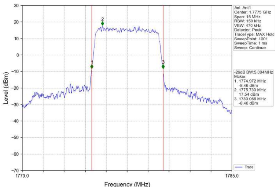
Band66_5MHz_QPSK_HCH_1777.5MHz_RB_25_0_NTNV
