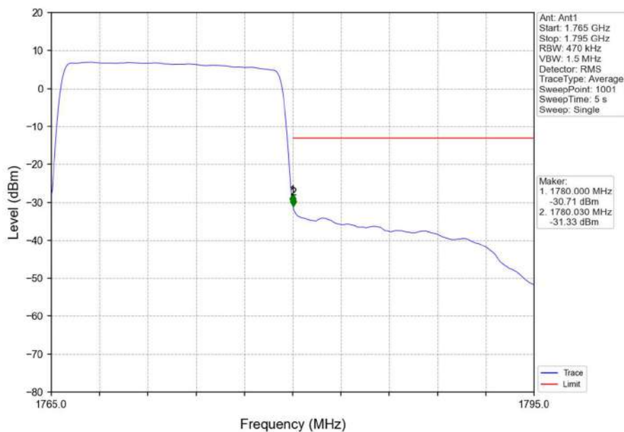
Band66_15MHz_16QAM_HCH_1772.5MHz_RB_75_0_NTNV
