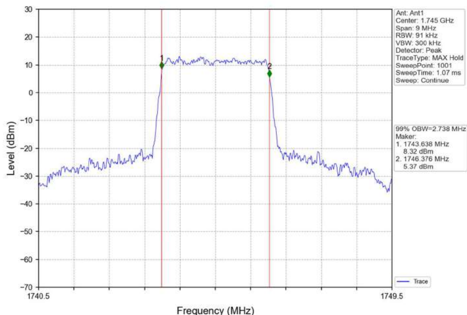
Band66_3MHz_16QAM_MCH_1745MHz_RB_15_0_NTNV
