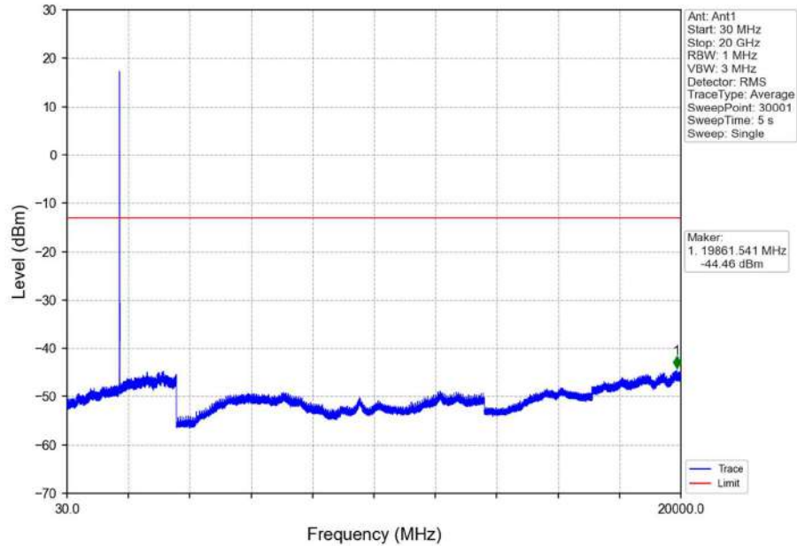
Band66_3MHz_16QAM_MCH_1745MHz_RB_1_0_NTNV
