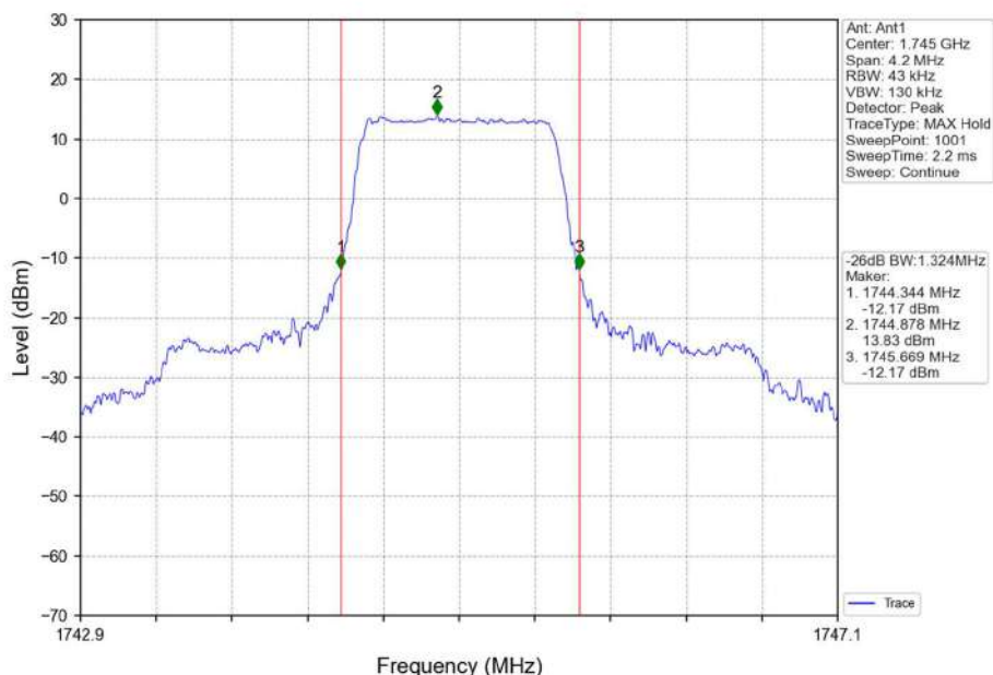
Band66_1.4MHz_QPSK_MCH_1745MHz_RB_6_0_NTNV
