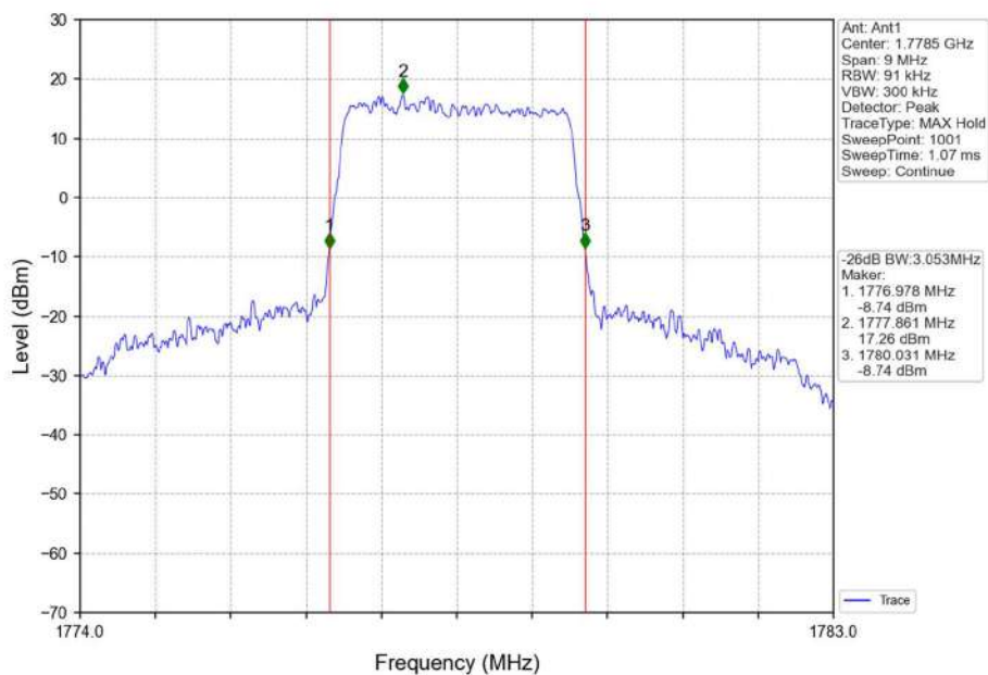
Band66_3MHz_16QAM_HCH_1778.5MHz_RB_15_0_NTNV
