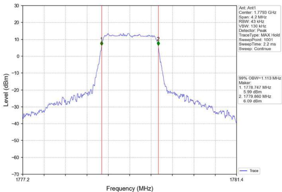
Band66_1.4MHz_16QAM_HCH_1779.3MHz_RB_6_0_NTNV
