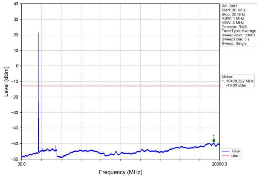
Band66_15MHz_QPSK_MCH_1745MHz_RB_1_0_NTNV
