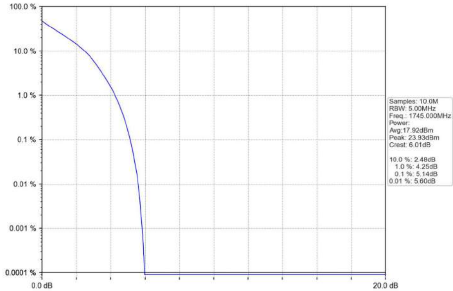
Band66_3MHz_QPSK_MCH_1745MHz_RB_15_0_NTNV
