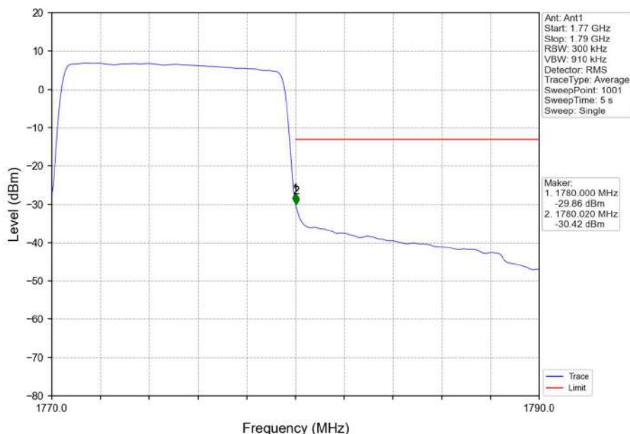
Band66_10MHz_16QAM_HCH_1775MHz_RB_50_0_NTNV
