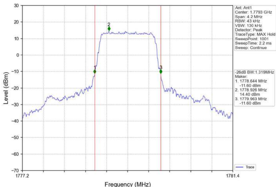
Band66_1.4MHz_QPSK_HCH_1779.3MHz_RB_6_0_NTNV
