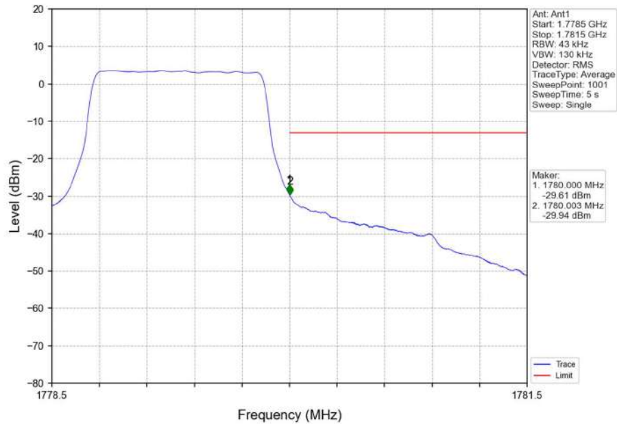
Band66_1.4MHz_16QAM_HCH_1779.3MHz_RB_6_0_NTNV
