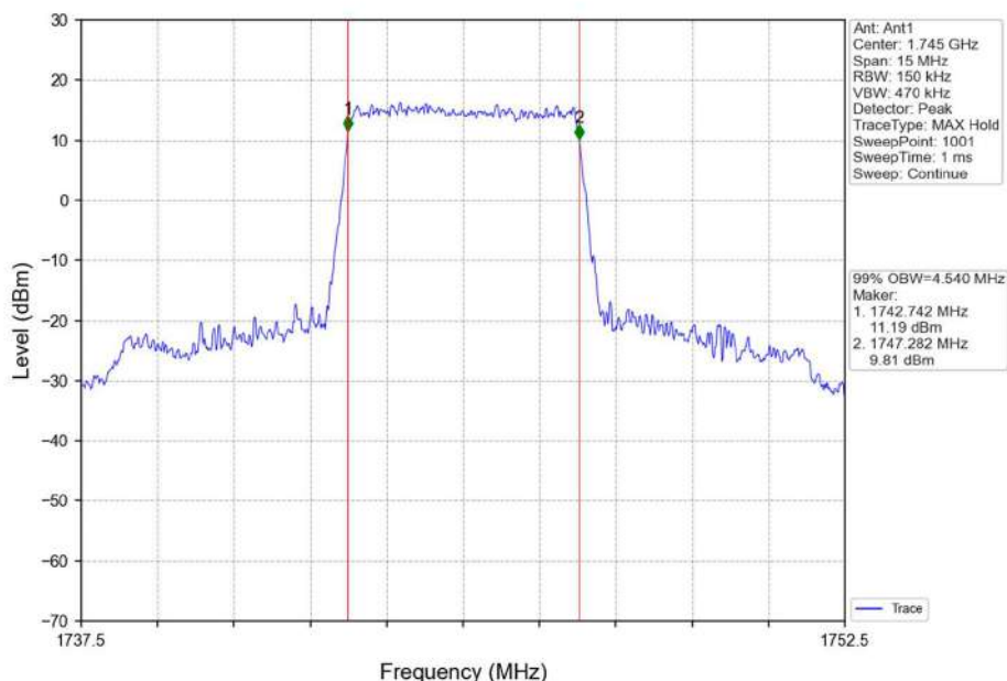
Band66_5MHz_QPSK_MCH_1745MHz_RB_25_0_NTNV
