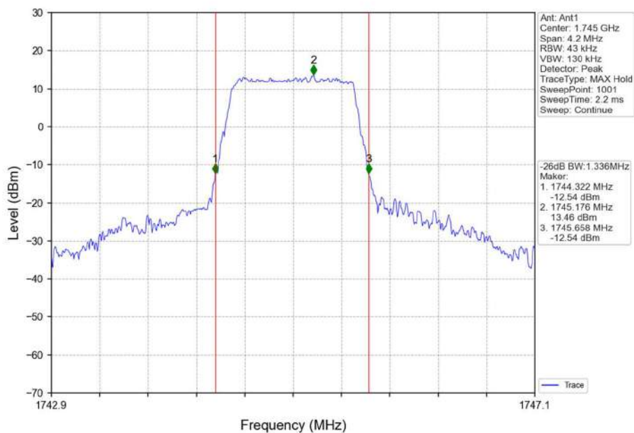
Band66_1.4MHz_16QAM_MCH_1745MHz_RB_6_0_NTNV
