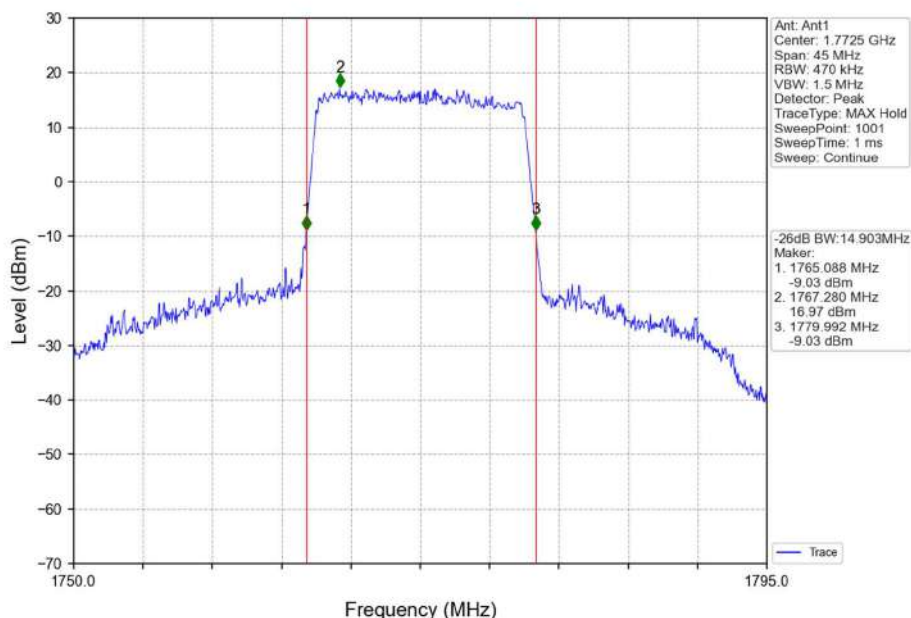
Band66_15MHz_16QAM_HCH_1772.5MHz_RB_75_0_NTNV
