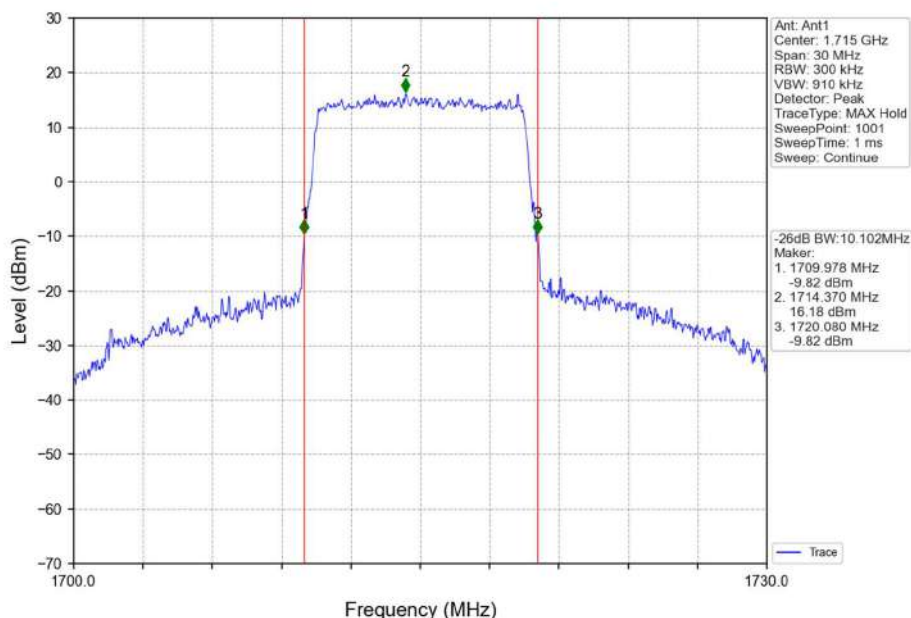
Band66_10MHz_16QAM_LCH_1715MHz_RB_50_0_NTNV
