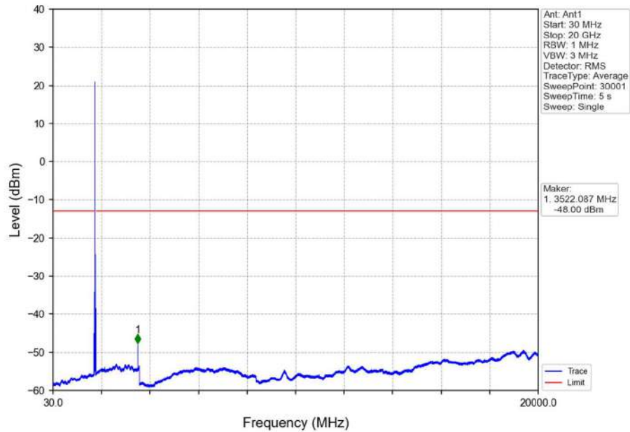
Band66_20MHz_16QAM_HCH_1770MHz_RB_1_0_NTNV
