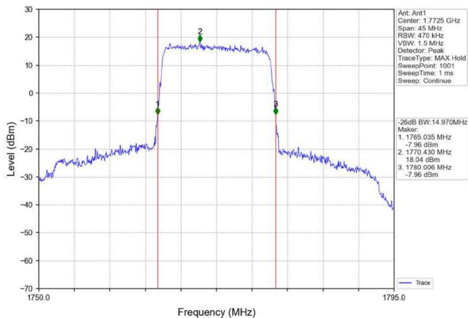
Band66_15MHz_QPSK_HCH_1772.5MHz_RB_75_0_NTNV
