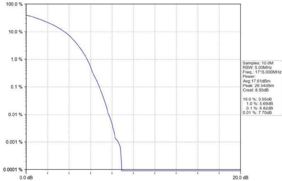
Band66_10MHz_16QAM_LCH_1715MHz_RB_50_0_NTNV
