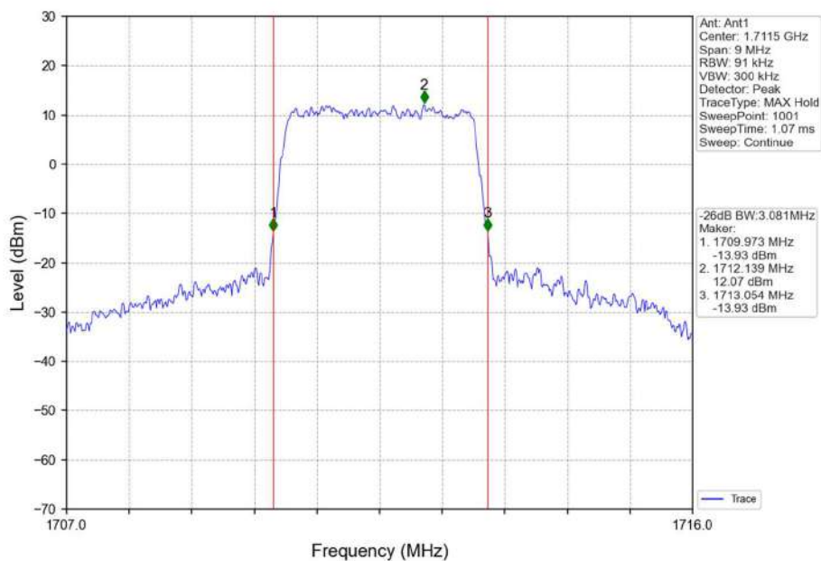
Band66_3MHz_16QAM_LCH_1711.5MHz_RB_15_0_NTNV
