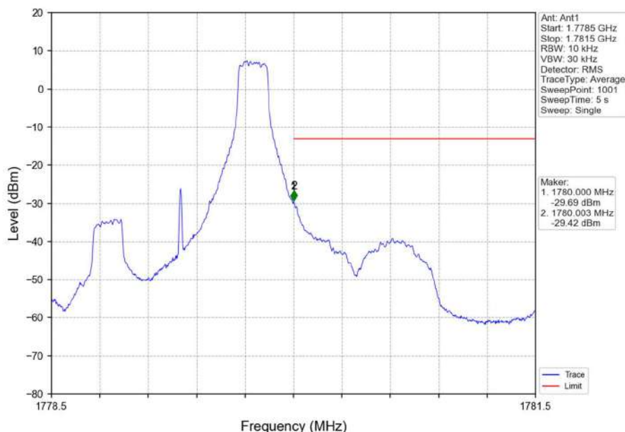
Band66_1.4MHz_QPSK_HCH_1779.3MHz_RB_1_5_NTNV
