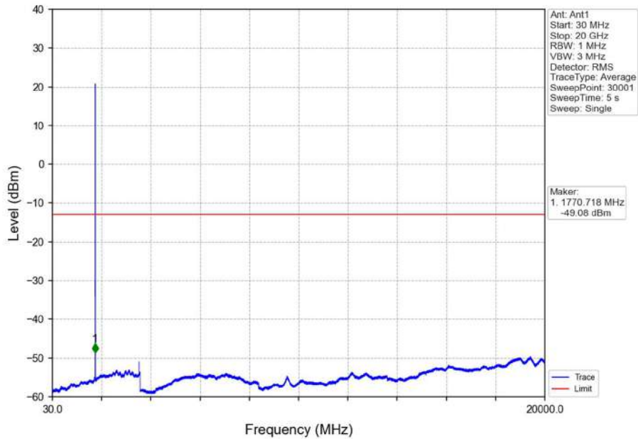
Band66_3MHz_16QAM_HCH_1778.5MHz_RB_1_0_NTNV
