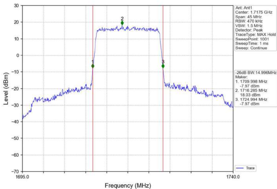
Band66_15MHz_QPSK_LCH_1717.5MHz_RB_75_0_NTNV
