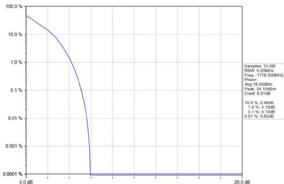
Band66_3MHz_QPSK_HCH_1778.5MHz_RB_15_0_NTNV
