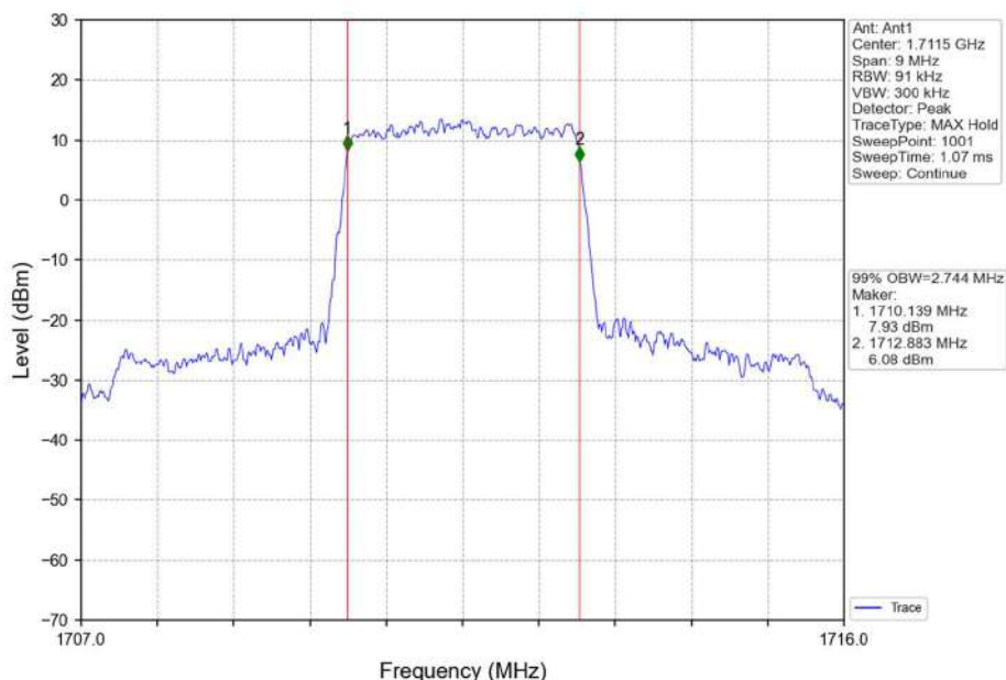
Band66_3MHz_QPSK_LCH_1711.5MHz_RB_15_0_NTNV
