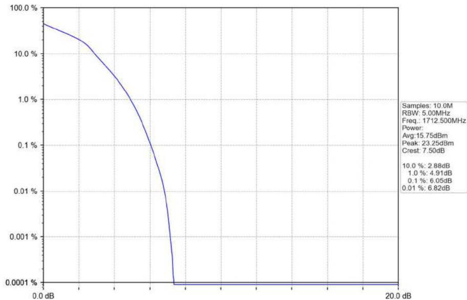
Band66_5MHz_16QAM_LCH_1712.5MHz_RB_25_0_NTNV
