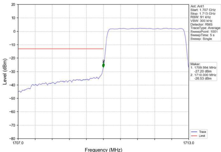
Band66_3MHz_16QAM_LCH_1711.5MHz_RB_15_0_NTNV
