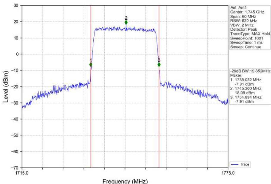
Band66_20MHz_16QAM_MCH_1745MHz_RB_100_0_NTNV
