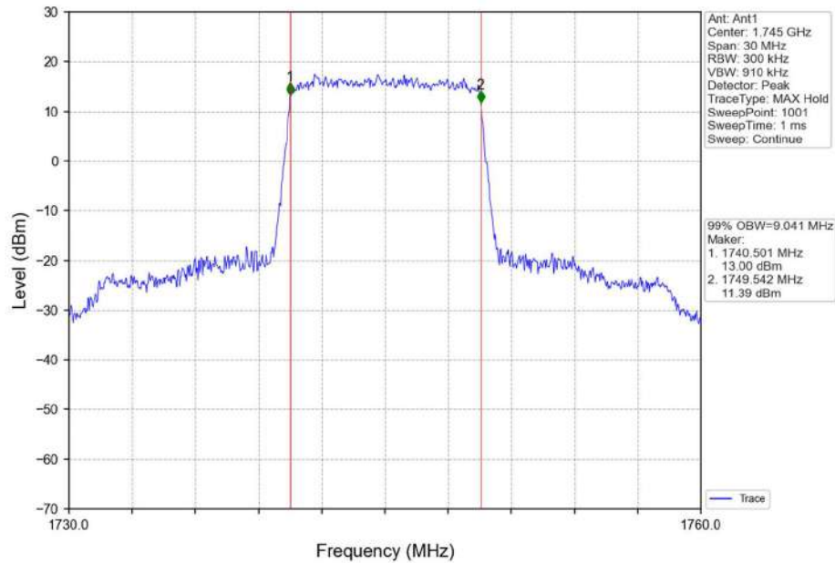
Band66_10MHz_QPSK_MCH_1745MHz_RB_50_0_NTNV
