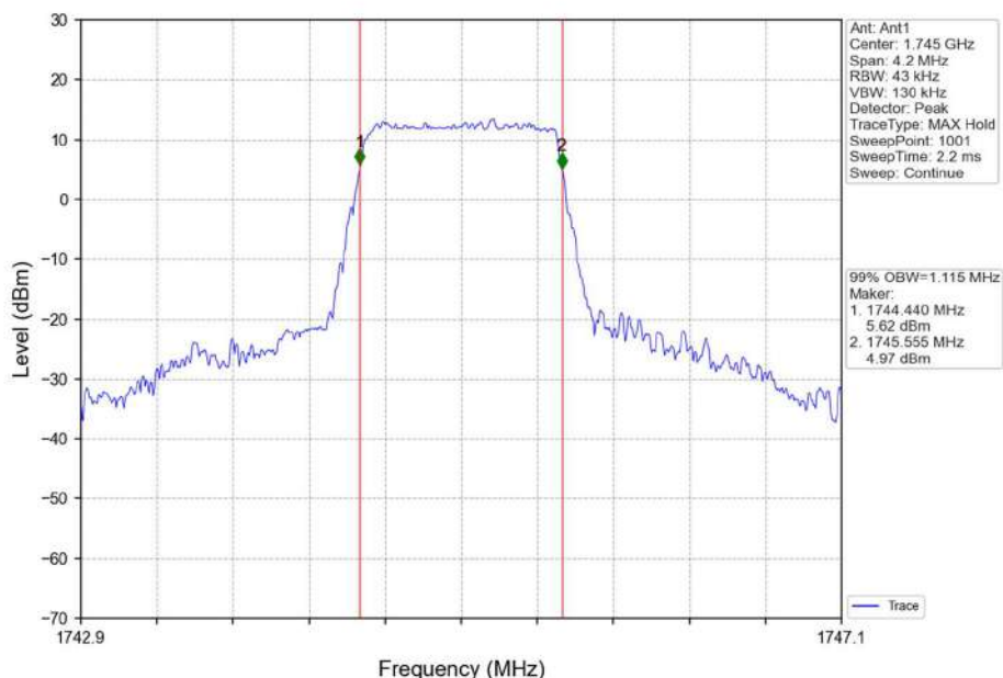
Band66_1.4MHz_16QAM_MCH_1745MHz_RB_6_0_NTNV
