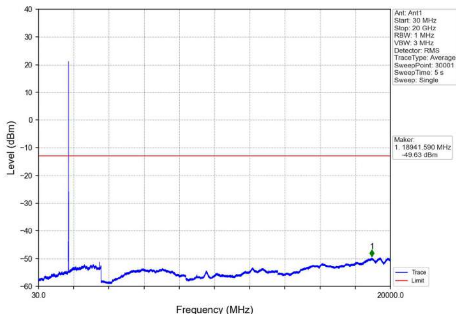
Band66_5MHz_QPSK_MCH_1745MHz_RB_1_0_NTNV
