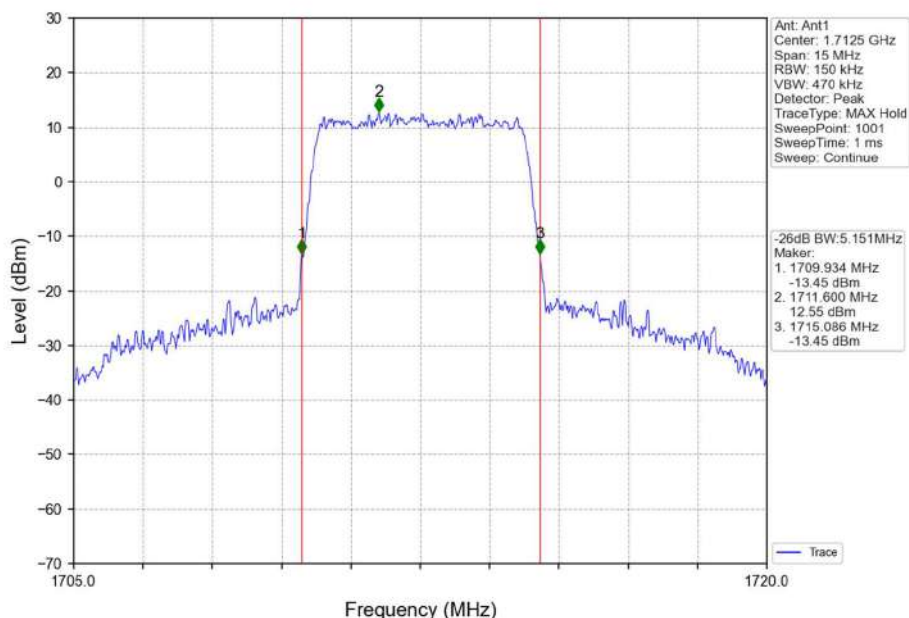
Band66_5MHz_16QAM_LCH_1712.5MHz_RB_25_0_NTNV
