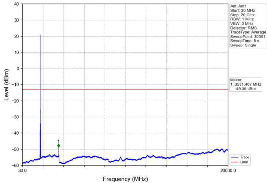
Band66_15MHz_16QAM_HCH_1772.5MHz_RB_1_0_NTNV
