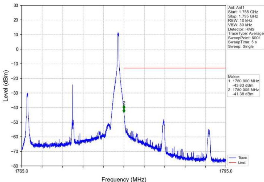
Band66_15MHz_QPSK_HCH_1772.5MHz_RB_1_74_NTNV
