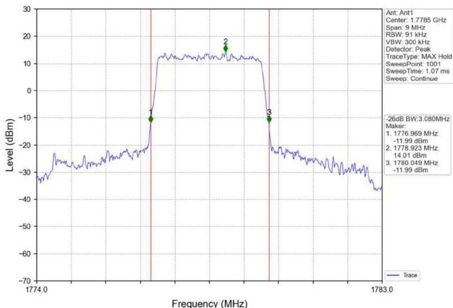
Band66_3MHz_QPSK_HCH_1778.5MHz_RB_15_0_NTNV
