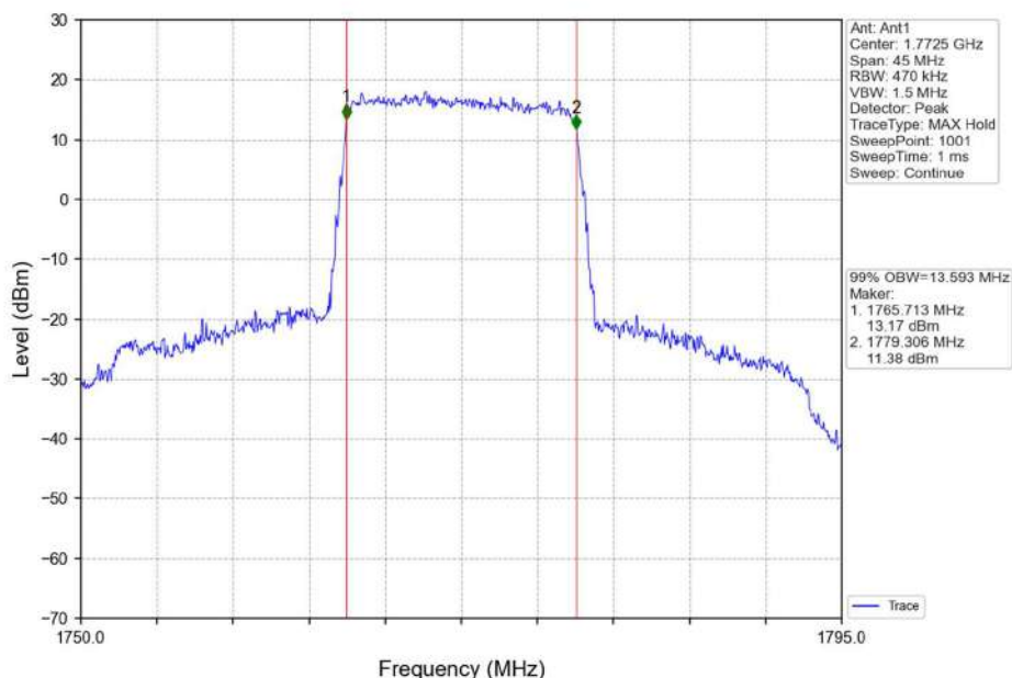
Band66_15MHz_QPSK_HCH_1772.5MHz_RB_75_0_NTNV
