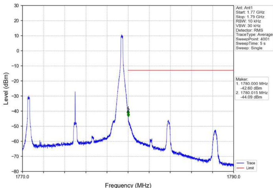
Band66_10MHz_16QAM_HCH_1775MHz_RB_1_49_NTNV
