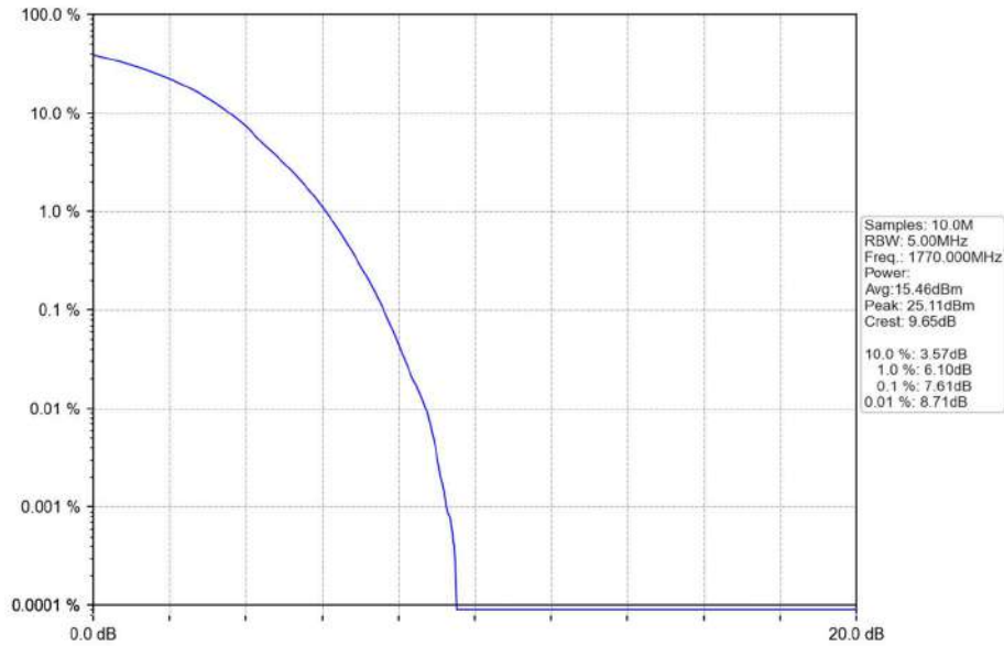
Band66_20MHz_16QAM_HCH_1770MHz_RB_100_0_NTNV
