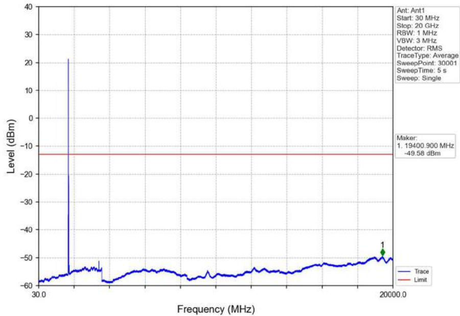
Band66_15MHz_QPSK_LCH_1717.5MHz_RB_1_0_NTNV
