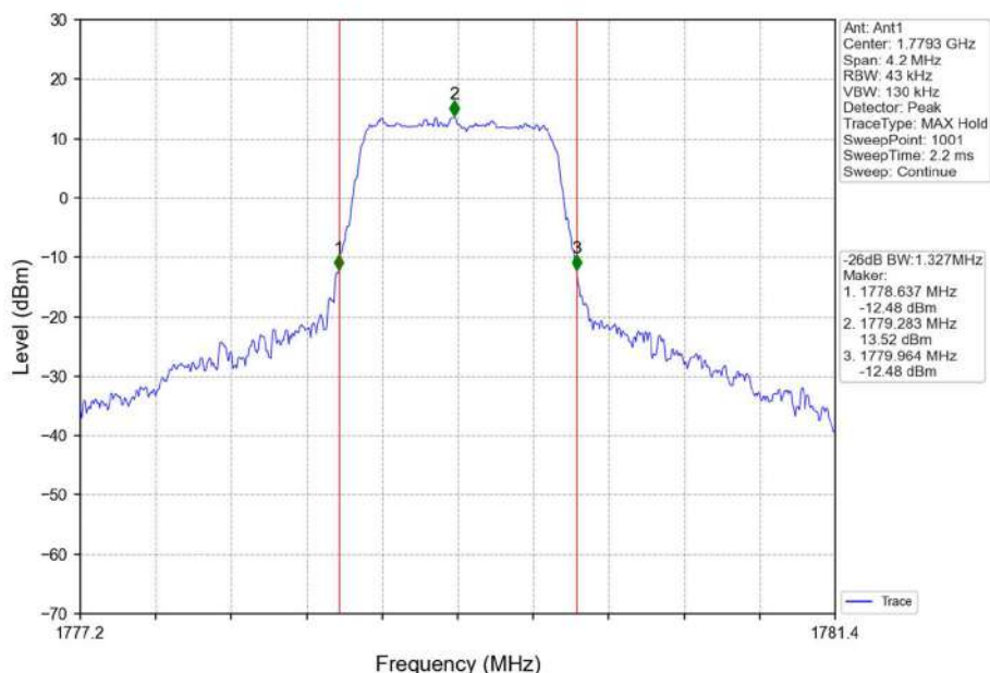
Band66_1.4MHz_16QAM_HCH_1779.3MHz_RB_6_0_NTNV
