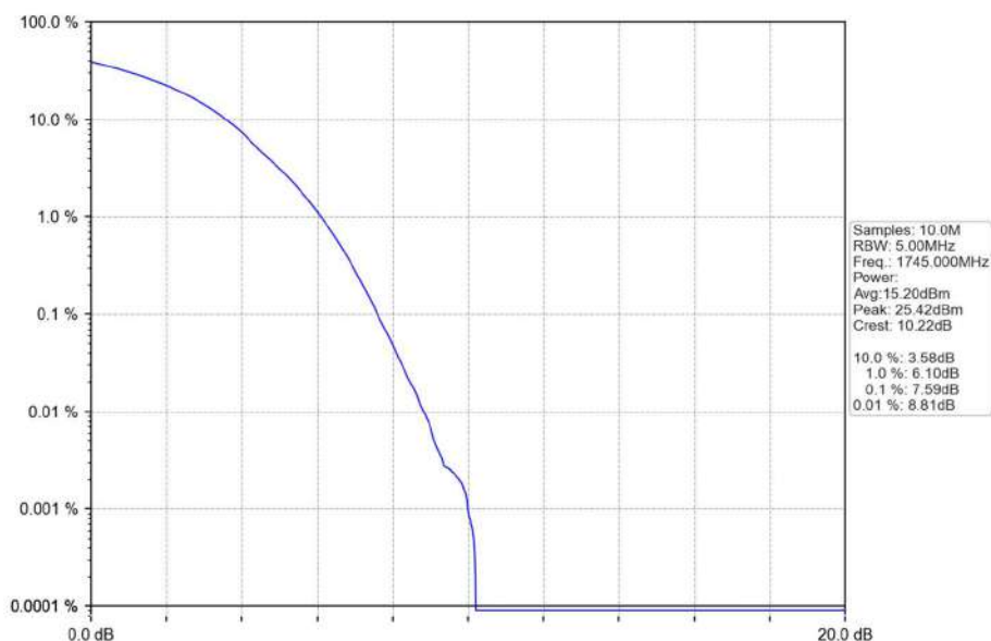
Band66_20MHz_16QAM_MCH_1745MHz_RB_100_0_NTNV
