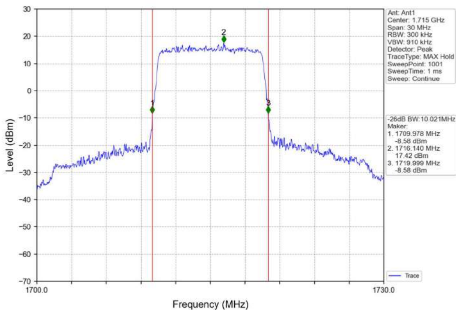
Band66_10MHz_QPSK_LCH_1715MHz_RB_50_0_NTNV
