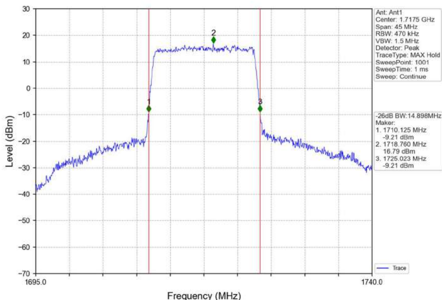
Band66_15MHz_16QAM_LCH_1717.5MHz_RB_75_0_NTNV
