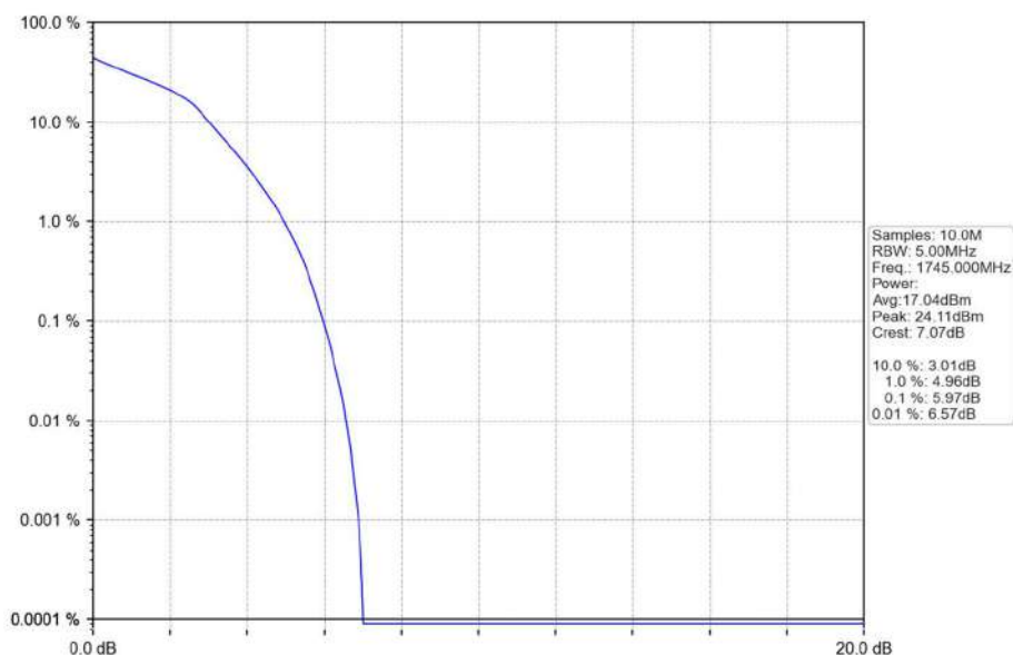
Band66_3MHz_16QAM_MCH_1745MHz_RB_15_0_NTNV
