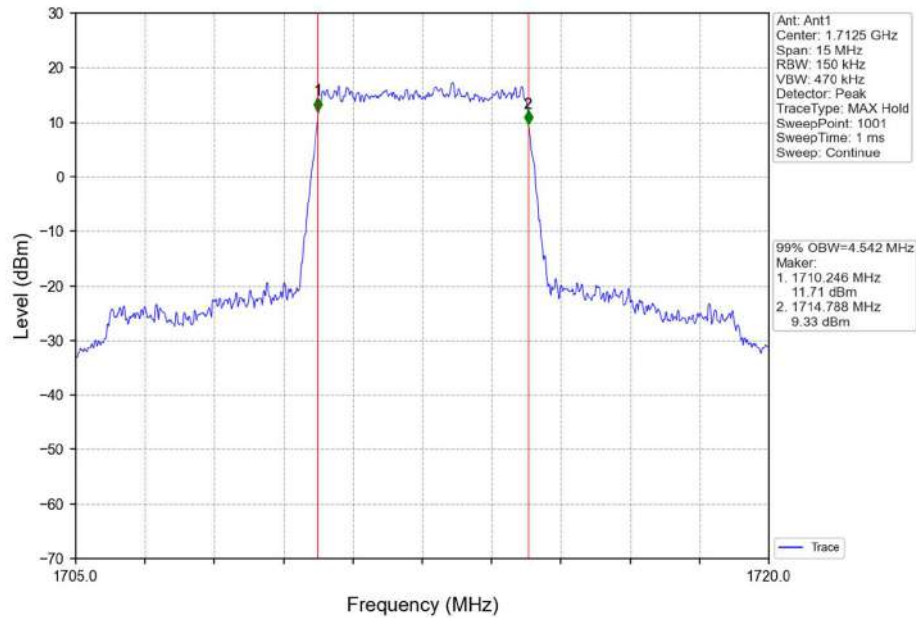
Band66_5MHz_QPSK_LCH_1712.5MHz_RB_25_0_NTNV
