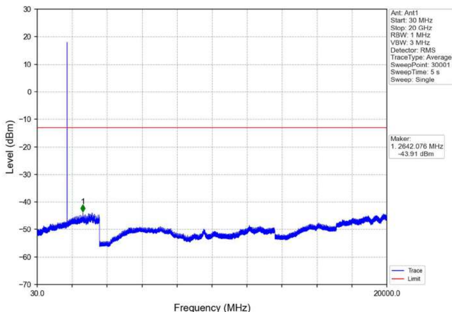
Band66_1.4MHz_QPSK_MCH_1745MHz_RB_1_0_NTNV
