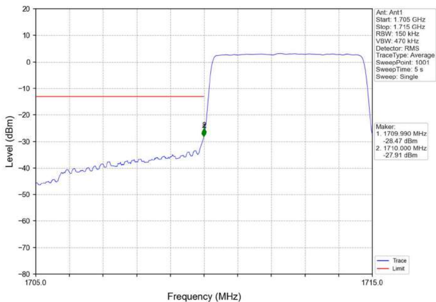
Band66_5MHz_16QAM_LCH_1712.5MHz_RB_25_0_NTNV
