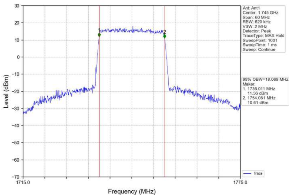
Band66_20MHz_16QAM_MCH_1745MHz_RB_100_0_NTNV
