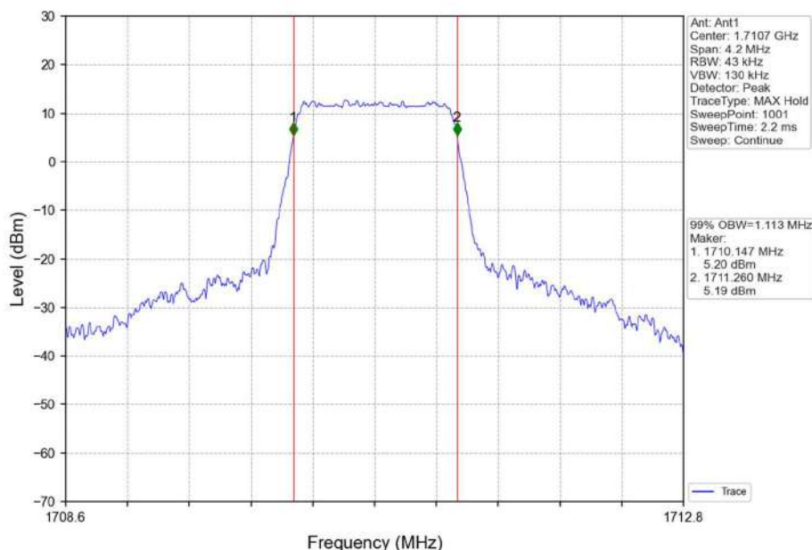
Band66_1.4MHz_16QAM_LCH_1710.7MHz_RB_6_0_NTNV
