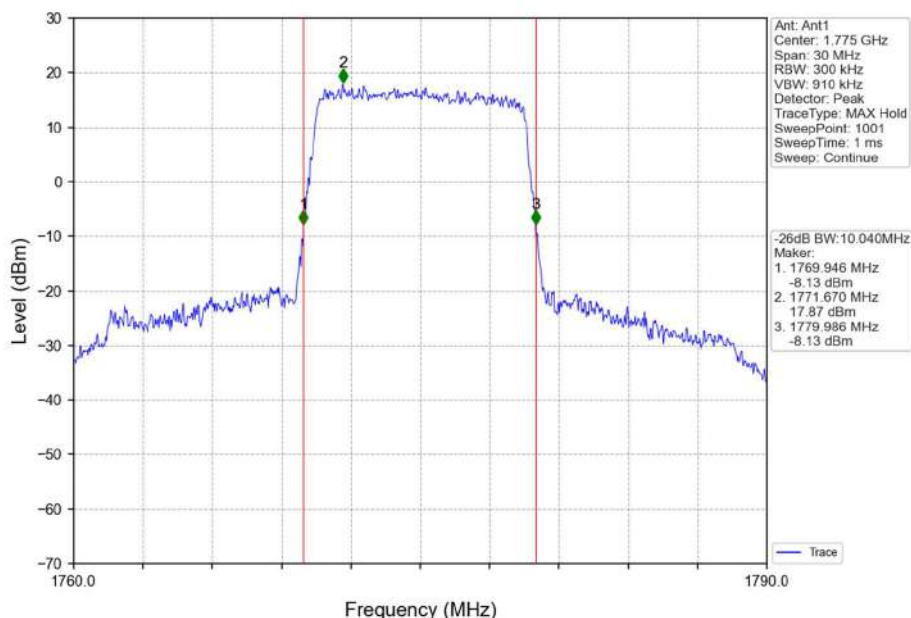
Band66_10MHz_QPSK_HCH_1775MHz_RB_50_0_NTNV
