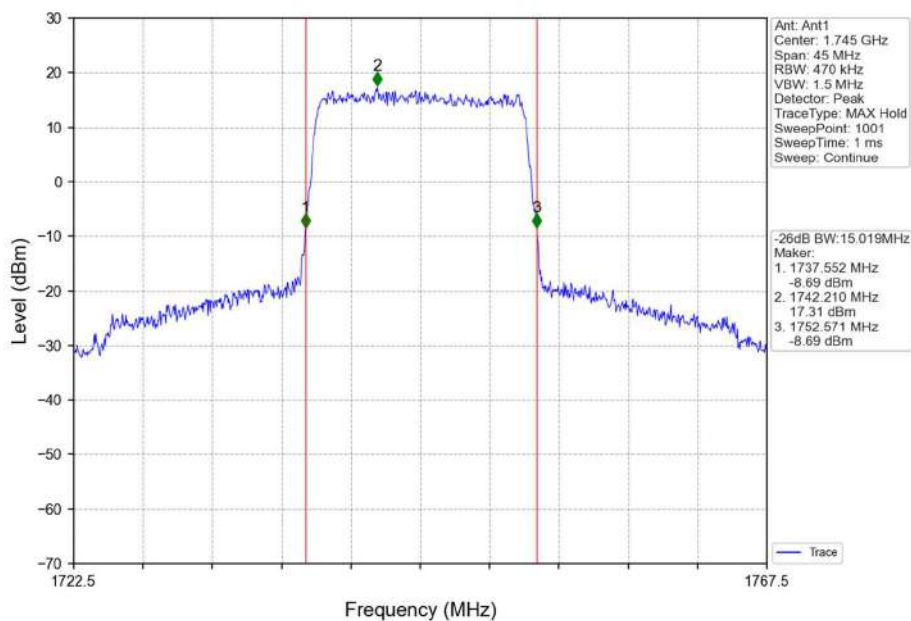
Band66_15MHz_16QAM_MCH_1745MHz_RB_75_0_NTNV
