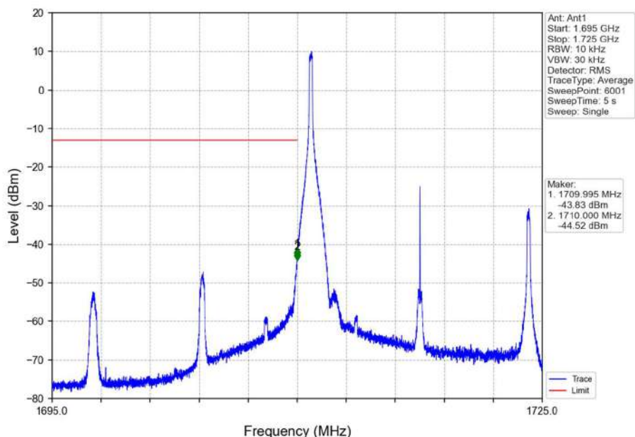
Band66_15MHz_16QAM_LCH_1717.5MHz_RB_1_0_NTNV
