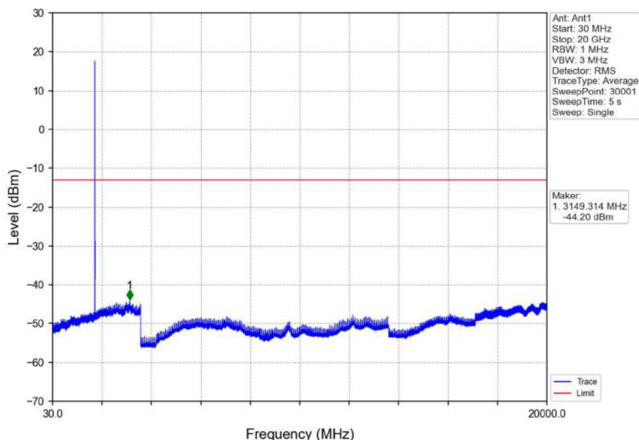
Band66_3MHz_QPSK_MCH_1745MHz_RB_1_0_NTNV
