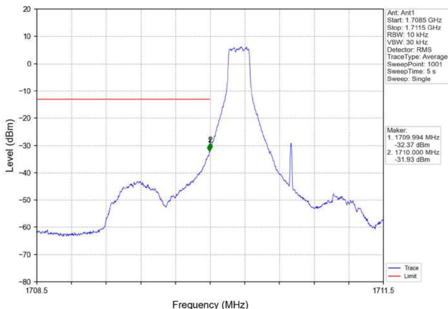
Band66_1.4MHz_16QAM_LCH_1710.7MHz_RB_1_0_NTNV
