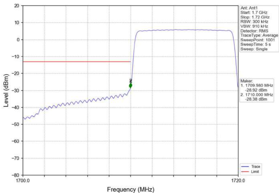
Band66_10MHz_16QAM_LCH_1715MHz_RB_50_0_NTNV
