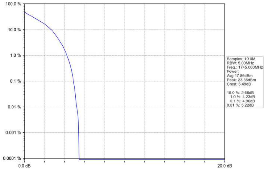
Band66_1.4MHz_QPSK_MCH_1745MHz_RB_6_0_NTNV
