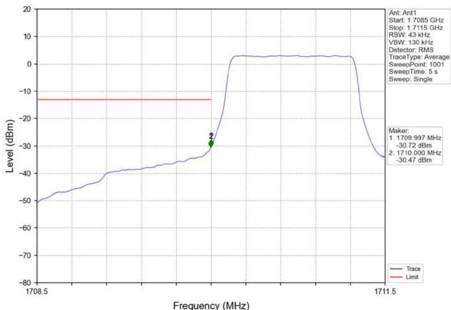
Band66_1.4MHz_16QAM_LCH_1710.7MHz_RB_6_0_NTNV
