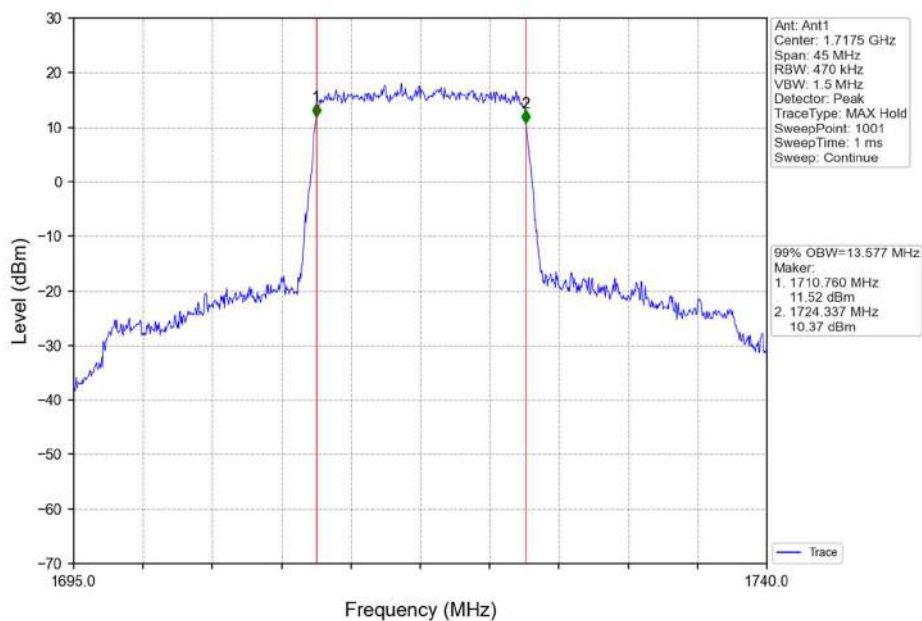
Band66_15MHz_QPSK_LCH_1717.5MHz_RB_75_0_NTNV
