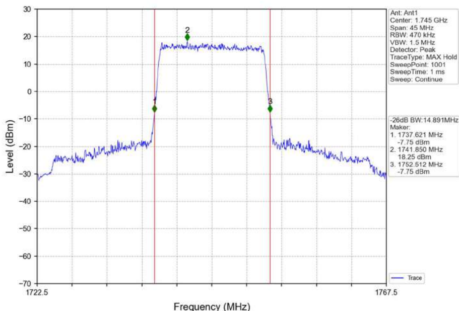
Band66_15MHz_QPSK_MCH_1745MHz_RB_75_0_NTNV
