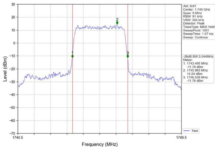
Band66_3MHz_QPSK_MCH_1745MHz_RB_15_0_NTNV
