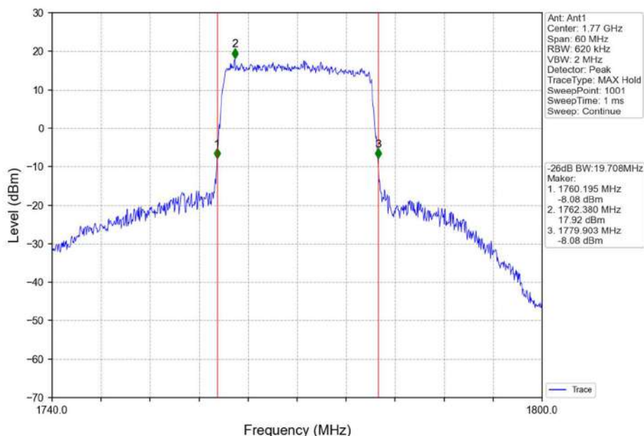
Band66_20MHz_16QAM_HCH_1770MHz_RB_100_0_NTNV
