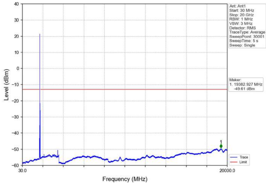
Band66_20MHz_16QAM_MCH_1745MHz_RB_1_0_NTNV
