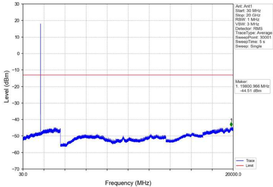
Band66_3MHz_QPSK_LCH_1711.5MHz_RB_1_0_NTNV
