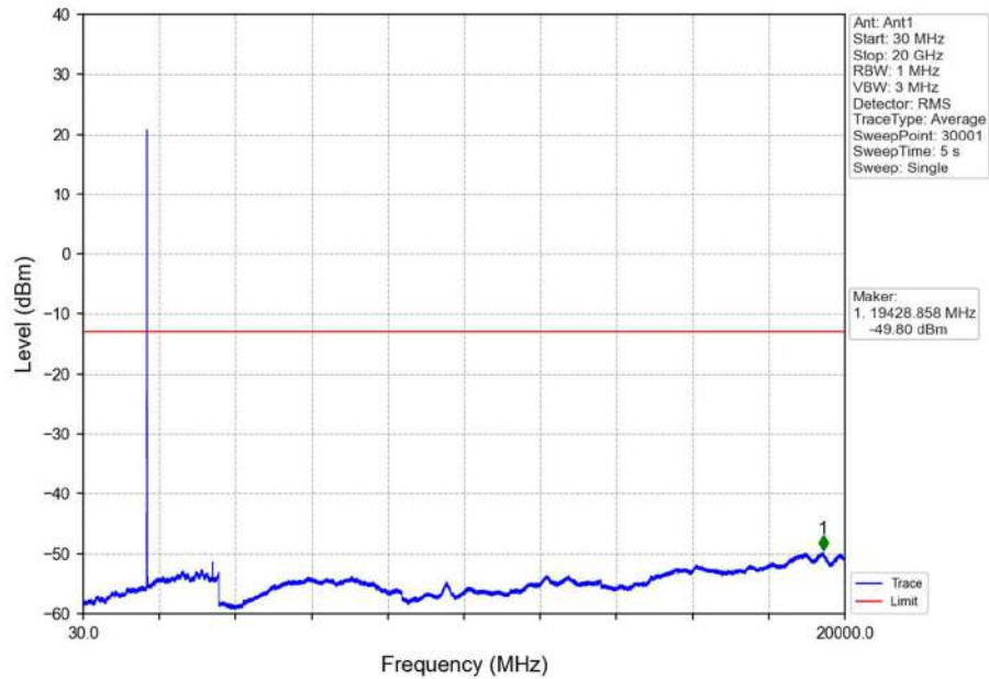
Band66_5MHz_QPSK_LCH_1712.5MHz_RB_1_0_NTNV
