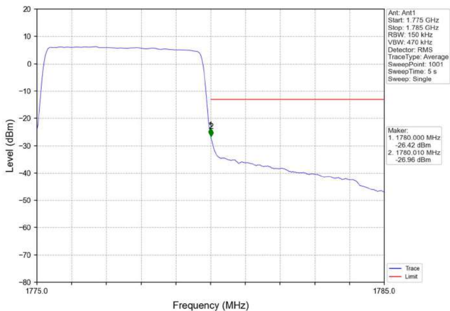
Band66_5MHz_16QAM_HCH_1777.5MHz_RB_25_0_NTNV
