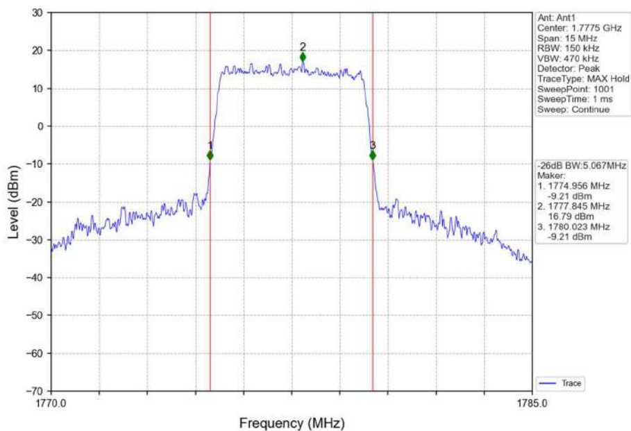
Band66_5MHz_16QAM_HCH_1777.5MHz_RB_25_0_NTNV
