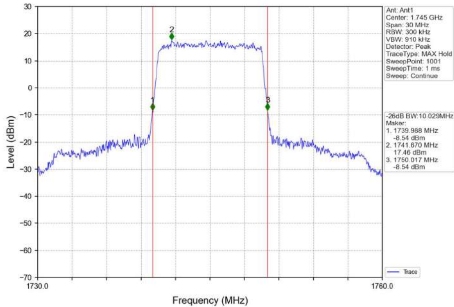
Band66_10MHz_QPSK_MCH_1745MHz_RB_50_0_NTNV
