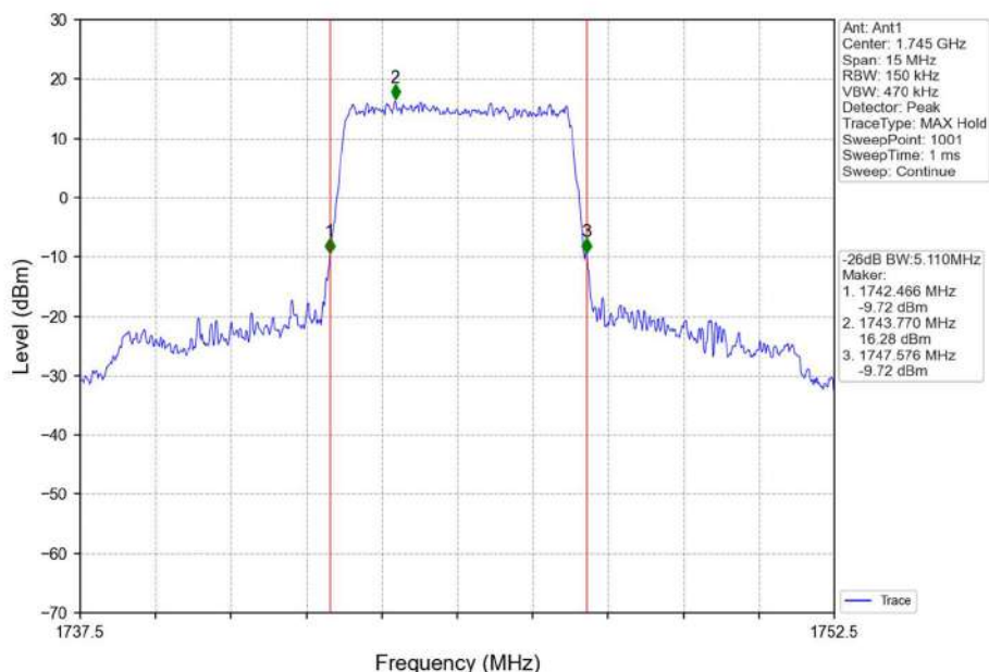
Band66_5MHz_QPSK_MCH_1745MHz_RB_25_0_NTNV
