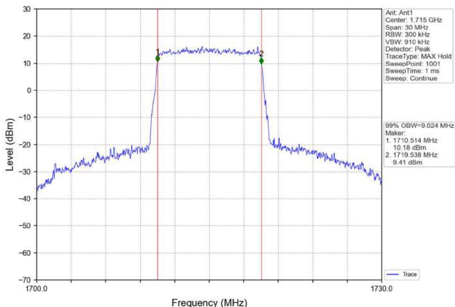
Band66_10MHz_16QAM_LCH_1715MHz_RB_50_0_NTNV
