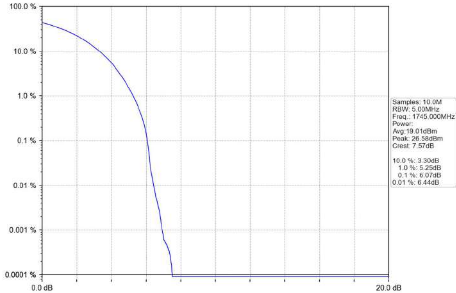
Band66_10MHz_QPSK_MCH_1745MHz_RB_50_0_NTNV
