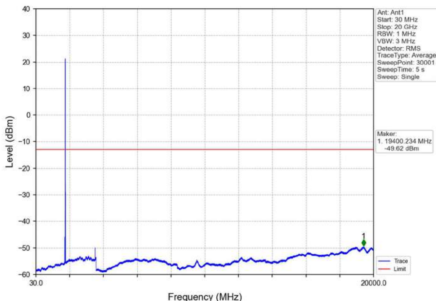
Band66_10MHz_16QAM_HCH_1775MHz_RB_1_0_NTNV
