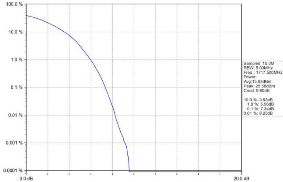
Band66_15MHz_16QAM_LCH_1717.5MHz_RB_75_0_NTNV
