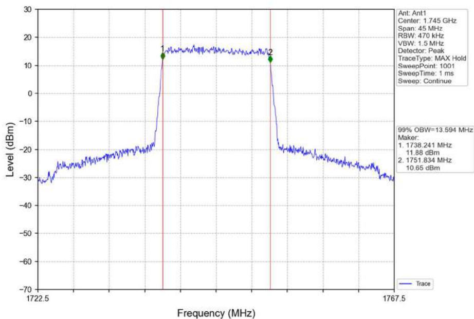
Band66_15MHz_16QAM_MCH_1745MHz_RB_75_0_NTNV
