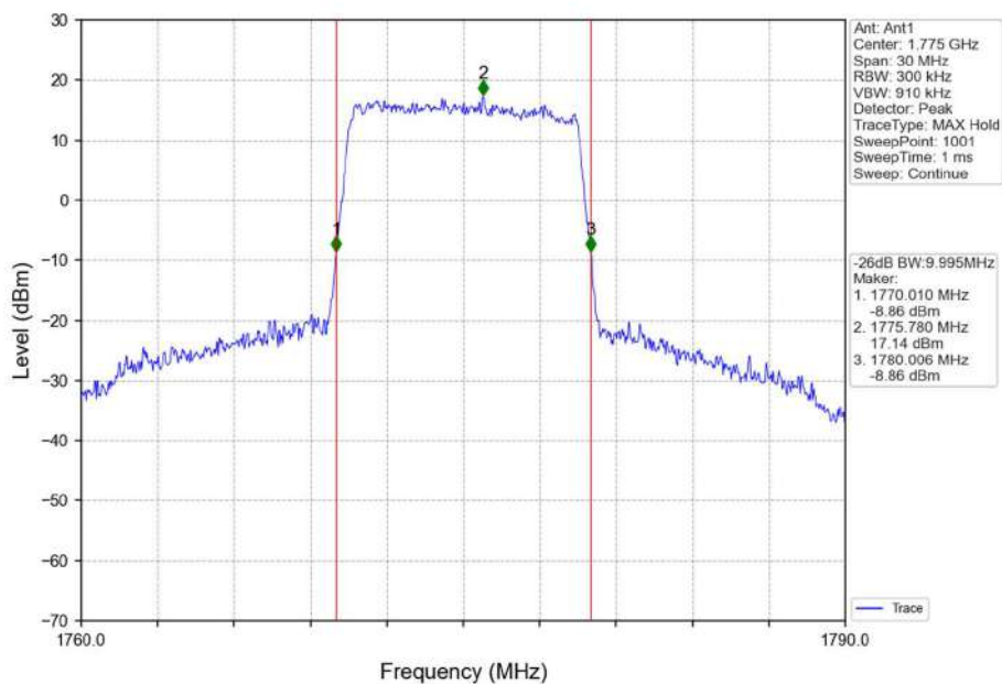
Band66_10MHz_16QAM_HCH_1775MHz_RB_50_0_NTNV
