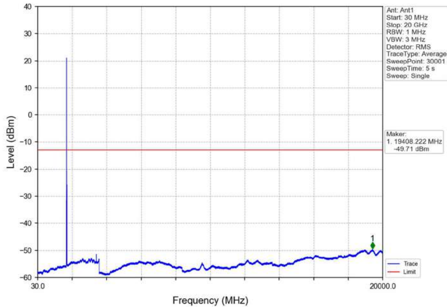
Band66_10MHz_QPSK_LCH_1715MHz_RB_1_0_NTNV
