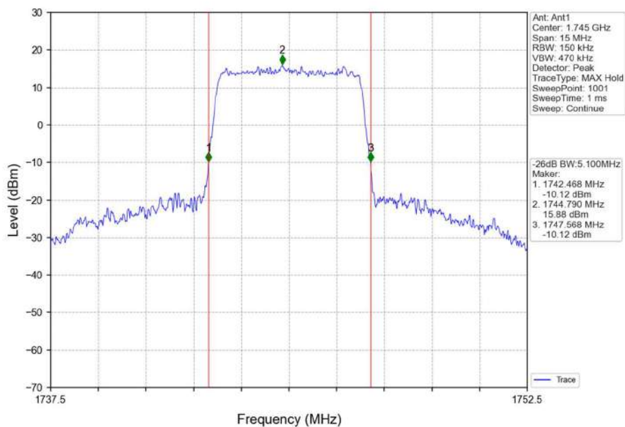
Band66_5MHz_16QAM_MCH_1745MHz_RB_25_0_NTNV
