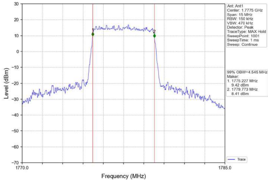
Band66_5MHz_16QAM_HCH_1777.5MHz_RB_25_0_NTNV
