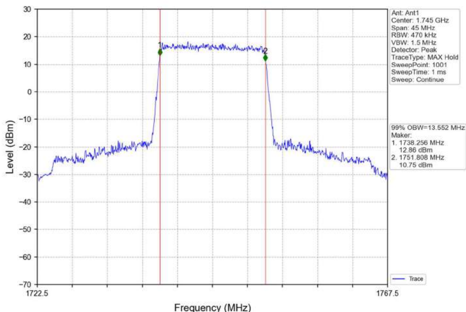
Band66_15MHz_QPSK_MCH_1745MHz_RB_75_0_NTNV
