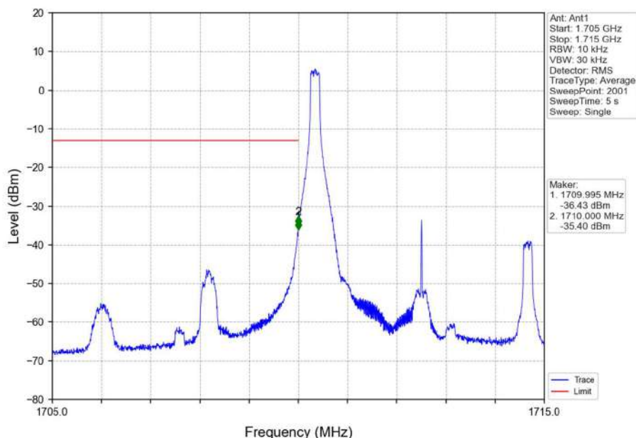
Band66_5MHz_16QAM_LCH_1712.5MHz_RB_1_0_NTNV
