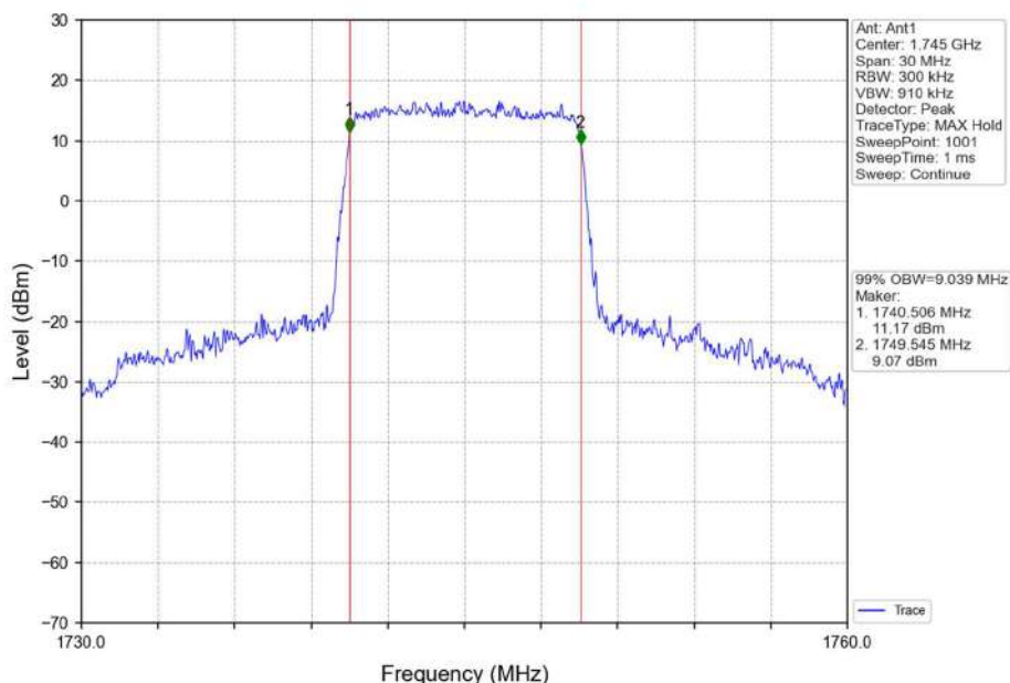
Band66_10MHz_16QAM_MCH_1745MHz_RB_50_0_NTNV
