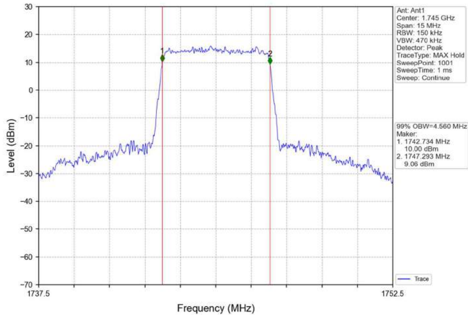
Band66_5MHz_16QAM_MCH_1745MHz_RB_25_0_NTNV
