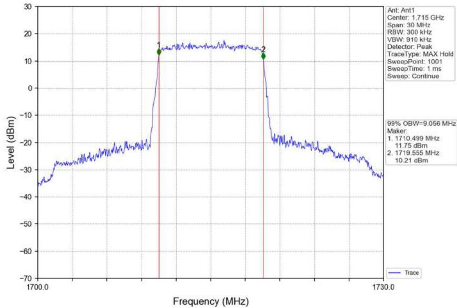
Band66_10MHz_QPSK_LCH_1715MHz_RB_50_0_NTNV
