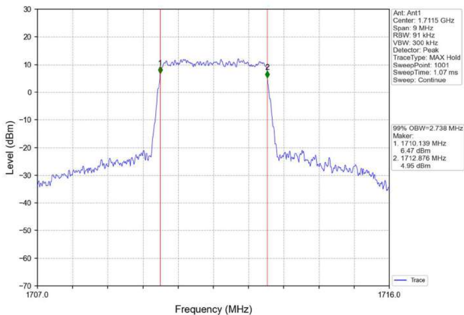
Band66_3MHz_16QAM_LCH_1711.5MHz_RB_15_0_NTNV
