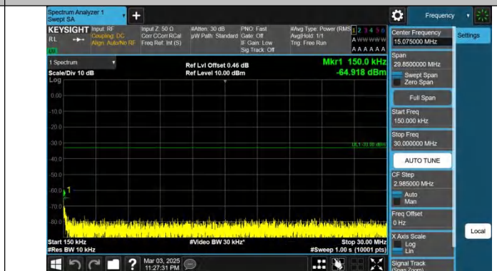
Band66-10MHz-QPSK-132622-1RB#0-0.15~30-PASS
