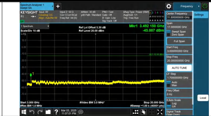
Band66-3MHz-QPSK-132322-1RB#14-3000~20000-PASS
