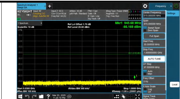
Band66-10MHz-QPSK-132022-1RB#49-30~1000-PASS
