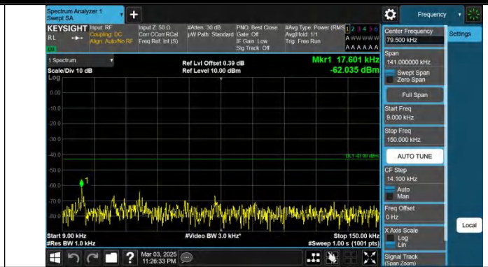
Band66-10MHz-QPSK-132322-1RB#49-0.009~0.15-PASS
