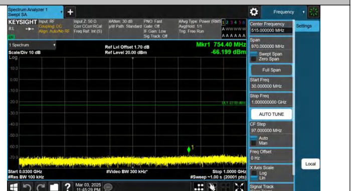
Band66-20MHz-QPSK-132322-1RB#99-30~1000-PASS
