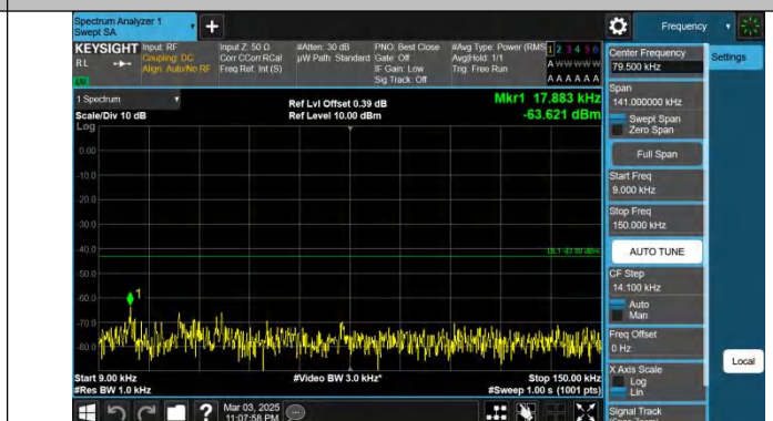
Band66-3MHz-QPSK-132657-1RB#14-0.009~0.15-PASS
