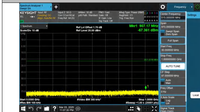
Band66-3MHz-QPSK-132657-1RB#0-30~1000-PASS
