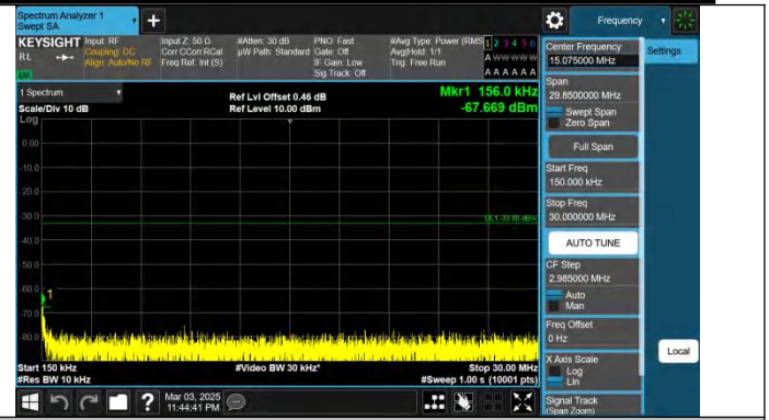
Band66-20MHz-QPSK-132322-1RB#0-0.15~30-PASS
