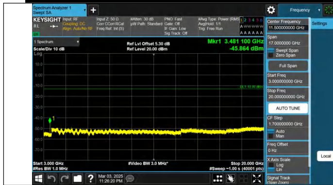
Band66-10MHz-QPSK-132322-1RB#0-3000~20000-PASS
