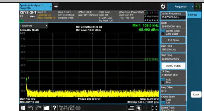
Band66-3MHz-QPSK-132657-1RB#0-0.15~30-PASS
