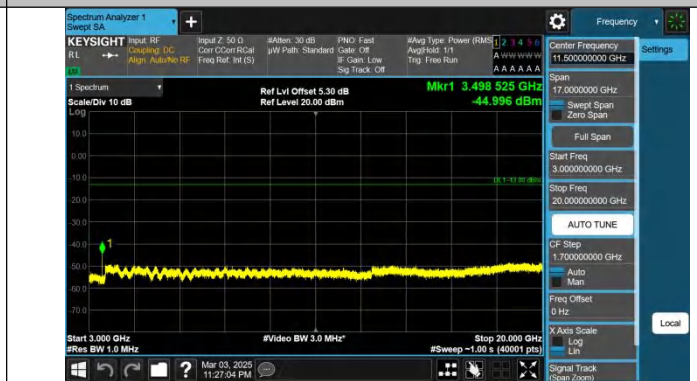
Band66-10MHz-QPSK-132322-1RB#49-3000~20000-PASS
