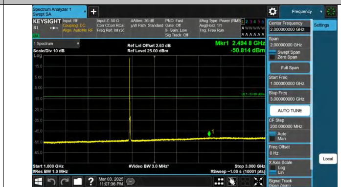
Band66-3MHz-QPSK-132657-1RB#0-1000~3000-PASS
