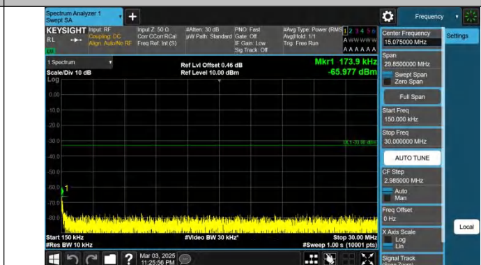
Band66-10MHz-QPSK-132322-1RB#0-0.15~30-PASS
