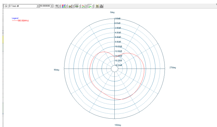
GSM900 / WCDMA B8 / LTE B8 Phi=90deg
