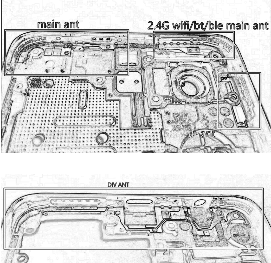
Antenna Photo:
