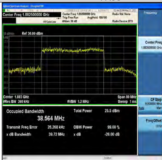
NTNV-N25-15kHz-40MHz-CP-64QAM-Mid-Outer_Full -----PASS
