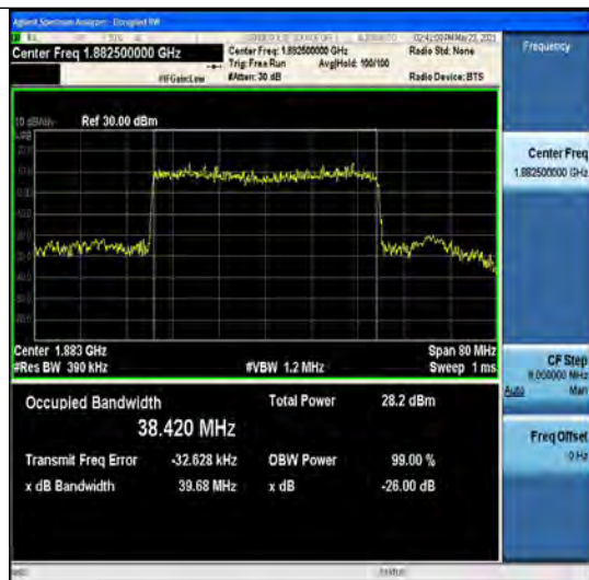
NTNV-N25-15kHz-40MHz-DFT-QPSK-Mid-Outer_Fu II-----PASS
