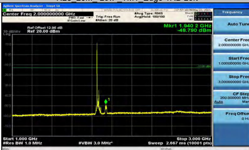
N25_20M_Low_TM1_Edge_1RB_Left
