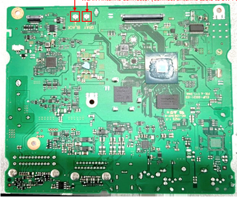
Main PCB F2 side
