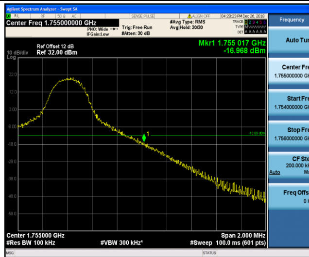
Band4_10MHz_16QAM_20350_1RB#49
