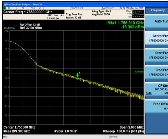
Band4_20MHz_QPSK_20300_1RB#99
