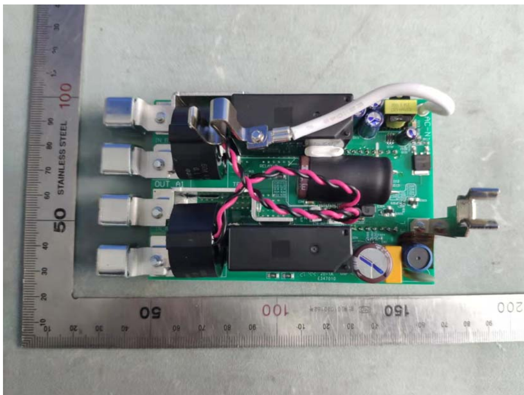
FIGURE 8 QO 60A RELAYWITH CURENT TRANSFORMER PON (M/N: GPM-QP1R60240-21) MAINBOARD FRONT
