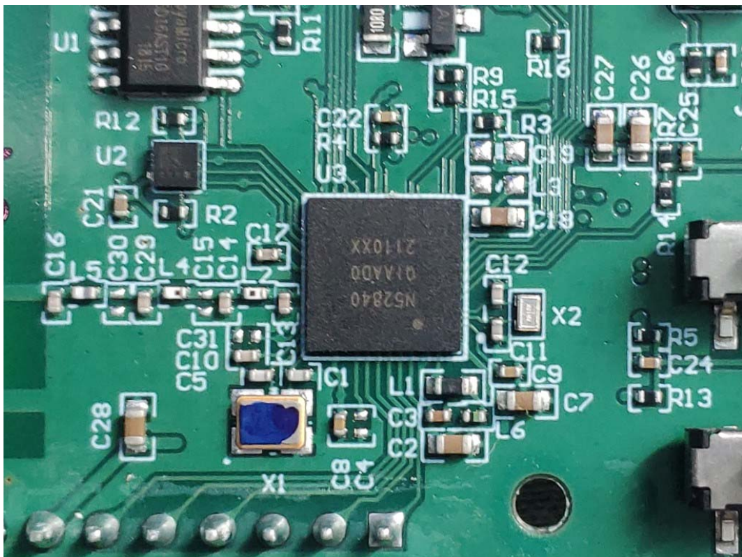
FIGURE 10 QO 60A RELAYWITH CURENT TRANSFORMER PON (M/N: GPM-QP1R60240-21) CHIP & CRYSTAL ON MAINBOARD
