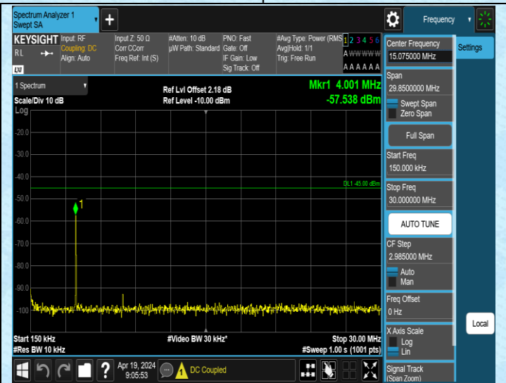
Band41_10MHz_QPSK_41190_1RB#0_0.15~30_0.15~30
