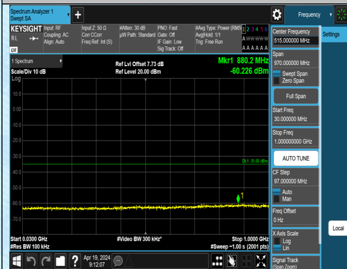
Band41_15MHz_QPSK_41165_1RB#0_30~1000_30~1000
