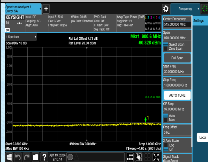
Band41_15MHz_QPSK_40590_1RB#0_30~1000_30~1000
