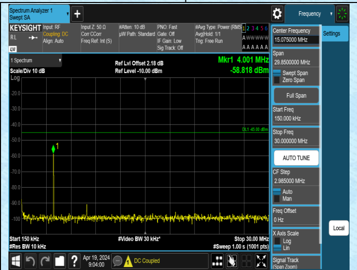
Band41_10MHz_QPSK_40590_1RB#0_0.15~30_0.15~30
