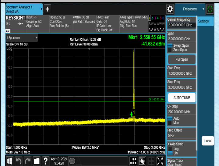
Band41_10MHz_QPSK_40590_1RB#0_1000~3000_1000~3000
