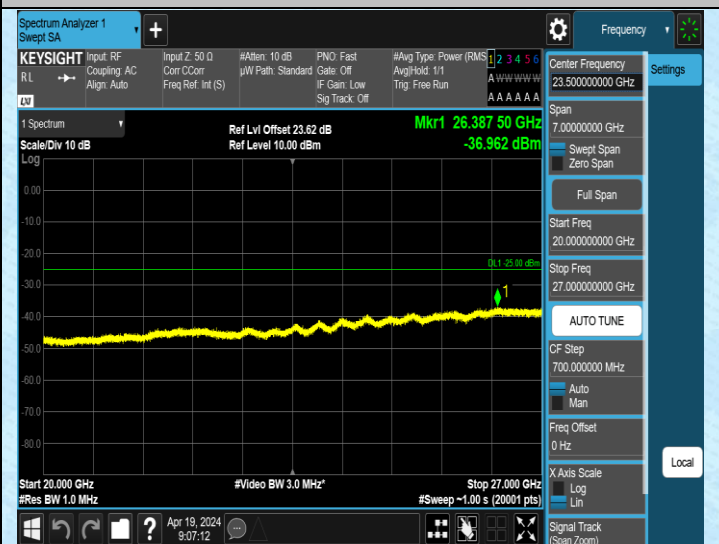
Band41_10MHz_QPSK_41190_1RB#0_20000~27000_20000~2
