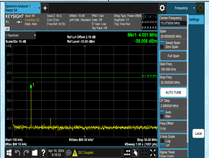
Band41_20MHz_QPSK_41140_1RB#0_0.15~30_0.15~30
