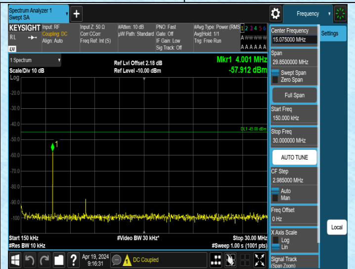
Band41_20MHz_QPSK_40590_1RB#0_0.15~30_0.15~30
