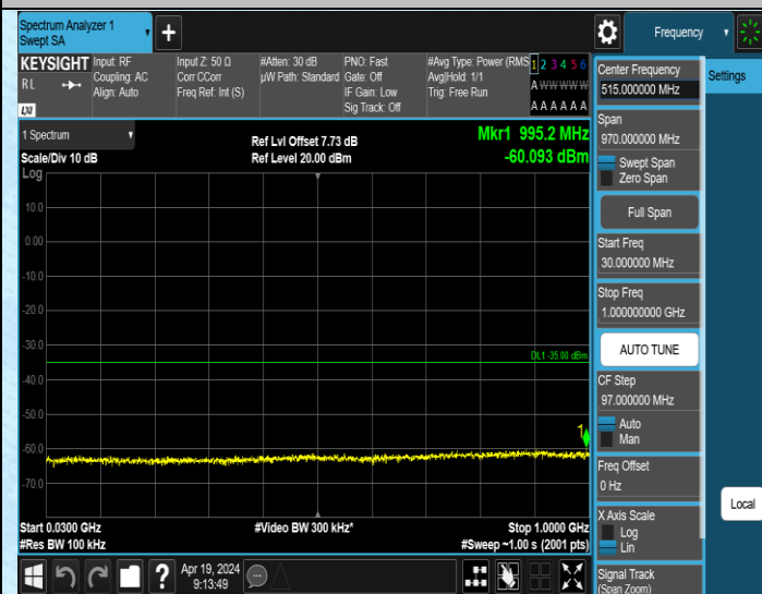
Band41_20MHz_QPSK_40140_1RB#0_30~1000_30~1000
