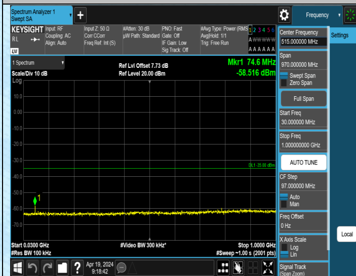
Band41_20MHz_QPSK_41140_1RB#0_30~1000_30~1000
