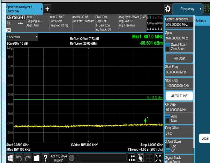
Band41_10MHz_QPSK_41190_1RB#0_30~1000_30~1000
