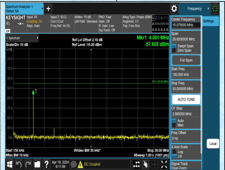
Band41_15MHz_QPSK_41165_1RB#0_0.15~30_0.15~30
