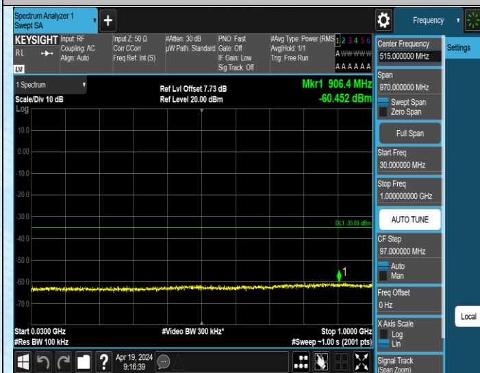
Band41_20MHz_QPSK_40590_1RB#0_30~1000_30~1000
