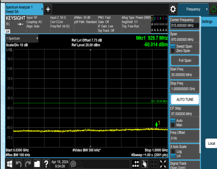
Band41_10MHz_QPSK_40590_1RB#0_30~1000_30~1000
