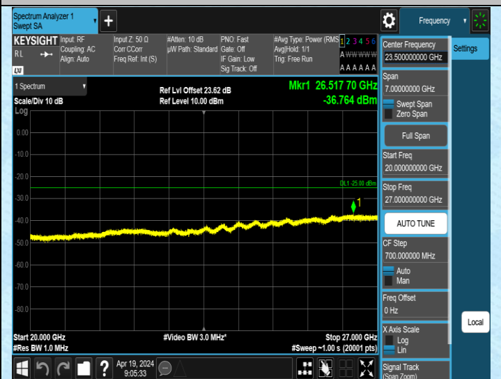
Band41_10MHz_QPSK_40590_1RB#0_20000~27000_20000~2
