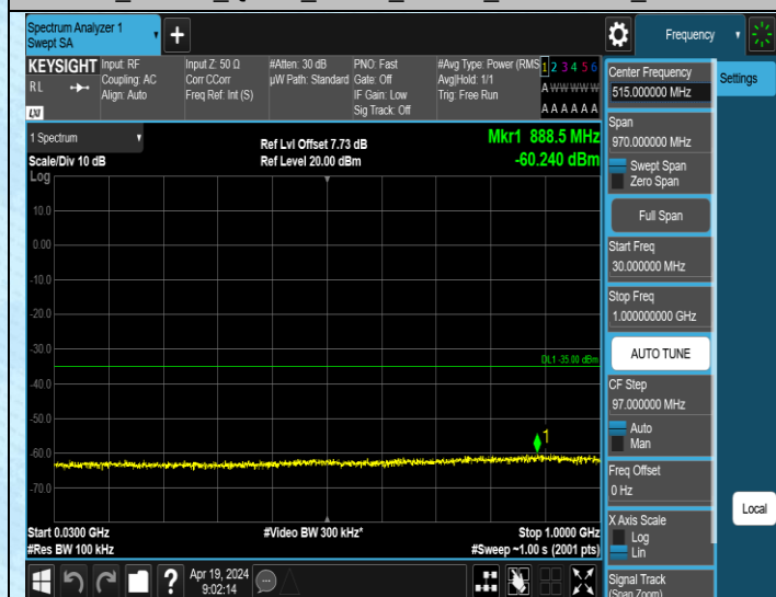
Band41_10MHz_QPSK_40090_1RB#0_30~1000_30~1000
