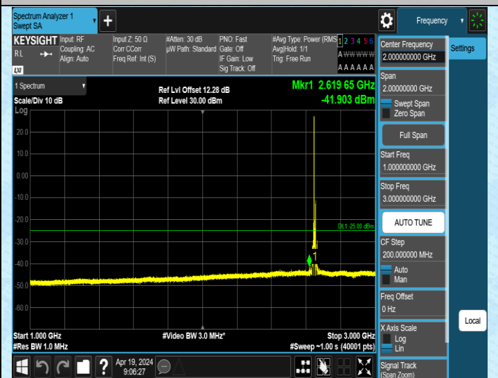
Band41_10MHz_QPSK_41190_1RB#0_1000~3000_1000~3000
