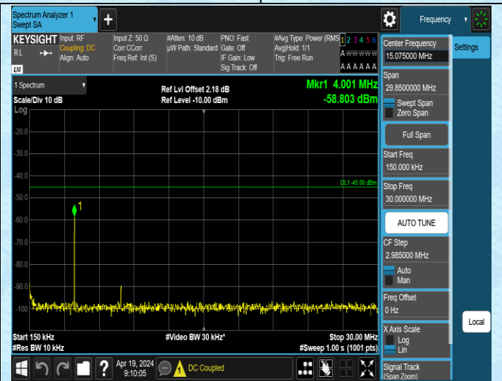
Band41_15MHz_QPSK_40590_1RB#0_0.15~30_0.15~30
