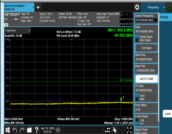
Band41_15MHz_QPSK_40115_1RB#0_30~1000_30~1000
