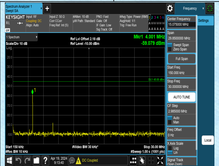
Band41_20MHz_QPSK_40140_1RB#0_0.15~30_0.15~30
