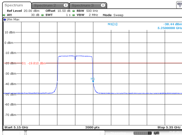
ax40_5230MHz_RU_Full_Chain 2
