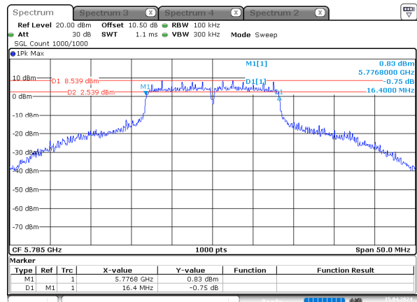
a_5785MHz_Chain 0
