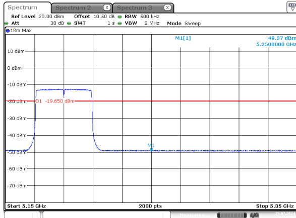
ax40_5190MHz_RU_Full_Chain 2
