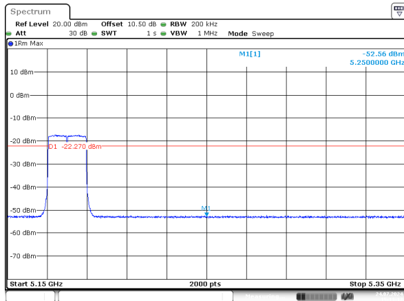
ax20_5180MHz_RU_Full_Chain 0
