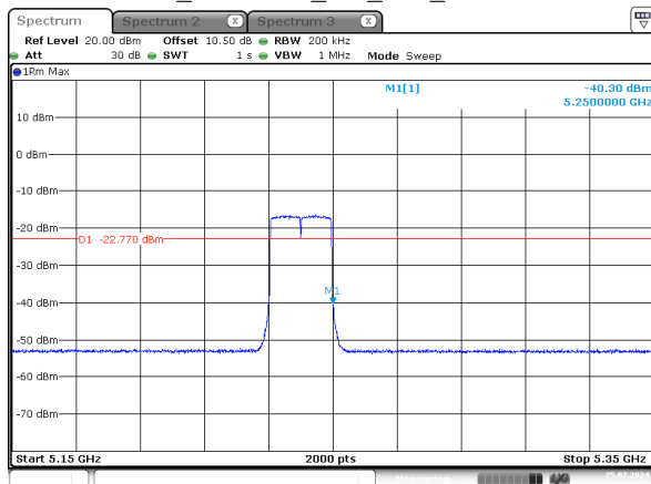
ax20_5240MHz_RU_Full_Chain 2
