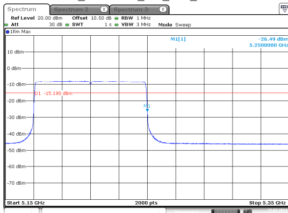
ax80_5210MHz_RU_Full_Chain 2
