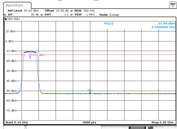
a_5180MHz_Chain 1
