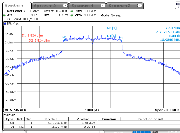
a_5745MHz_Chain 0
