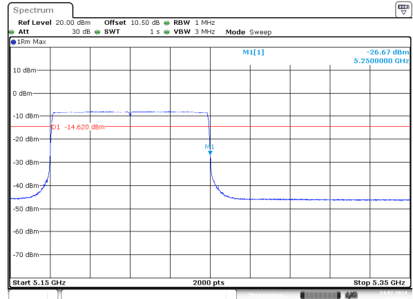
ax80_5210MHz_RU_Full_Chain 1
