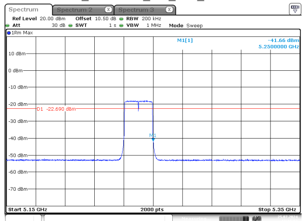
ax20_5240MHz_RU_Full_Chain 3
