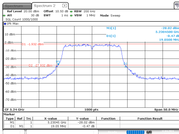
a_5240MHz_Chain 0
