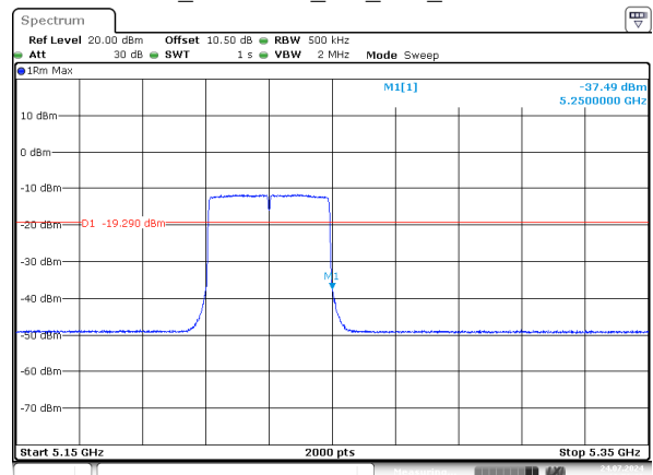
ax40_5230MHz_RU_Full_Chain 1
