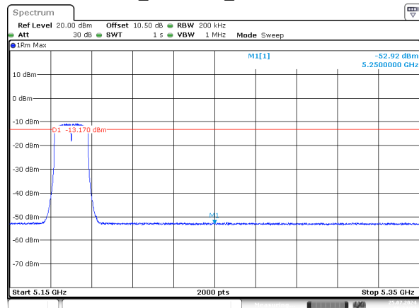
a_5180MHz_Chain 0
