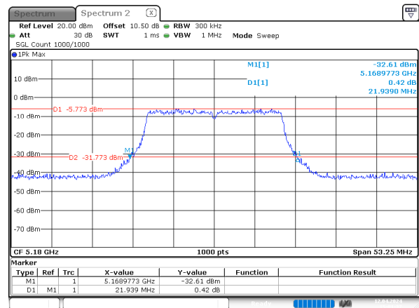
n20_5180MHz_Chain 0
