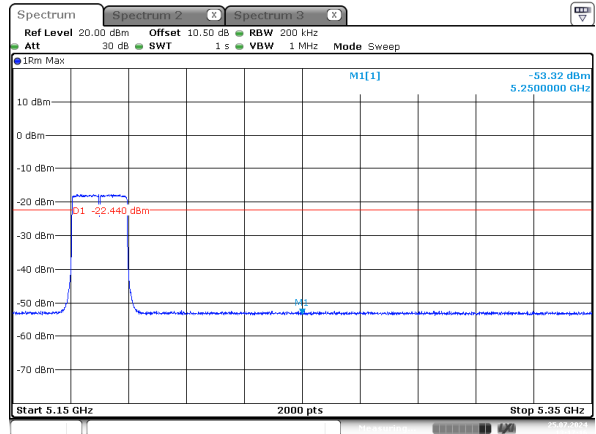
ax20_5180MHz_RU_Full_Chain 3
