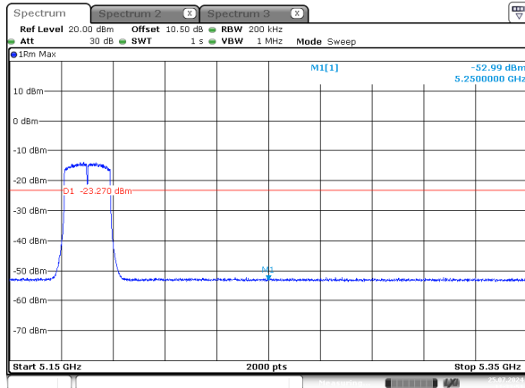
n20_5180MHz_Chain 2
