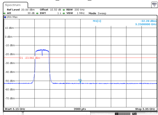
n20_5200MHz_Chain 1
