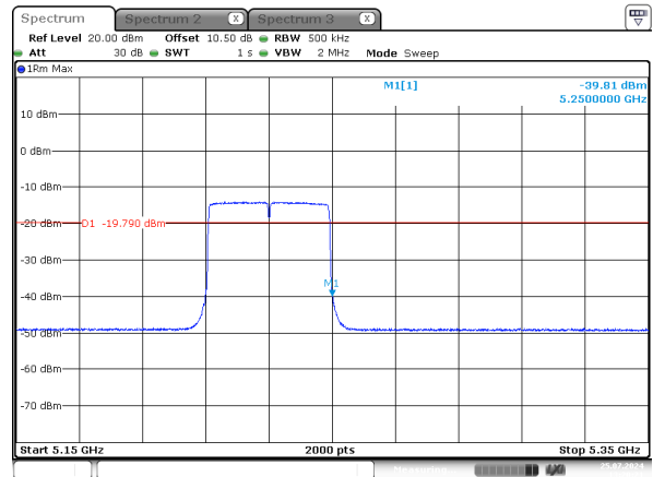
ax40_5230MHz_RU_Full_Chain 3
