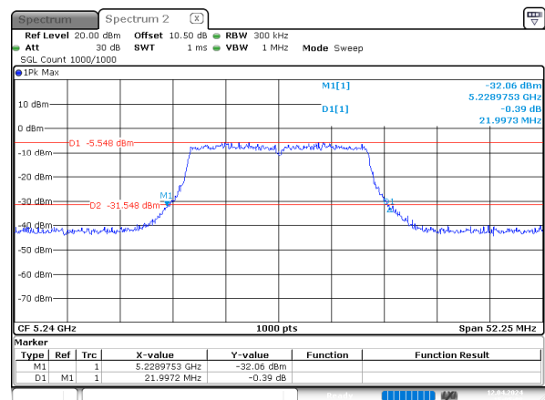
n20_5240MHz_Chain 0
