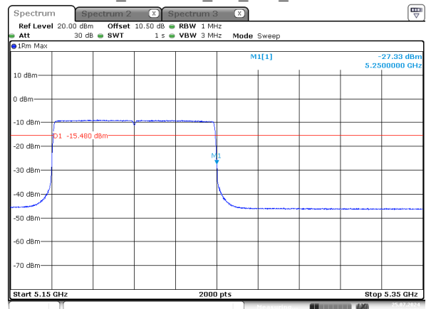
ax80_5210MHz_RU_Full_Chain 3
