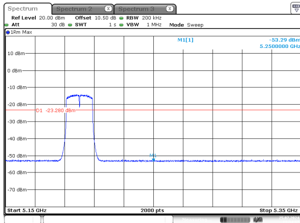
n20_5200MHz_Chain 2
