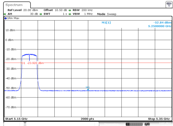
n20_5180MHz_Chain 1
