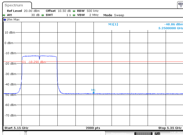
ax40_5190MHz_RU_Full_Chain 0
