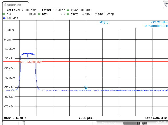
n20_5180MHz_Chain 0
