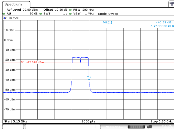
ax20_5240MHz_RU_Full_Chain 0
