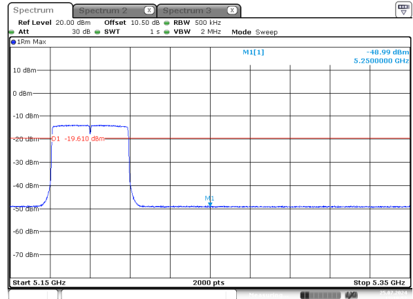
ax40_5190MHz_RU_Full_Chain 3
