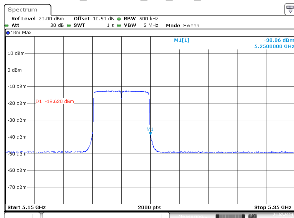
ax40_5230MHz_RU_Full_Chain 0
