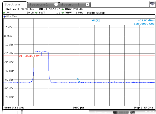
ax20_5200MHz_RU_Full_Chain 3
