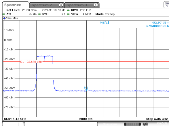
ax20_5200MHz_RU_Full_Chain 2
