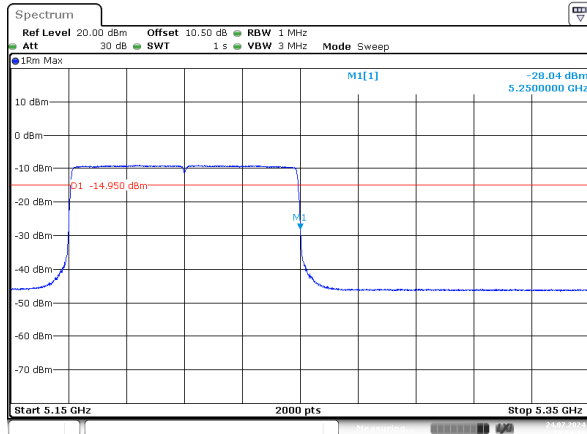
ax80_5210MHz_RU_Full_Chain 0
