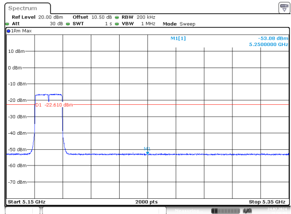
ax20_5180MHz_RU_Full_Chain 1
