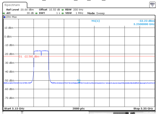
ax20_5200MHz_RU_Full_Chain 1
