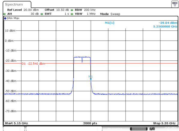
ax20_5240MHz_RU_Full_Chain 1
