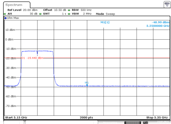
ax40_5190MHz_RU_Full_Chain 1
