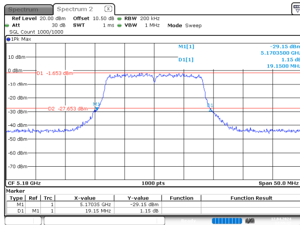
a_5180MHz_Chain 0
