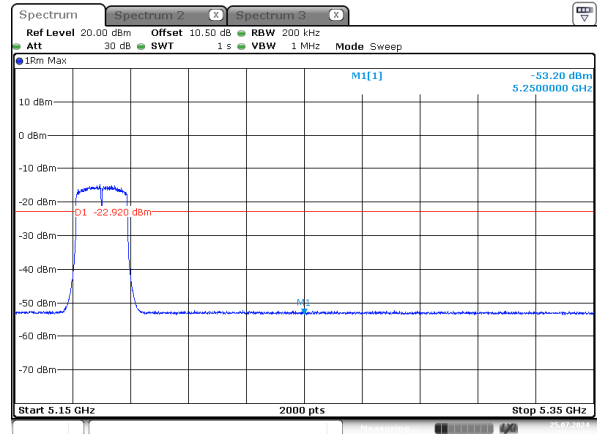
n20_5180MHz_Chain 3
