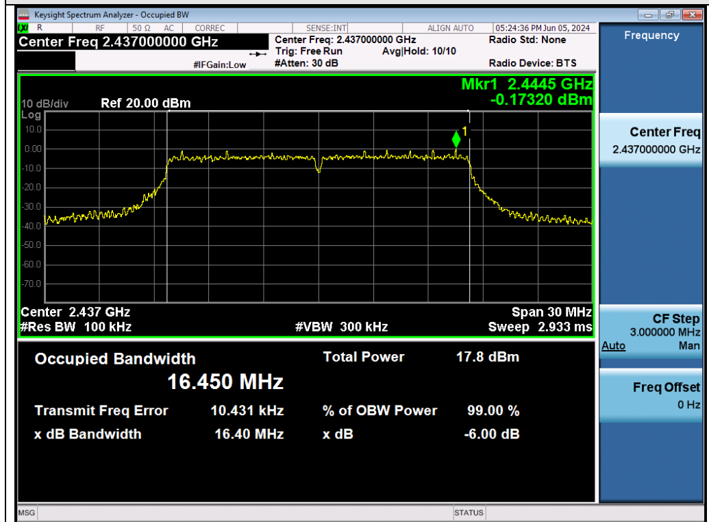
Test_Graph_802.11g_ANT1_2437_6Mbps_DTBSW
