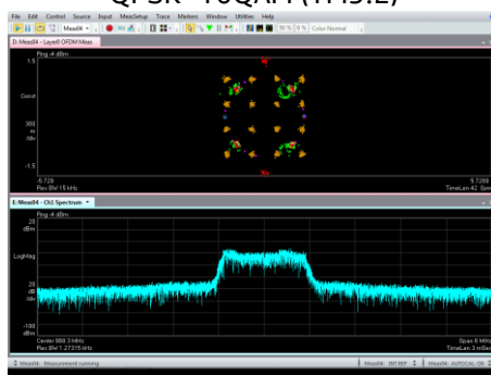
QPSK+16QAM (TM3.2)
