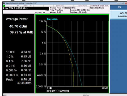
PAR_TM3.1a_3C_1.4+1.4+ NBLoT_863_864_868_TX1_2tx_868
