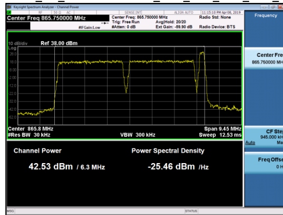
Ch_Power_TM3.1a_3C_1.4+1.4+NBIoT_863_864_868_TX1_4tx (NBIoT_SA)
