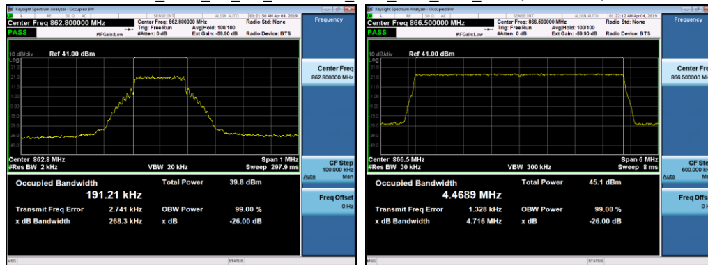
OBW_TM3_1a_2C_NBIoT+5_862_866_TX1_862 (NB-IoT SA)
