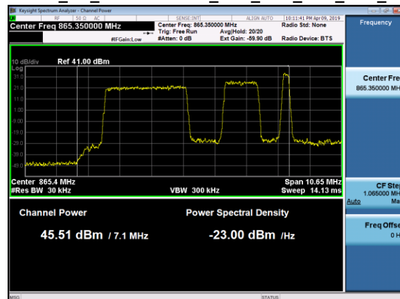
Ch_Power_TM3.1a_3C_3+1.4+NBlot_863_867_868_TX1_2tx (NBlot_SA)
