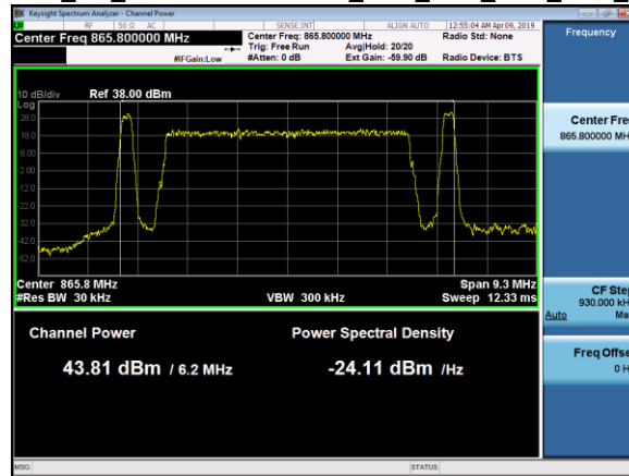
Ch_Power_TM3.1a_3C_NBIoT+5+ NBIoT_862_865_868_TX1_4tx (NBIoT_2SA)
