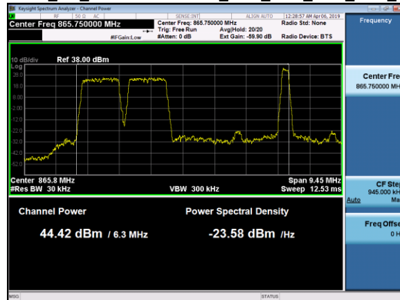
Ch_Power_TM3.1a_3C_1.4+1.4+ NBIoT_863_864_868_TX1_2tx (NBIoT_SA)
