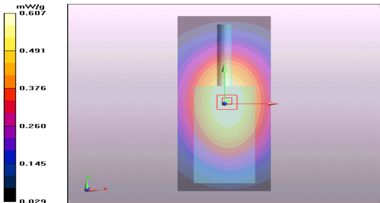
Figure 1: Face held for Digital Modulation at 12.5KHz Channel Separation Front towards Phantom 435.5 MHz
