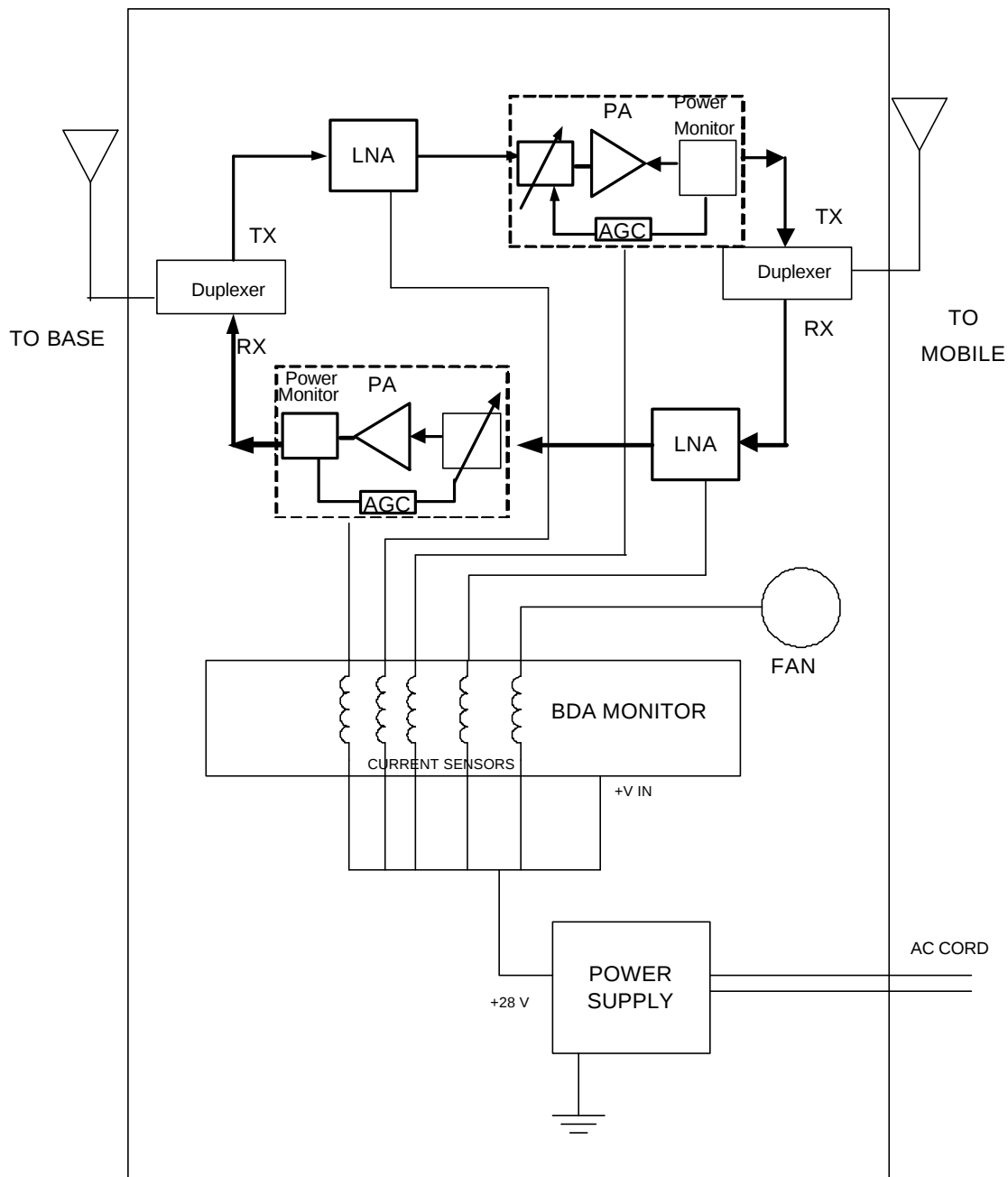
BDA-ESMR-50W90 ELELCTRICAL SCHEMATICS
