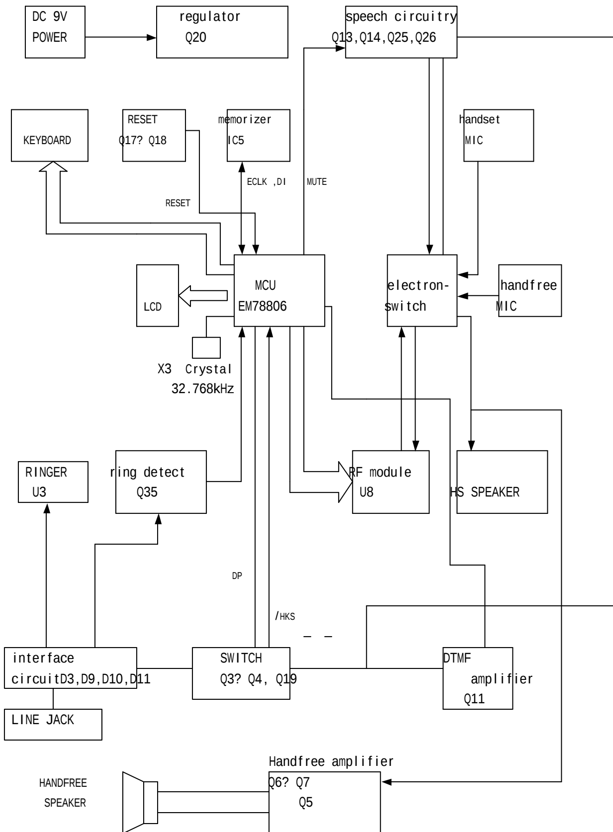
29660 block drawing (base unit)
