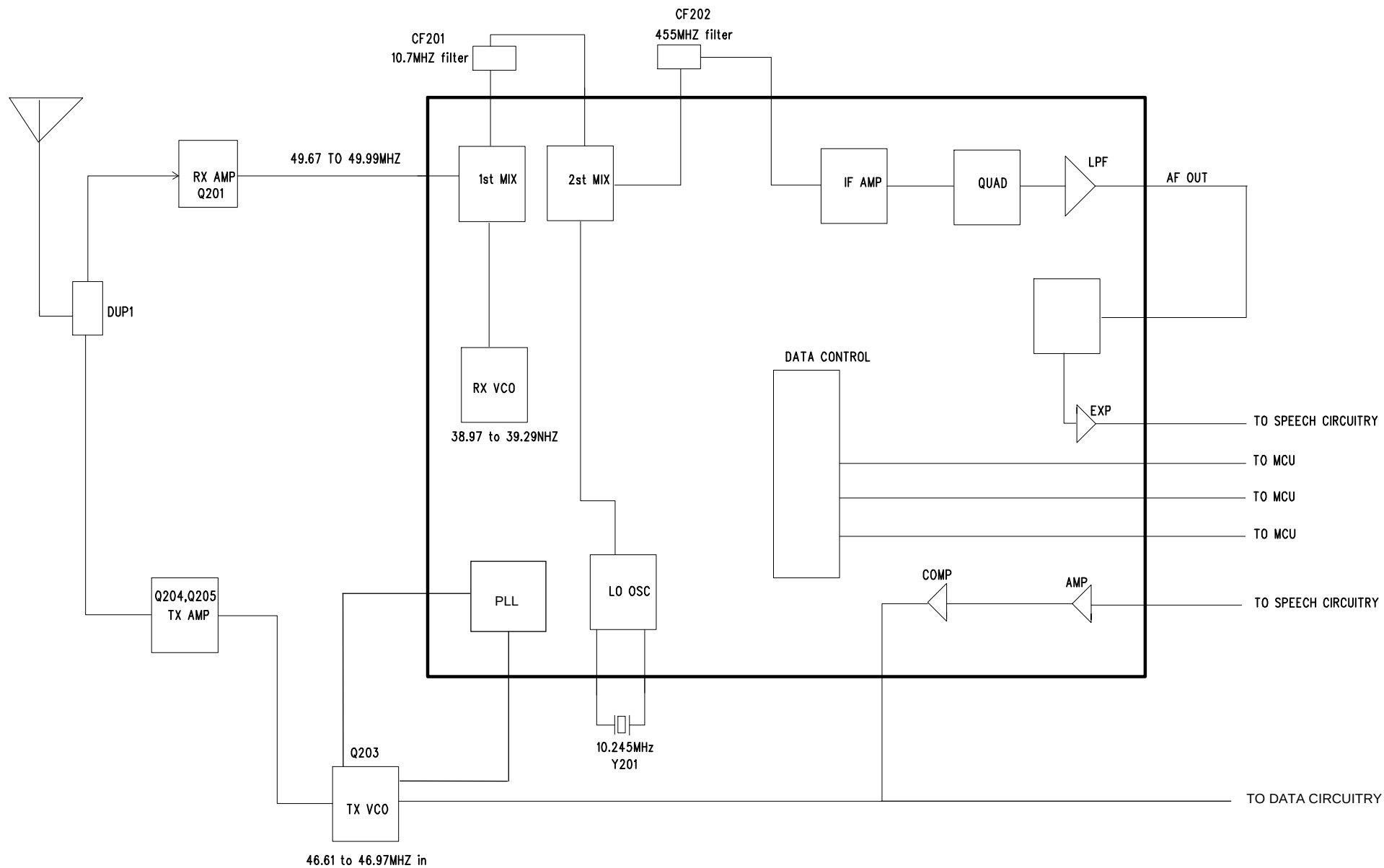
26760/29660 RF Module block drawing(base unit)
