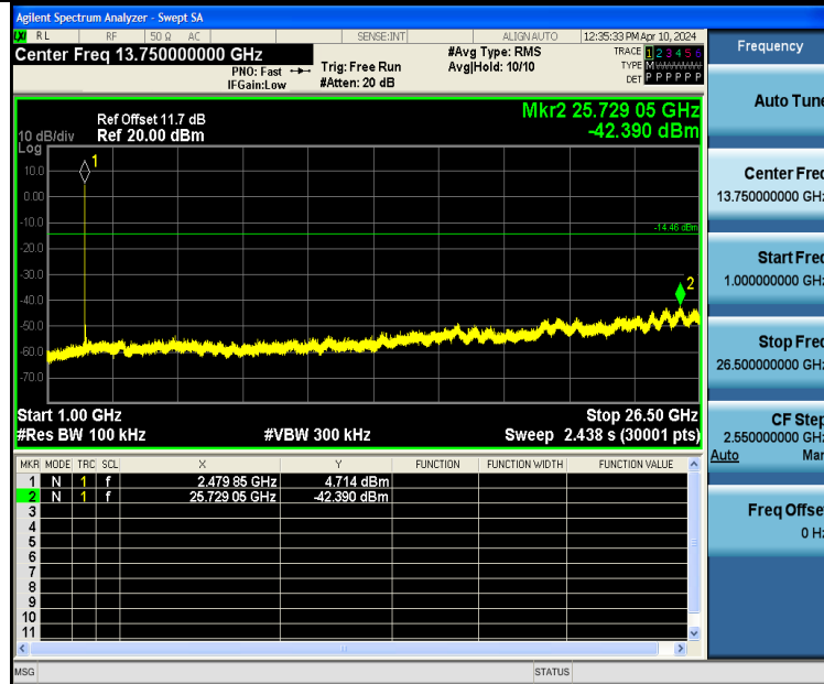
BLE_1M-Ant1-2480-1000~26500-PASS
