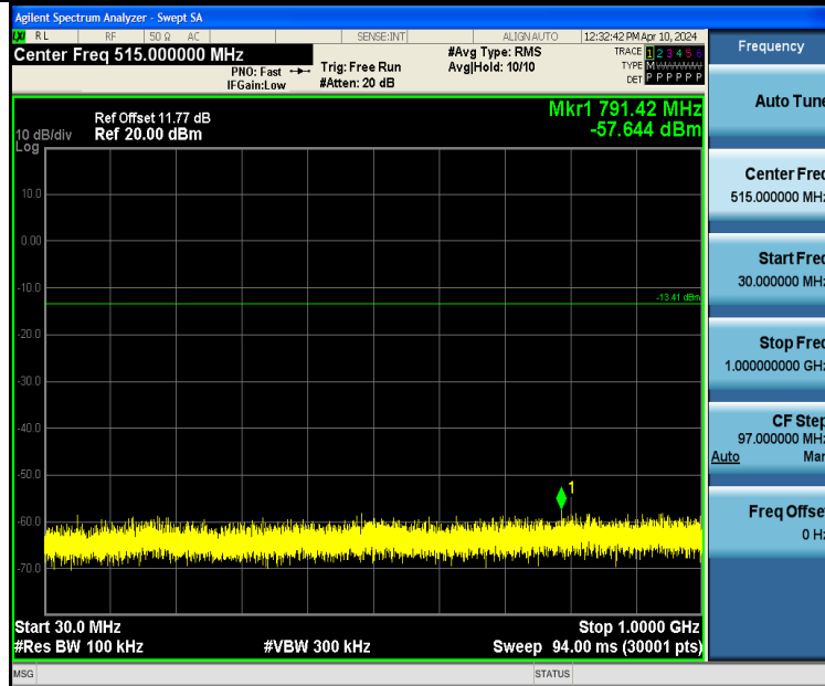
BLE_1M-Ant1-2440-30~1000-PASS
