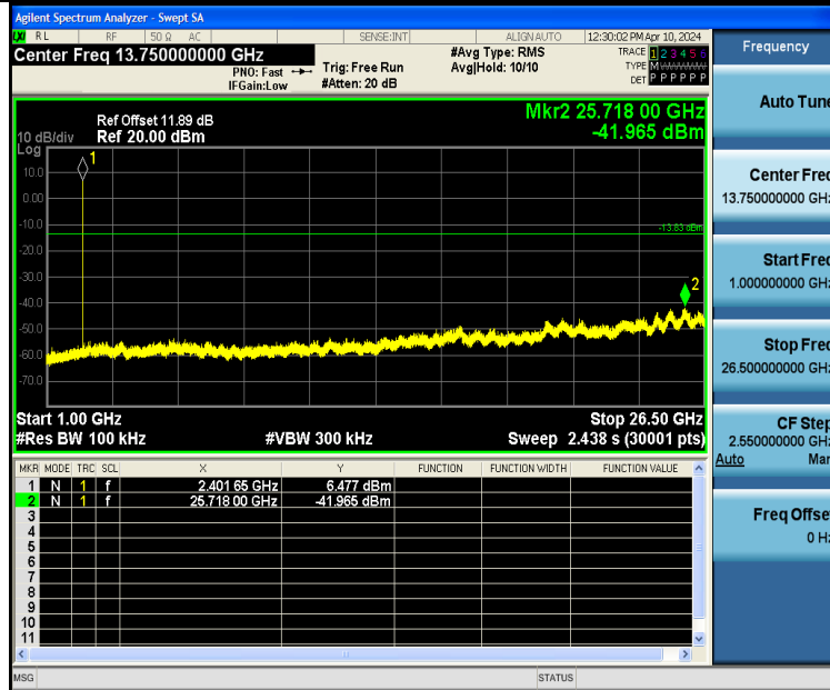
BLE_1M-Ant1-2402-1000~26500-PASS
