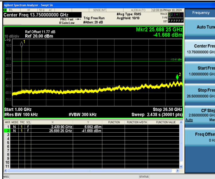
BLE_1M-Ant1-2440-1000~26500-PASS
