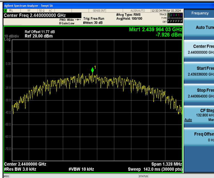
BLE_1M-Ant1-2440-PASS
