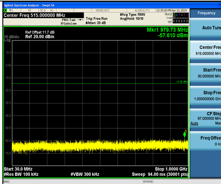
BLE_1M-Ant1-2480-30~1000-PASS
