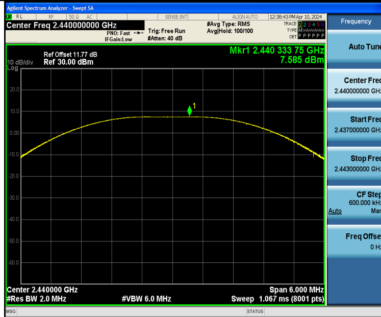
BLE_2M-Ant1-2440-PASS
