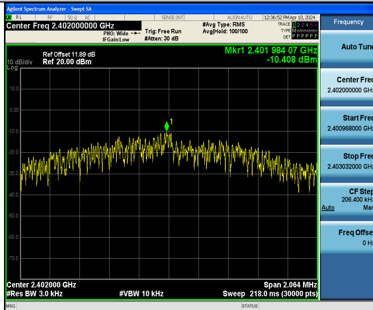
BLE_2M-Ant1-2402-PASS
