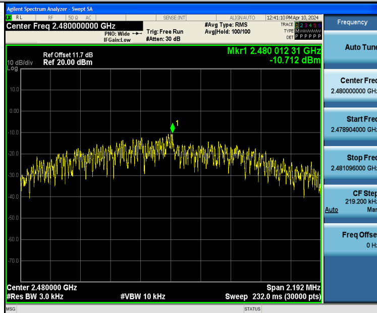
BLE_2M-Ant1-2480-PASS
