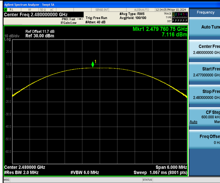
BLE_1M-Ant1-2480-PASS
