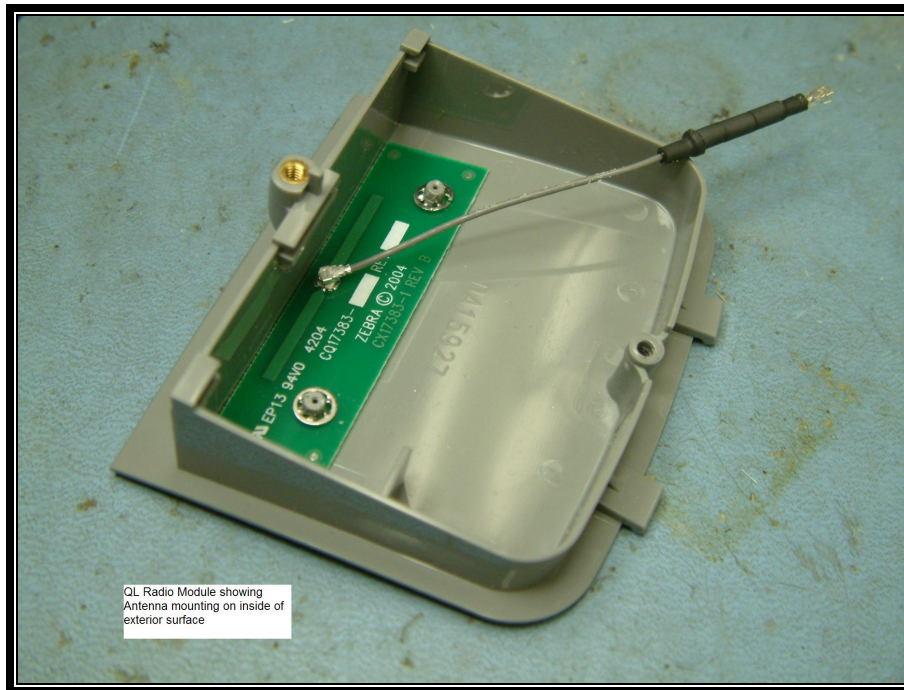
Photograph 1: QL radio module showing antenna mounting on inside of exterior surface
