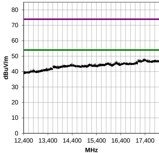
12400-18000 MHz, Run 21
