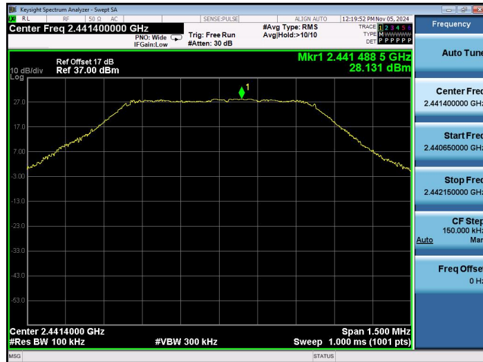
2.4G-Ant1-2441.4-0~Reference-PASS
