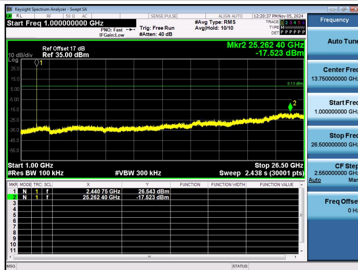
2.4G-Ant1-2441.4-1000~26500-PASS
