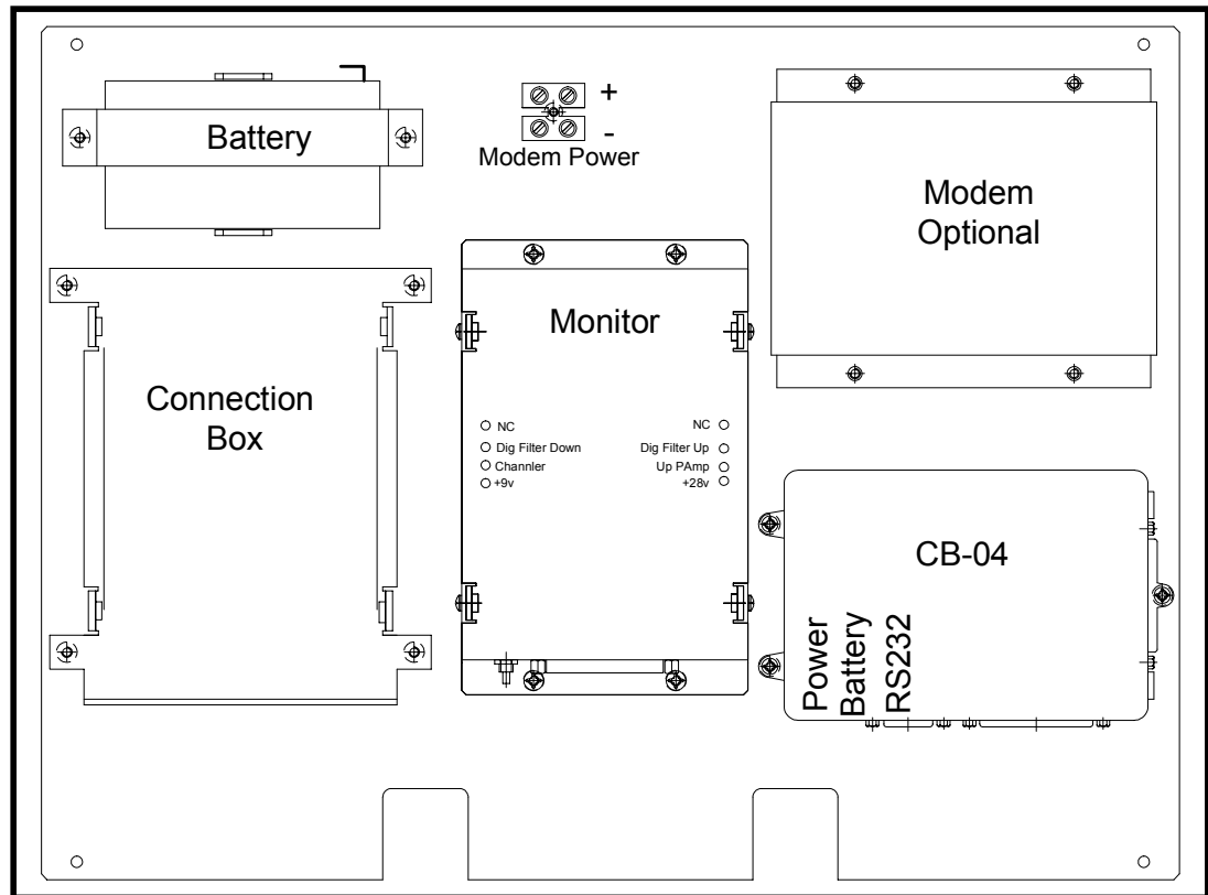
Figure 9: Digital Repeater Mechanical Outline - Cover
