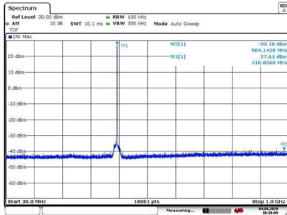
Figure 98: 30 – 1000 MHz
