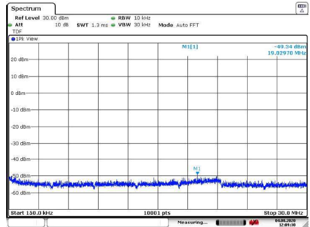
Figure 137: 150 kHz – 30 MHz
