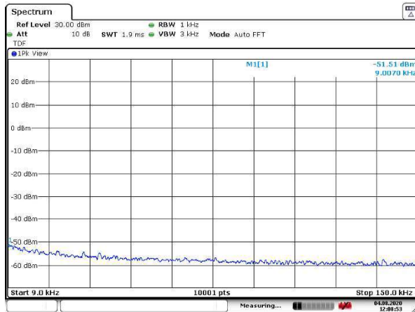
Figure 136: 9 – 150 kHz
