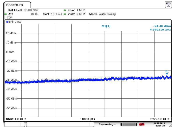
Figure 127: 1 – 5 GHz
