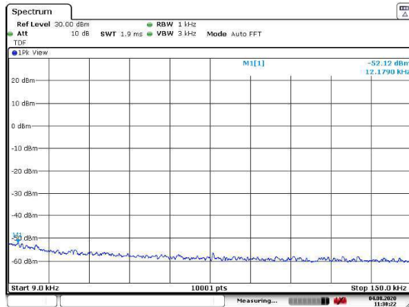
Figure 120: 9 – 150 kHz
