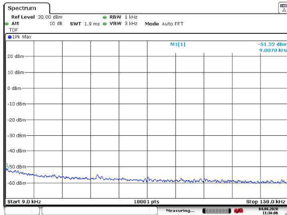
Figure 100: 9 – 150 kHz
