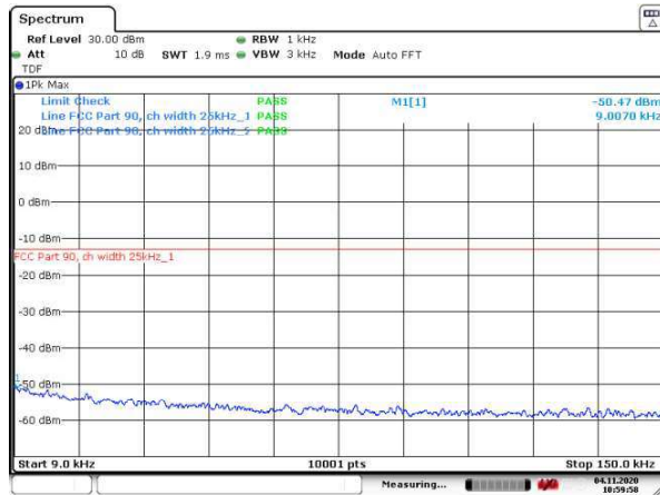
Figure 140: 9 – 150 kHz
