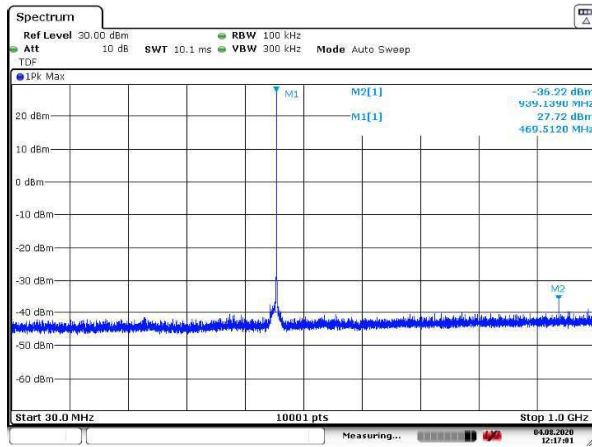
Figure 158: 30 – 1000 MHz
