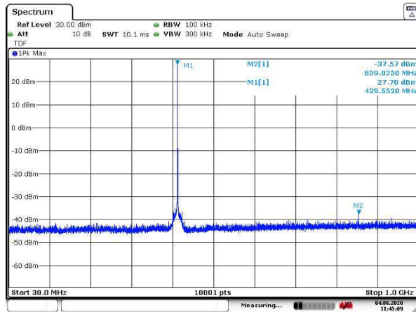
Figure 114: 30 – 1000 MHz
