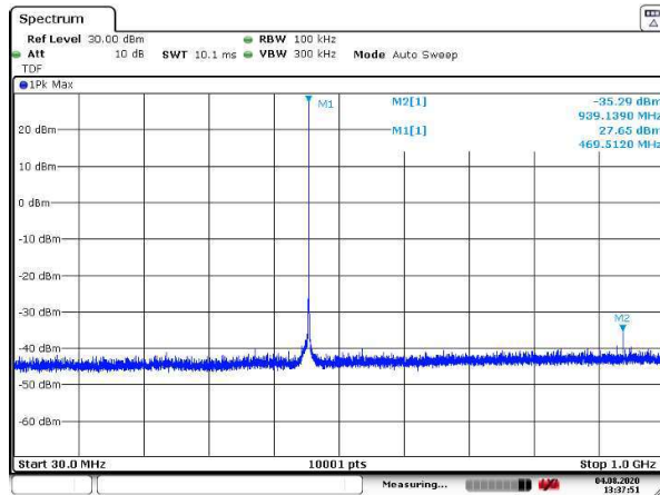
Figure 162: 30 – 1000 MHz
