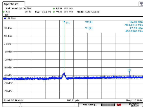
Figure 126: 30 – 1000 MHz
