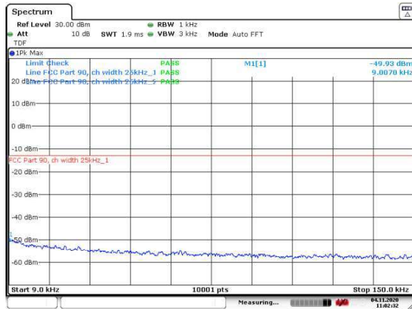
Figure 164: 9 – 150 kHz
