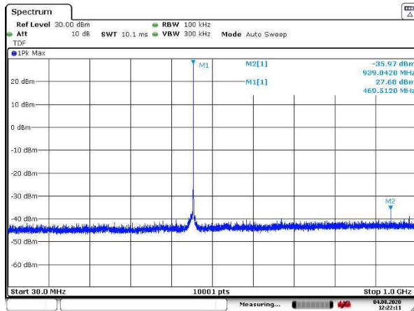
Figure 170: 30 – 1000 MHz
