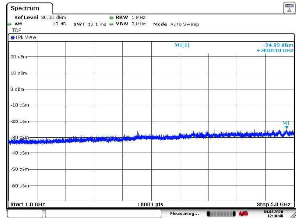
Figure 139: 1 – 5 GHz
