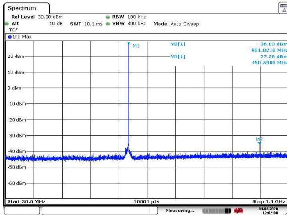
Figure 146: 30 – 1000 MHz
