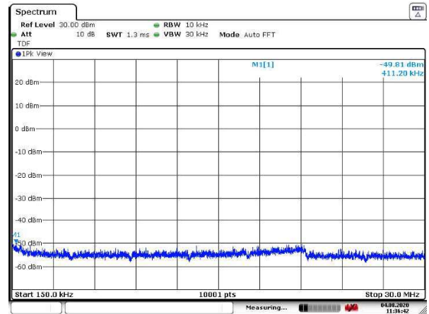
Figure 101: 150 kHz – 30 MHz
