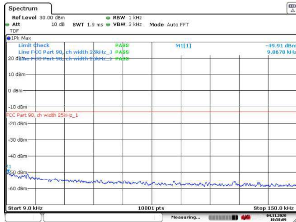
Figure 116: 9 – 150 kHz
