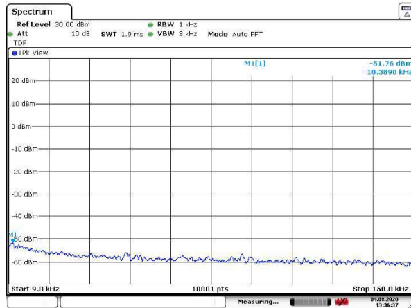
Figure 160: 9 – 150 kHz
