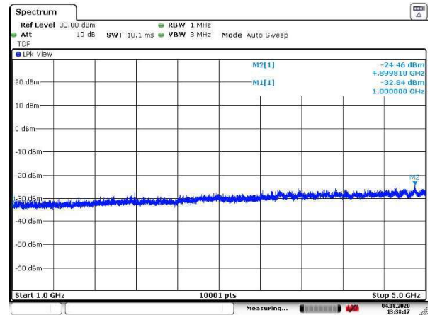
Figure 163: 1 – 5 GHz
