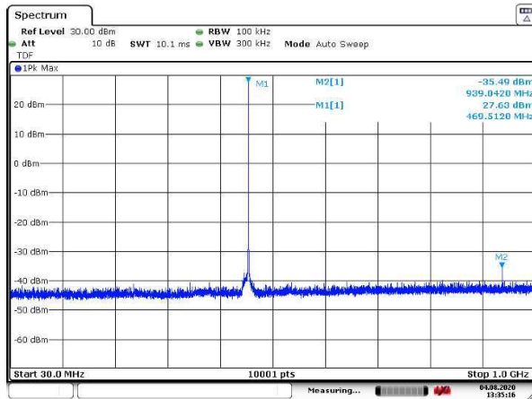
Figure 150: 30 – 1000 MHz
