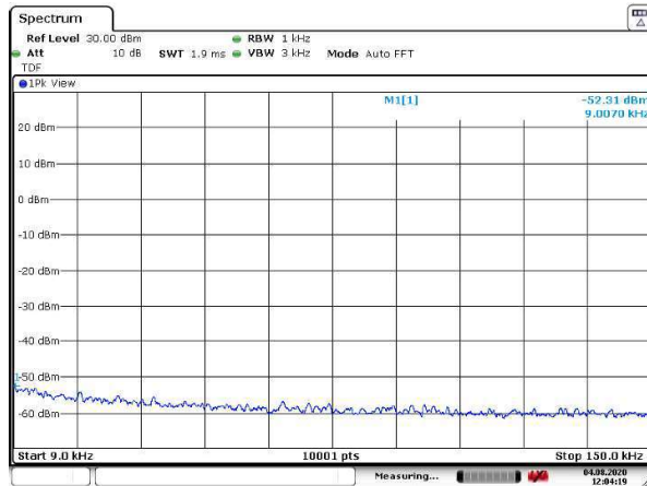
Figure 124: 9 – 150 kHz
