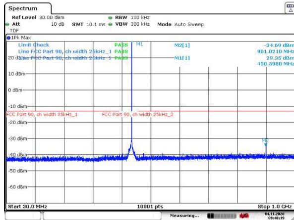
Figure 142: 30 – 1000 MHz
