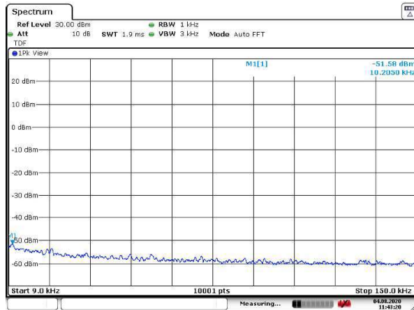
Figure 112: 9 – 150 kHz
