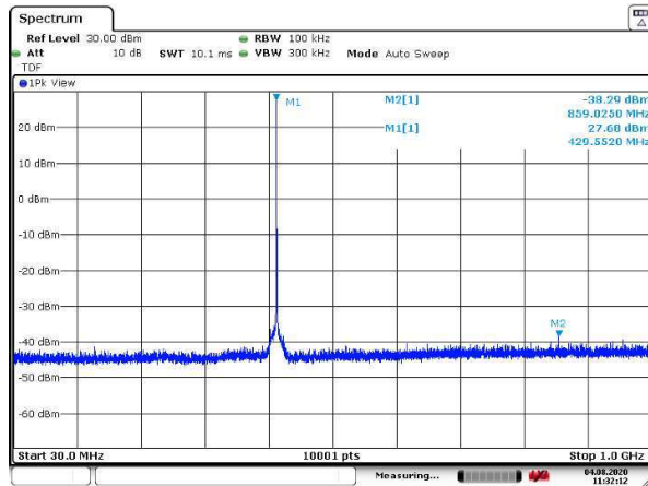
Figure 122: 30 – 1000 MHz
