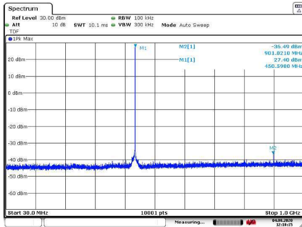
Figure 138: 30 – 1000 MHz
