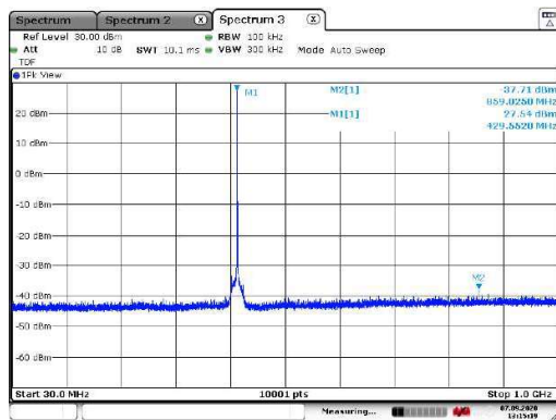
Figure 110: 30 – 1000 MHz
