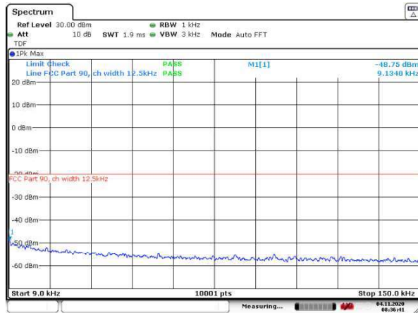
Figure 104: 9 – 150 kHz
