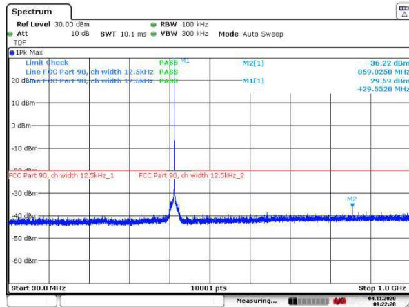
Figure 106: 30 – 1000 MHz
