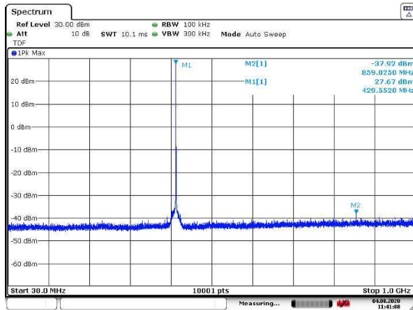
Figure 102: 30 – 1000 MHz
