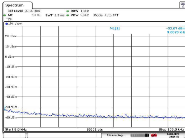
Figure 96: 9 – 150 kHz
