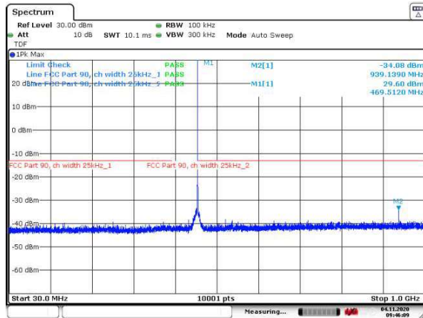
Figure 166: 30 – 1000 MHz
