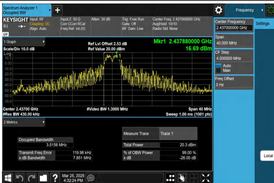
11AX20MIMO-Ant1-2437-52Tone-RU39
