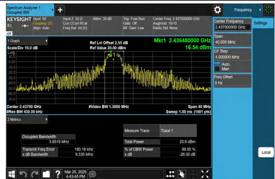
11AX20MIMO-Ant2-2437-52Tone-RU39
