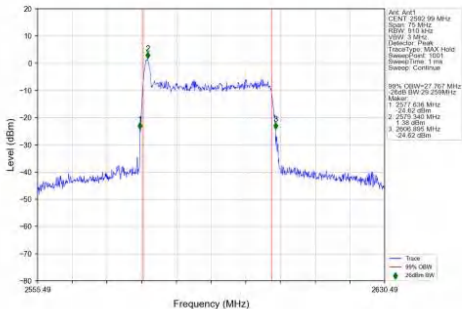
n41_30kHz_SISO_NTNV_30MHz_DFT-s-OFDM QPSK_2592.99MHz_Outer_Full_Ant1
