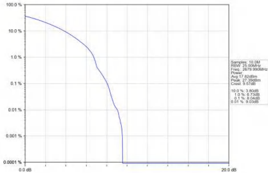
n41_30kHz_SISO_NTNV_20MHz_CP-OFDM_256_QAM_2679.99MHz_Outer_Full_Ant1
