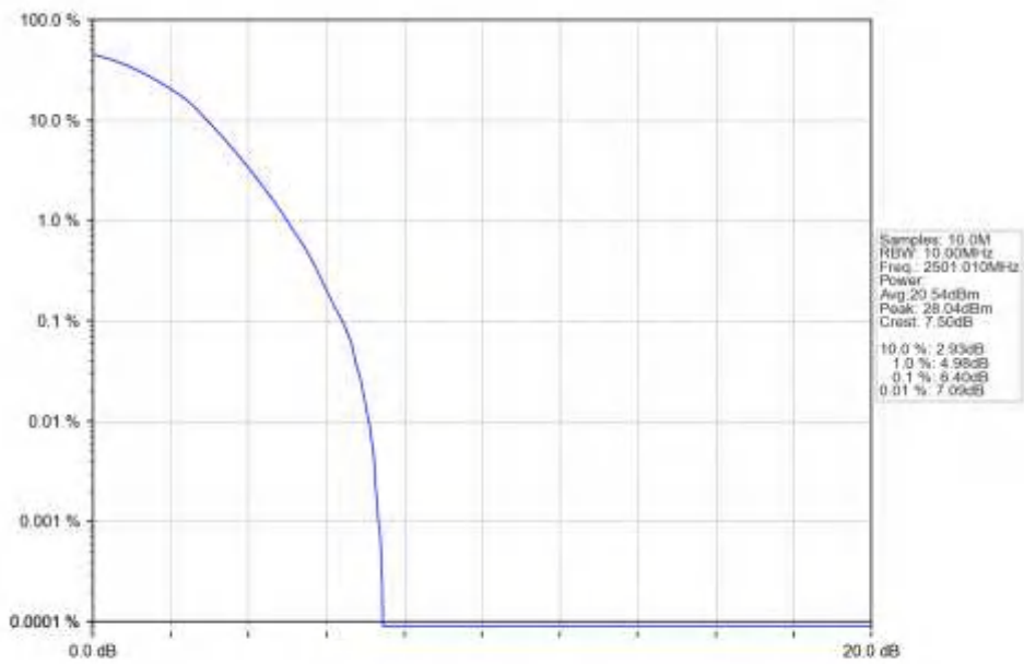
n41_30kHz_SISO_NTNV_10MHz_DFT-s-OFDM_64_QAM_2501.01MHz_Outer_Full_Ant1
