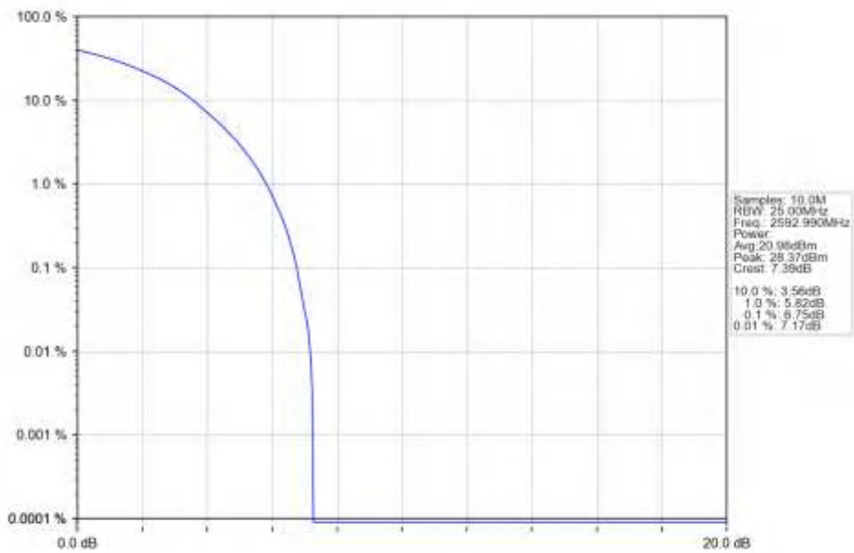
n41_30kHz_SISO_NTNV_15MHz_CP-OFDM_64_QAM_2592.99MHz_Outer_Full_Ant1
