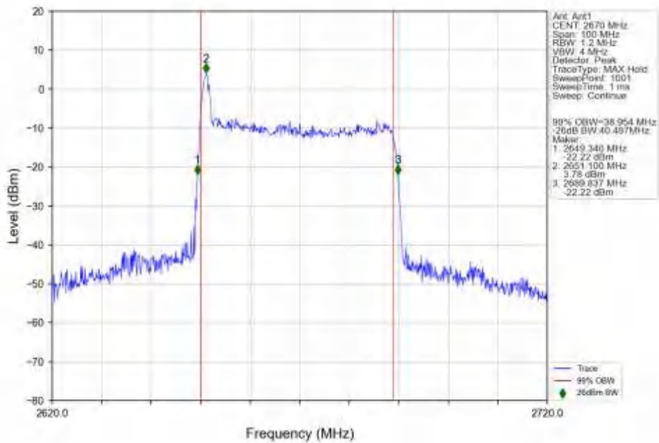
n41_30kHz_SISO_NTNV_40MHz_CP-OFDM_256_QAM_2670MHz_Outer_Full_Ant1
