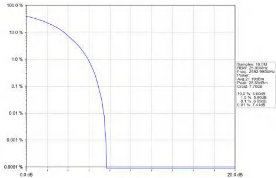
n41_30kHz_SISO_NTNV_20MHz_CP-OFDM_64_QAM_2592.99MHz_Outer_Full_Ant1
