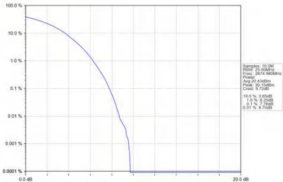
n41_30kHz_SISO_NTNV_30MHz_CP-OFDM_64_QAM_2674.98MHz_Outer_Full_Ant1
