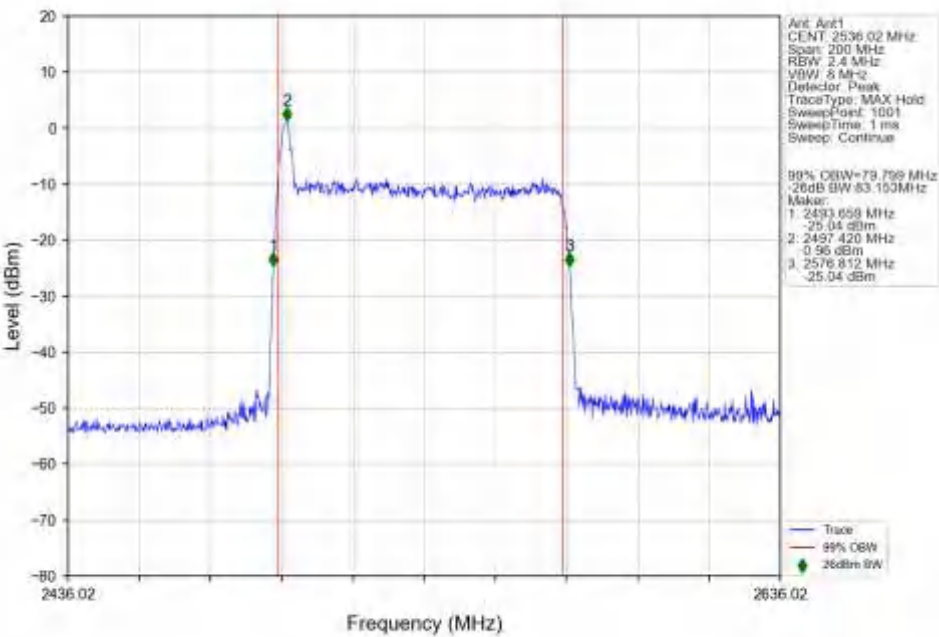
n41_30kHz_SISO_NTNV_80MHz_CP-OFDM_256_QAM_2536.02MHz_Outer_Full_Ant1
