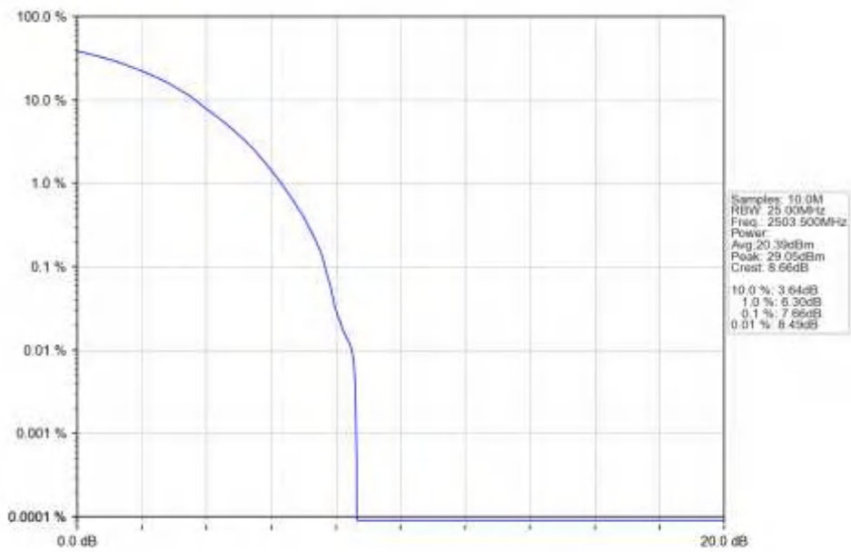
n41_30kHz_SISO_NTNV_15MHz_CP-OFDM_64_QAM_2503.5MHz_Outer_Full_Ant1
