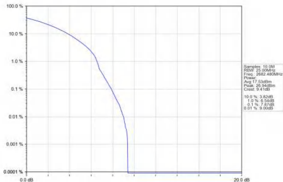
n41_30kHz_SISO_NTNV_15MHz_CP-OFDM_256_QAM_2682.48MHz_Outer_Full_Ant1
