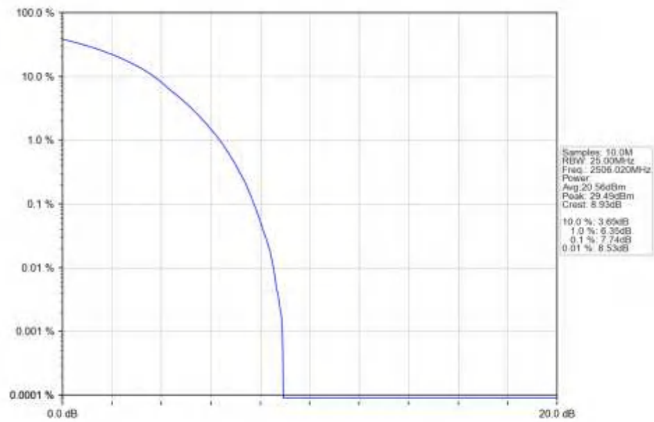
n41_30kHz_SISO_NTNV_20MHz_CP-OFDM_64_QAM_2506.02MHz_Outer_Full_Ant1
