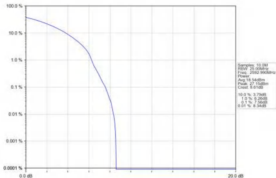
n41_30kHz_SISO_NTNV_15MHz_CP-OFDM_256_QAM_2592.99MHz_Outer_Full_Ant1
