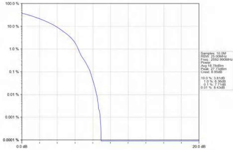
n41_30kHz_SISO_NTNV_20MHz_CP-OFDM_256_QAM_2592.99MHz_Outer_Full_Ant1
