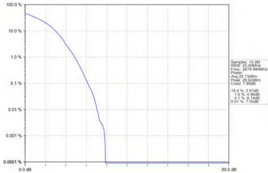
n41_30kHz_SISO_NTNV_20MHz_DFT-s-OFDM_64_QAM_2679.99MHz_Outer_Full_Ant1
