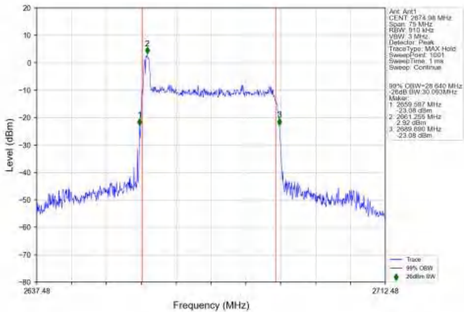
n41_30kHz_SISO_NTNV_30MHz_CP-OFDM_256_QAM_2674.98MHz_Outer_Full_Ant1
