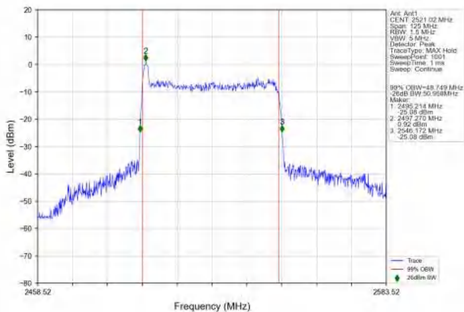
n41_30kHz_SISO_NTNV_50MHz_CP-OFDM_16_QAM_2521.02MHz_Outer_Full_Ant1
