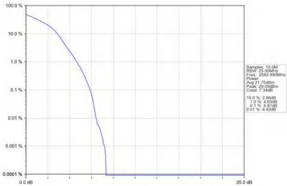
n41_30kHz_SISO_NTNV_20MHz_DFT-s-OFDM_16_QAM_2592.99MHz_Outer_Full_Ant1
