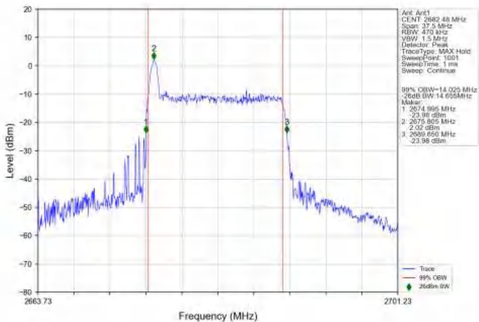
n41_30kHz_SISO_NTNV_15MHz_CP-OFDM_256_QAM_2682.48MHz_Outer_Full_Ant1
