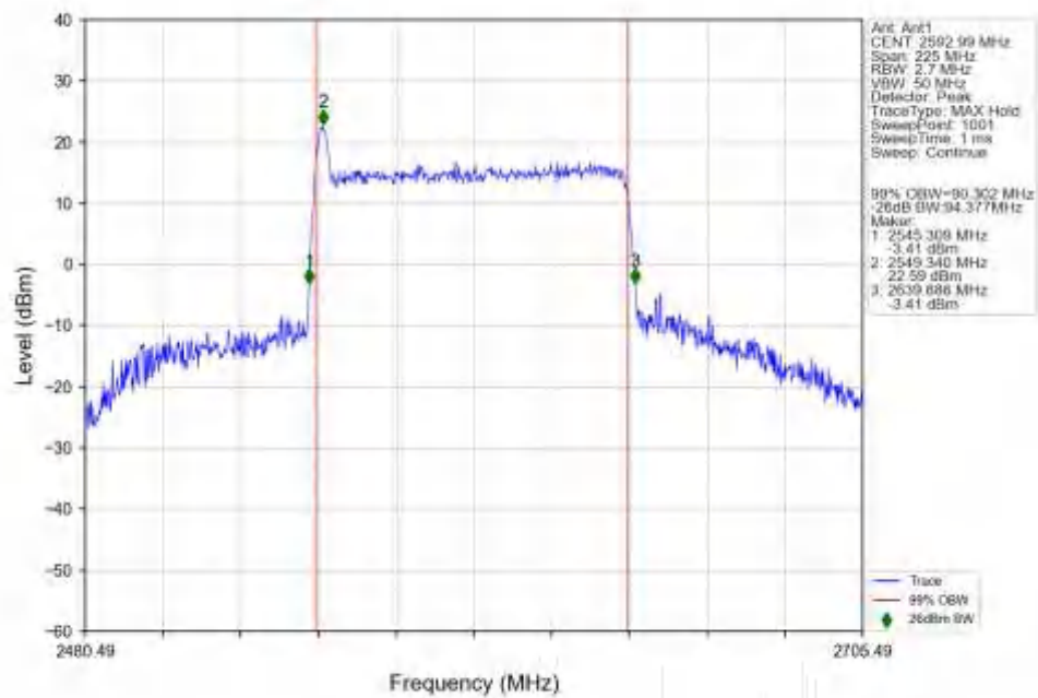
n41_30kHz_SISO_NTNV_90MHz_CP-OFDM_QPSK_2592.99MHz_Outer_Full_Ant1
