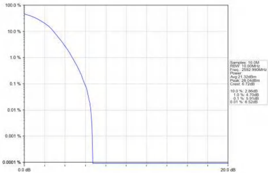
n41_30kHz_SISO_NTNV_10MHz_DFT-s-OFDM_64_QAM_2592.99MHz_Outer_Full_Ant1
