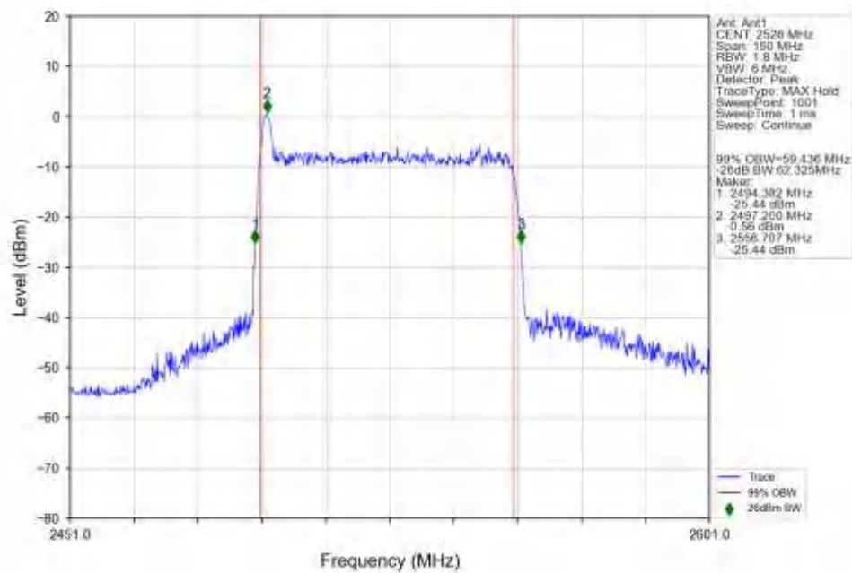
n41_30kHz_SISO_NTNV_60MHz_CP-OFDM_16_QAM_2526MHz_Outer_Full_Ant1
