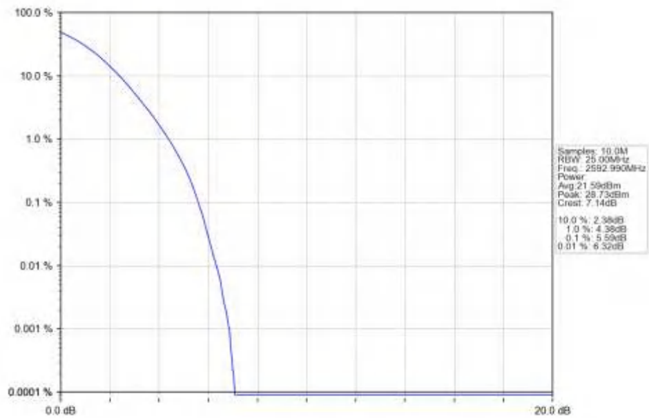
n41_30kHz_SISO_NTNV_30MHz_DFT-s-OFDM QPSK_2592.99MHz_Outer_Full_Ant1
