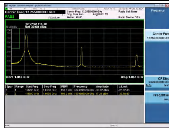
Band25-15MHz-16QAM-26115-1RB#0-PASS
