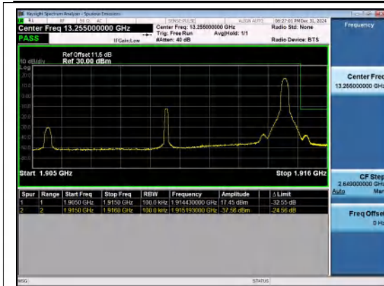
Band25-10MHz-16QAM-26640-1RB#49-PASS
