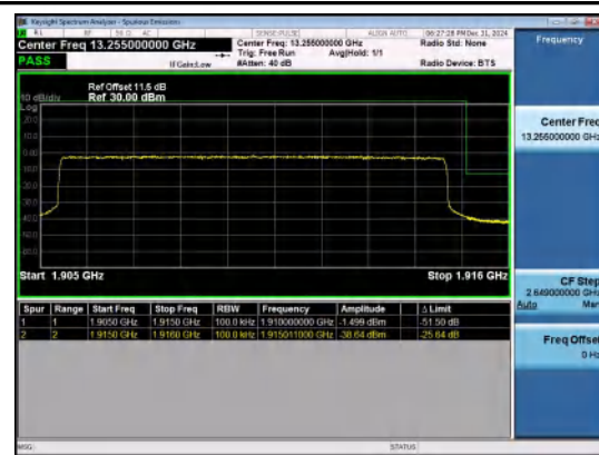
Band25-10MHz-16QAM-26640-50RB#0-PASS
