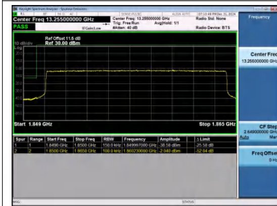
Band25-15MHz-QPSK-26115-75RB#0-PASS
