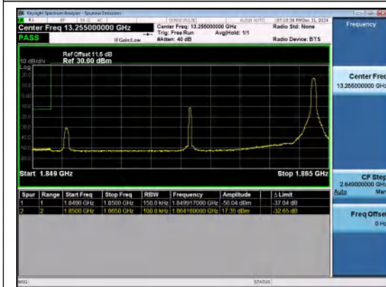
Band25-15MHz-16QAM-26115-1RB#74-PASS
