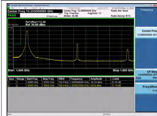
Band25-15MHz-QPSK-26115-1RB#0-PASS
