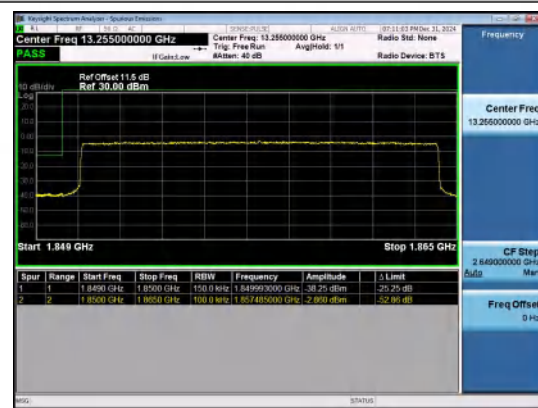
Band25-15MHz-16QAM-26115-75RB#0-PASS
