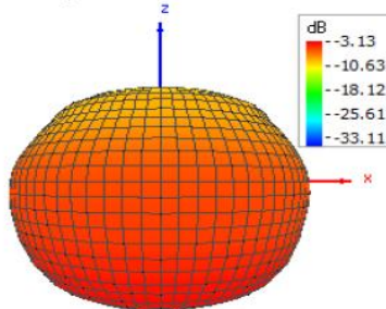
Theta = 90, Phi = 270
