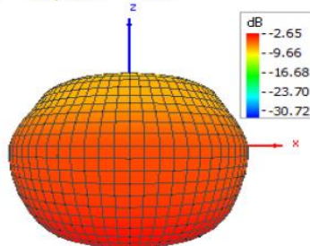
Theta = 90, Phi = 270
