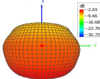
Theta = 90, Phi = 0
