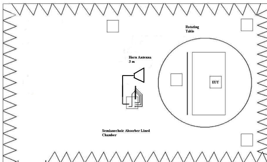
Setup for measurements > 1GHz.
