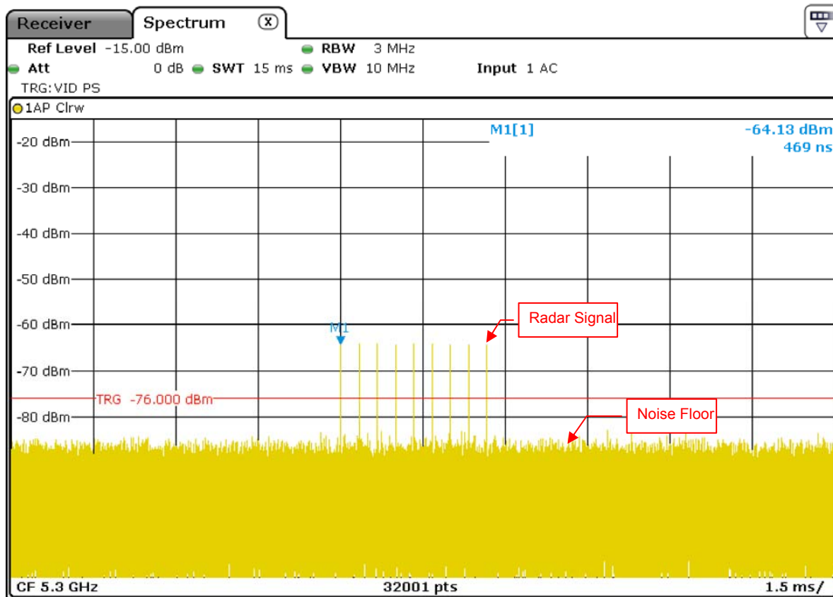
Radar Signal 6
