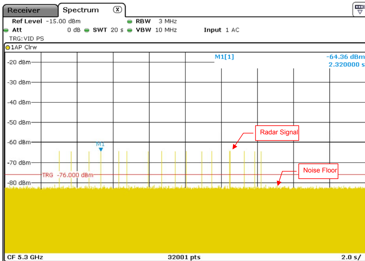
Radar Signal 5
