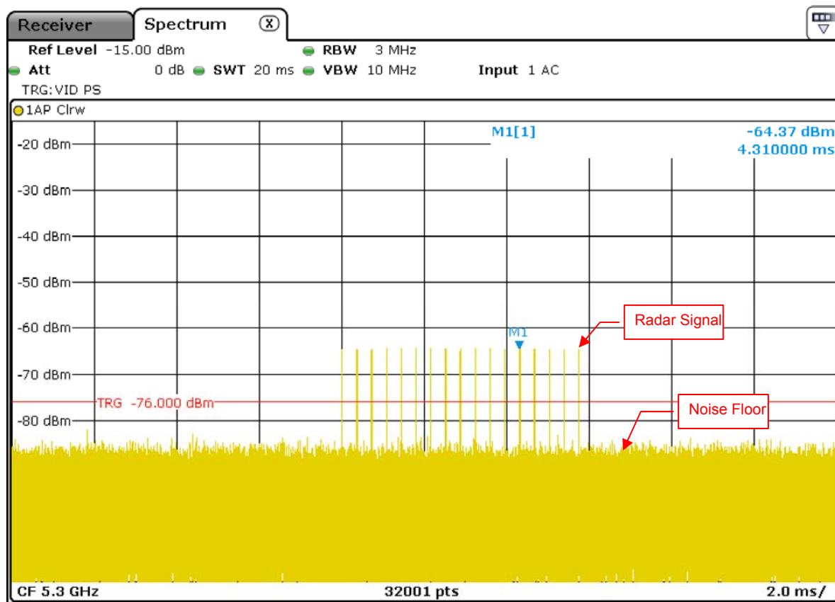
Radar Signal 3
