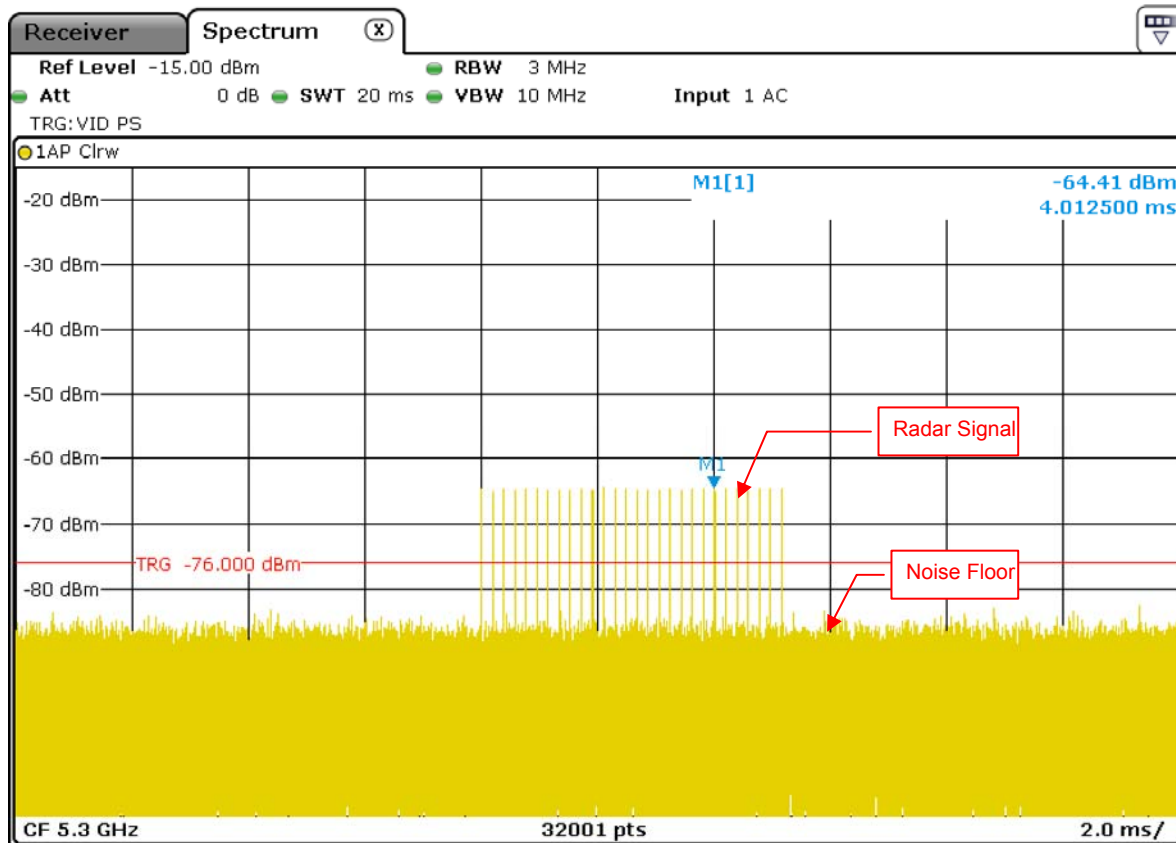
Radar Signal 2
