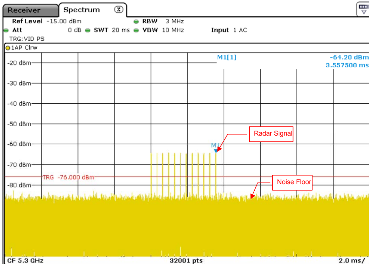
Radar Signal 4
