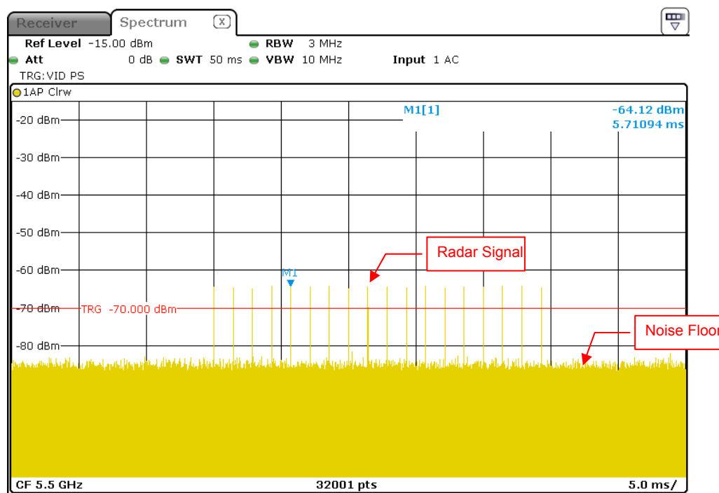
Radar Signal 0
