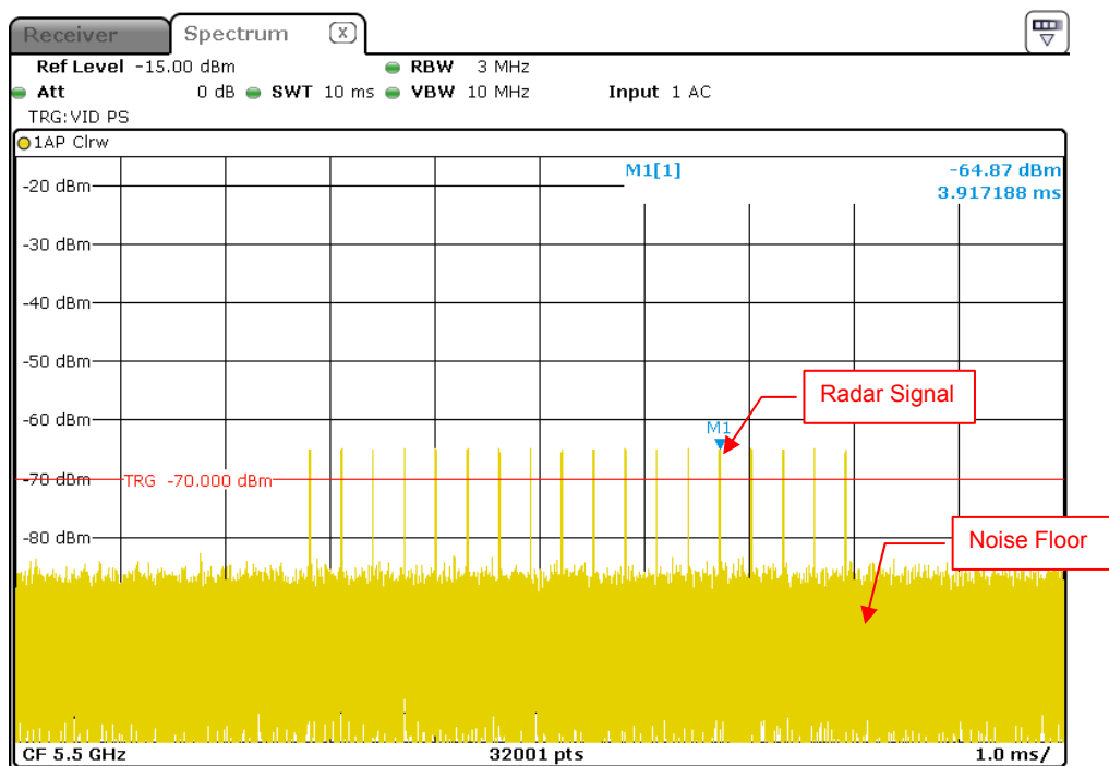
Radar Signal 3
