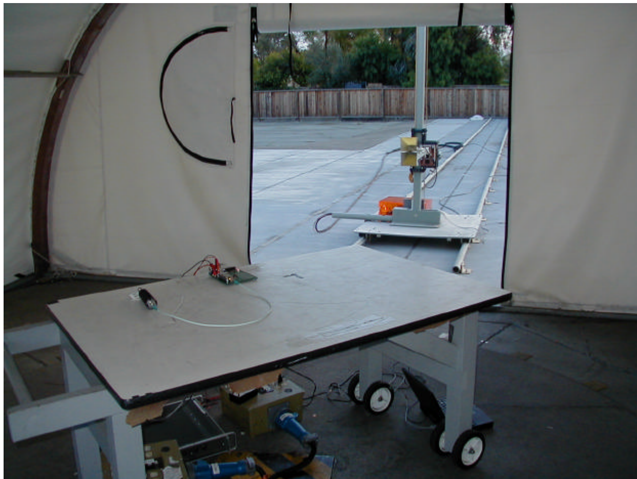
Setup Photo# 1
