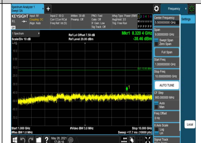
Band17-5MHz-QPSK-23790-1RB#0-Range2:1000~100
