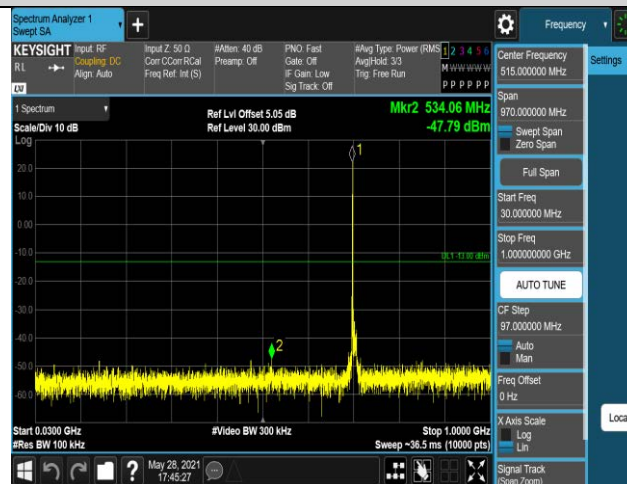
Band17-10MHz-16QAM-23800-1RB#0-Range1:30~
