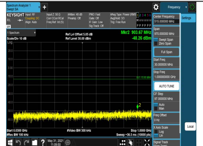
Band13-5MHz-16QAM-23205-1RB#0-Range1:30~100
