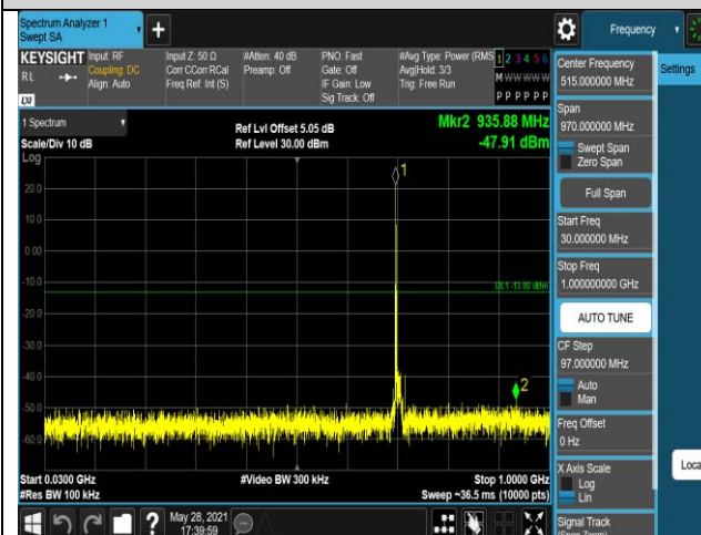
Band17-10MHz-QPSK-23800-1RB#0-Range1:30~1
