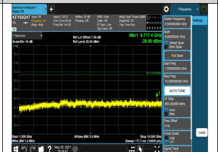
Band12-10MHz-16QAM-23095-1RB#0-Range2:1000~1
