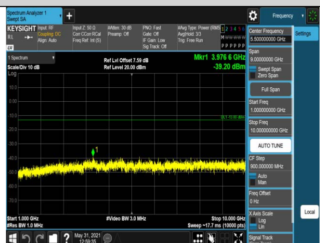
Band13-10MHz-QPSK-23230-1RB#0-Range2:1000~10000MHz
