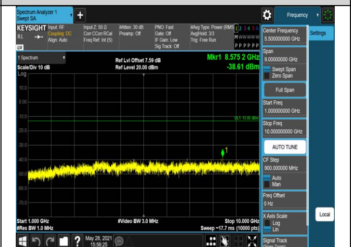
Band12-1.4MHz-16QAM-23095-1RB#0-Range2:1000~1
