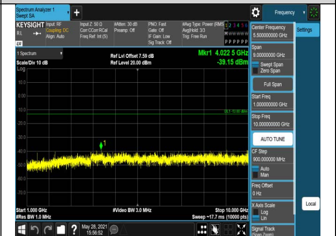
Band12-1.4MHz-16QAM-23017-1RB#0-Range2:1000~1
