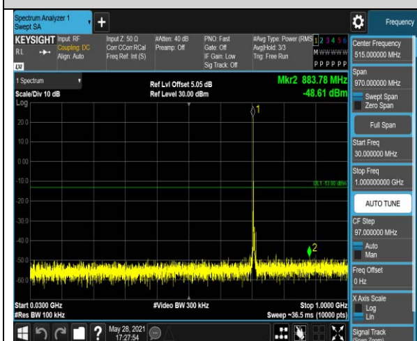
Band17-5MHz-QPSK-23825-1RB#0-Range1:30~10
