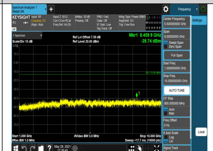
Band17-5MHz-16QAM-23790-1RB#0-Range2:1000~10
