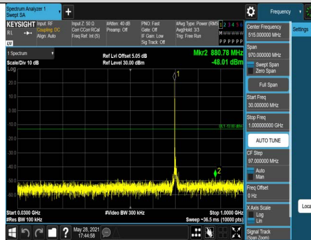
Band17-10MHz-16QAM-23790-1RB#0-Range1:30~
