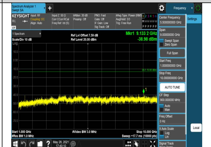
Band17-10MHz-QPSK-23800-1RB#0-Range2:1000~10
