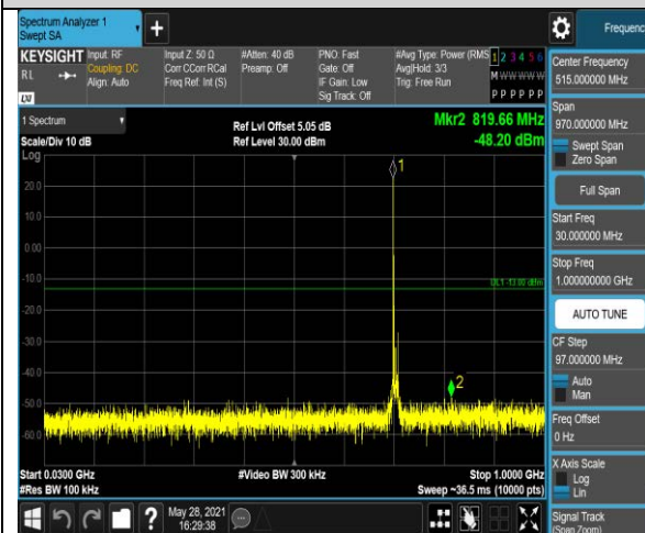
Band12-10MHz-16QAM-23060-1RB#0-Range1:30~1
