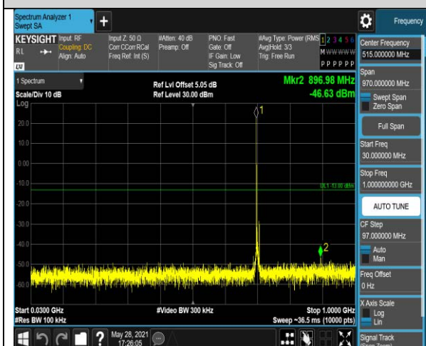
Band17-5MHz-QPSK-23790-1RB#0-Range1:30~10
