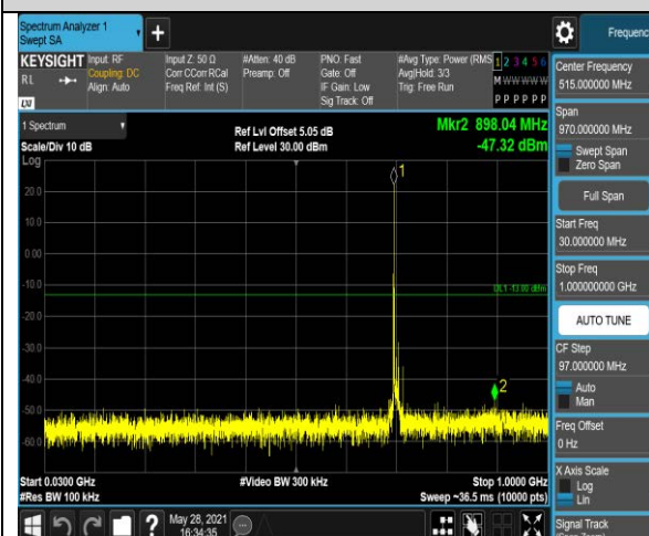
Band12-10MHz-16QAM-23095-1RB#0-Range1:30~1
