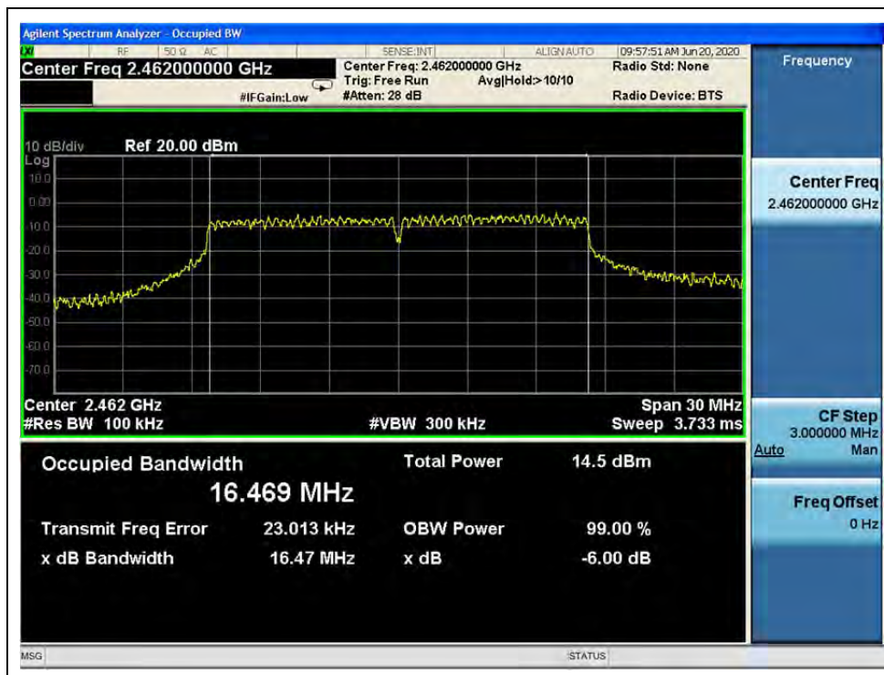
(Channel 11, 802.11g)
