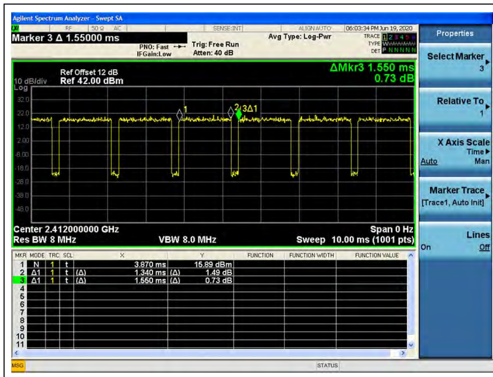
(Channel 1, 802.11g)
