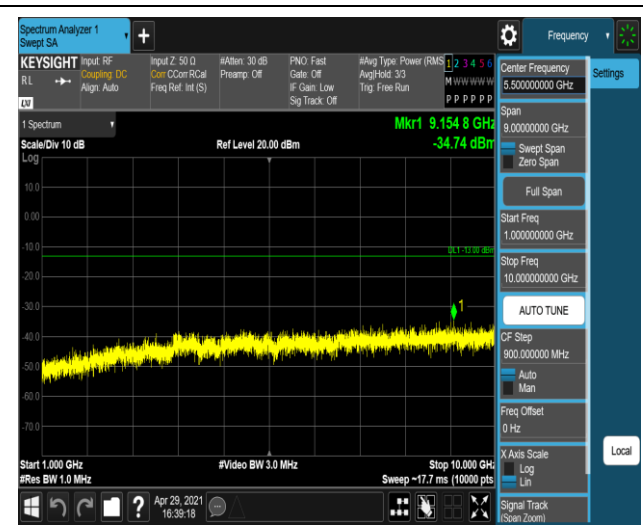
Band17-5MHz-QPSK-23755-1RB#0-Range2:1000~100
