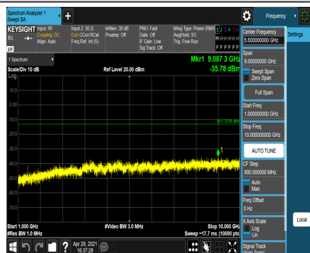
Band12-10MHz-16QAM-23095-1RB#0-Range2:1000~1 0000MHz
