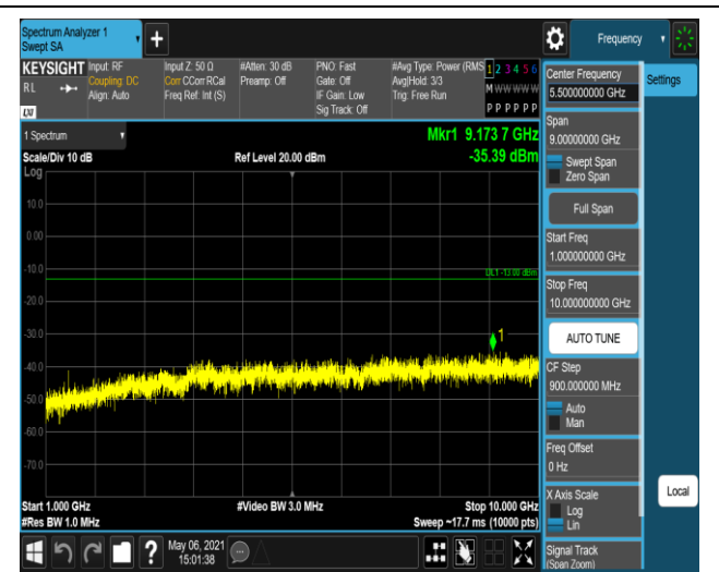
Band17-10MHz-16QAM-23790-1RB#0-Range2:1000~10000MHz
