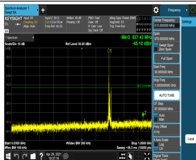
Band12-10MHz-16QAM-23095-1RB#0-Range1:30~ 1000MHz
