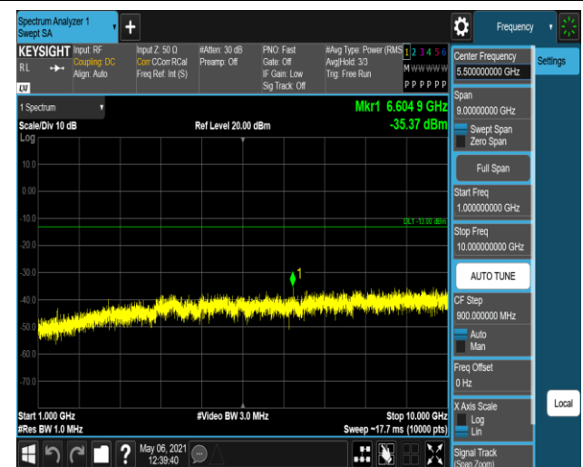
Band17-10MHz-QPSK-23780-1RB#0-Range2:1000~10
