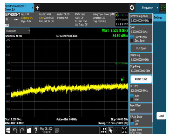
Band17-10MHz-16QAM-23800-1RB#0-Range2:1000~10000MHz
