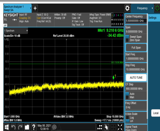
Band17-5MHz-16QAM-23755-1RB#0-Range2:1000~10
