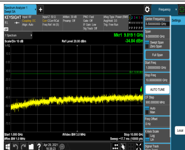
Band12-10MHz-16QAM-23130-1RB#0-Range2:1000~1 0000MHz
