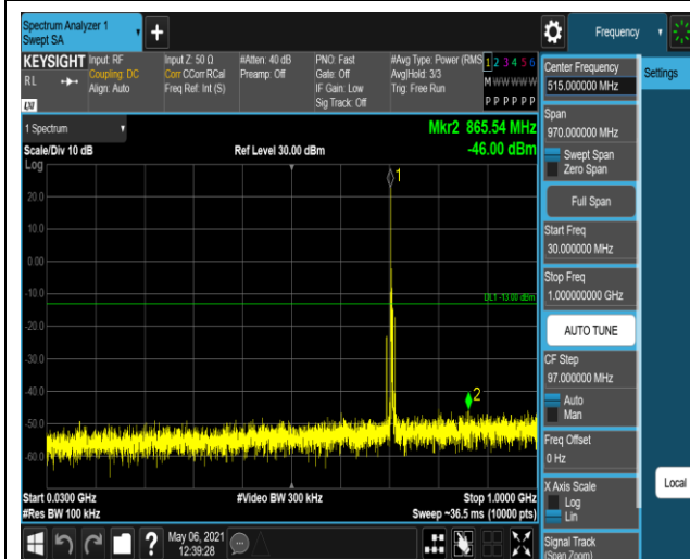
Band17-10MHz-QPSK-23780-1RB#0-Range1:30~1
