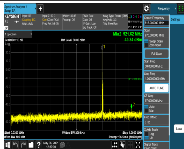
Band17-5MHz-16QAM-23790-1RB#0-Range1:30~1
