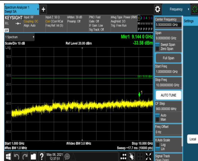
Band17-5MHz-16QAM-23790-1RB#0-Range2:1000~10
