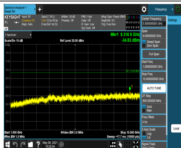
Band17-10MHz-QPSK-23800-1RB#0-Range2:1000~10
