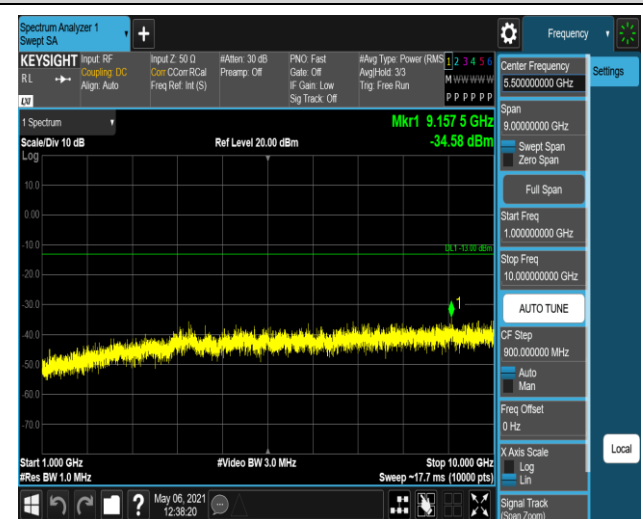
Band17-5MHz-QPSK-23790-1RB#0-Range2:1000~100
