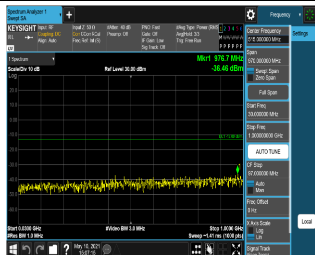
Band66-20MHz-QPSK-132322-1RB#0-Range1:30~
