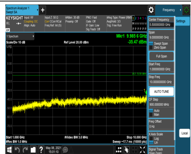
Band17-10MHz-QPSK-23780-1RB#0-Range2:1000~10
