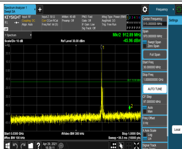
Band12-10MHz-16QAM-23130-1RB#0-Range1:30~ 1000MHz
