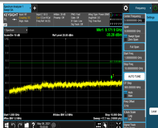
Band17-10MHz-16QAM-23780-1RB#0-Range2:1000~1
