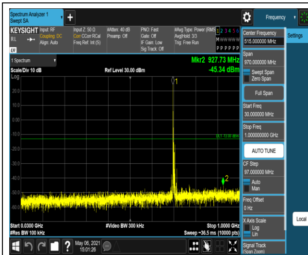
Band17-10MHz-16QAM-23790-1RB#0-Range1:30~1000MHz
