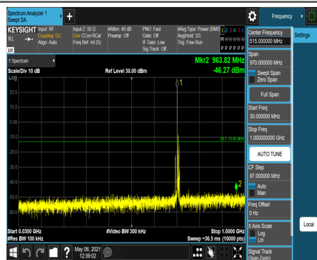
Band17-5MHz-16QAM-23755-1RB#0-Range1:30~1
