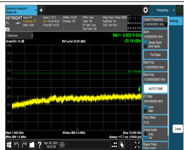
Band12-10MHz-QPSK-23095-1RB#0-Range2:1000~10
