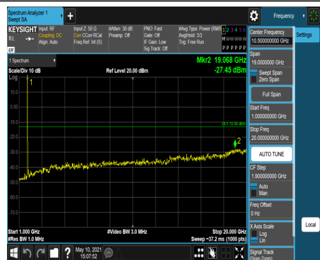
Band66-20MHz-16QAM-132072-1RB#0-Range2:1000~20000MHz
