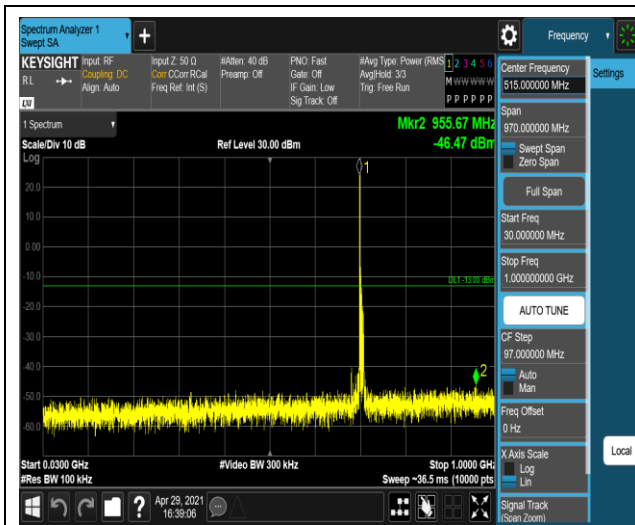
Band17-5MHz-QPSK-23755-1RB#0-Range1:30~10
