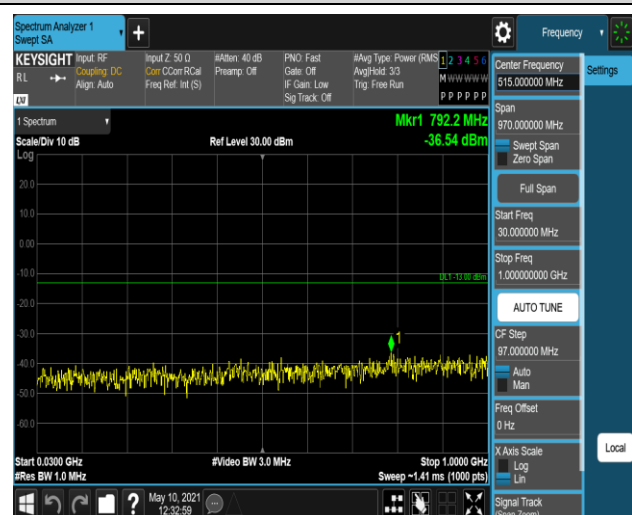
Band66-1.4MHz-QPSK-132665-1RB#0-Range1:30~ 1000MHz
