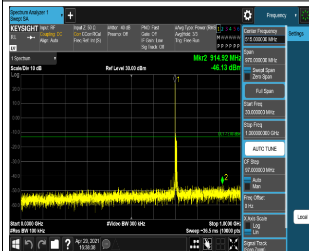
Band12-10MHz-QPSK-23130-1RB#0-Range1:30~1
