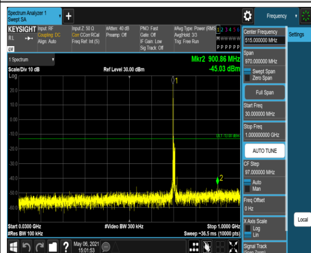
Band17-10MHz-QPSK-23800-1RB#0-Range1:30~1
