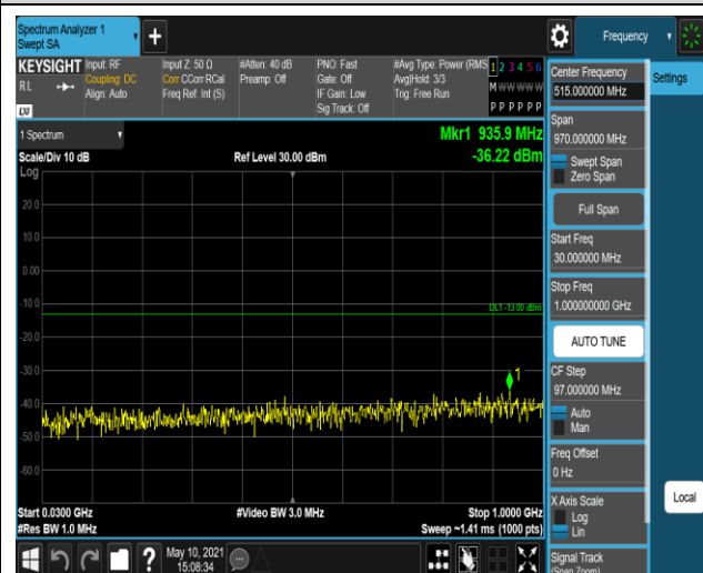
Band66-20MHz-16QAM-132572-1RB#0-Range1:30 ~1000MHz
