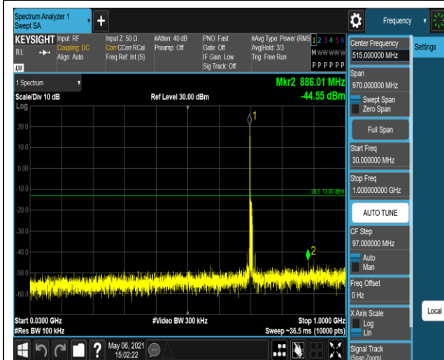
Band17-10MHz-16QAM-23800-1RB#0-Range1:30~1000MHz
