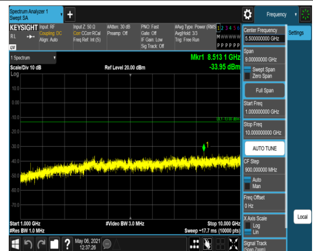
Band17-5MHz-QPSK-23790-1RB#0-Range2:1000~100
