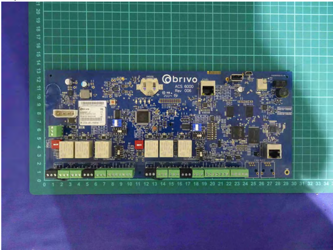
(178) EUT Photo – M/N: B-ACS6100R, B-ACS6100R-A, B-ACS6100R-E, B-ACS6100R-S
