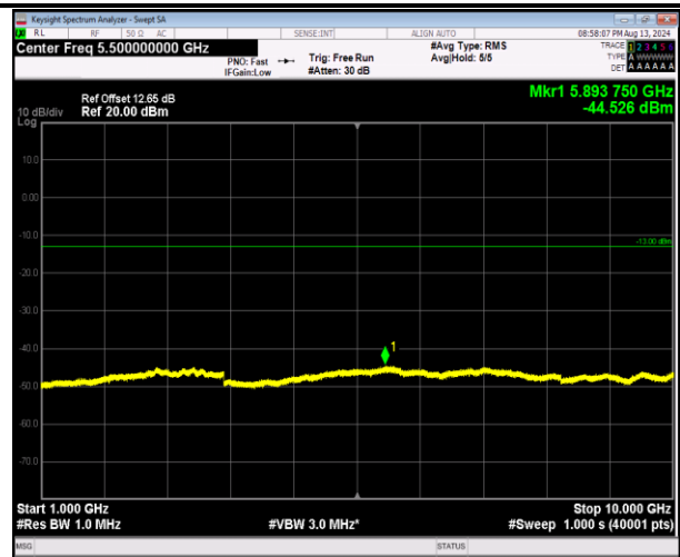
5-5-MHz-3MHz-QPSK-QPSK-20510-20549-1RB#0-0RB#0 -1000~10000MHz-PASS
