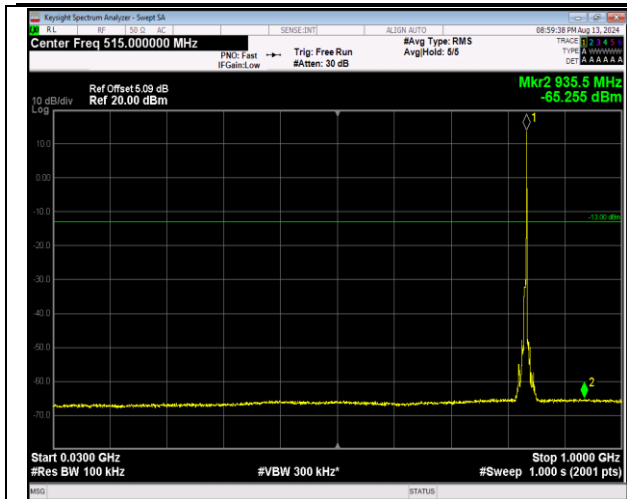
5-5-5MHz-3MHz-16QAM-16QAM-20510-20549-1RB#24-0RB#0-30~1000MHz-PASS
