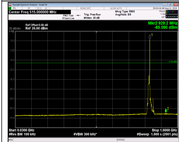
5-5-10MHz-10MHz-QPSK-QPSK-20450-20549-1RB#49-49 ORB#0-30~1000MHz-PASS
