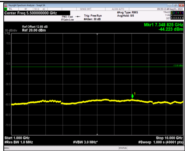
5-5-5MHz-3MHz-64QAM-64QAM-20595-20634-1RB#0-1RB #15-1000~10000MHz-PASS
