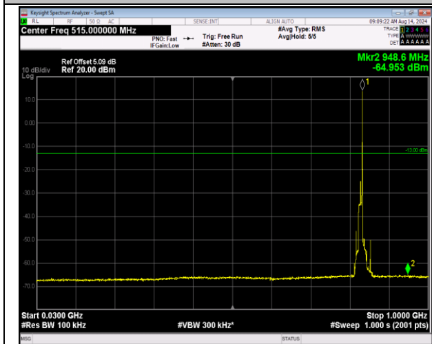
5-5-10MHz-10MHz-QPSK-QPSK-20476-20575-1RB#49-49 ORB#0-30~1000MHz-PASS
