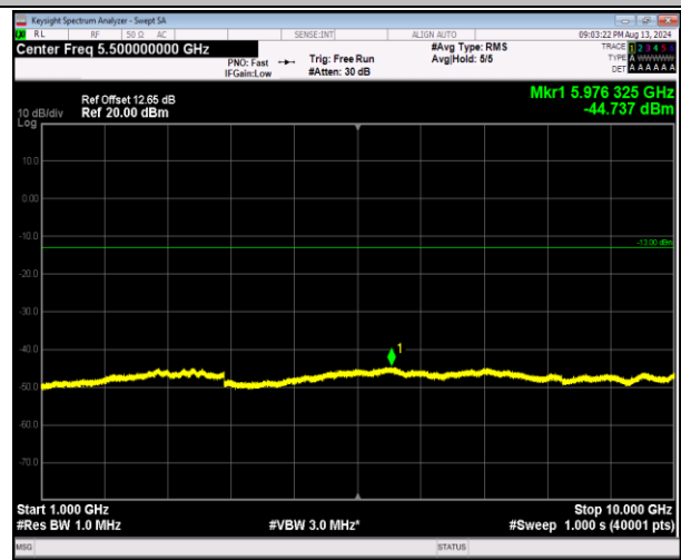
5-5-5MHz-3MHz-16QAM-16QAM-20595-20634-1RB#0-0RB #0-1000~10000MHz-PASS
