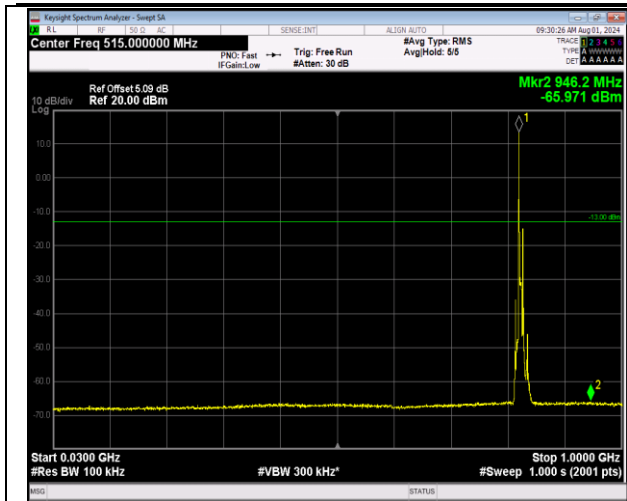
5-5-5MHz-3MHz-64QAM-64QAM-20425-20464-1RB#0-1 RB#15-30~1000MHz-PASS
