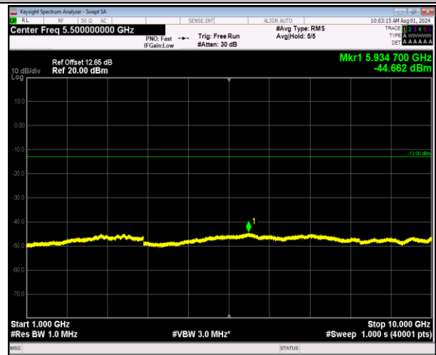
5-5-10MHz-10MHz-64QAM-64QAM-20476-20575-1RB#0-0 RB#0-1000~10000MHz-PASS
