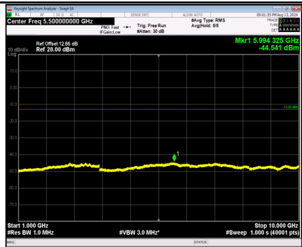
5-5-5MHz-3MHz-QPSK-QPSK-20510-20549-25RB#0-15RB #0-1000~10000MHz-PASS
