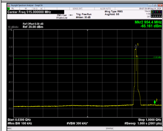
5-5-10MHz-10MHz-16QAM-16QAM-20450-20549-50RB#- 0-50RB#0-30~1000MHz-PASS
