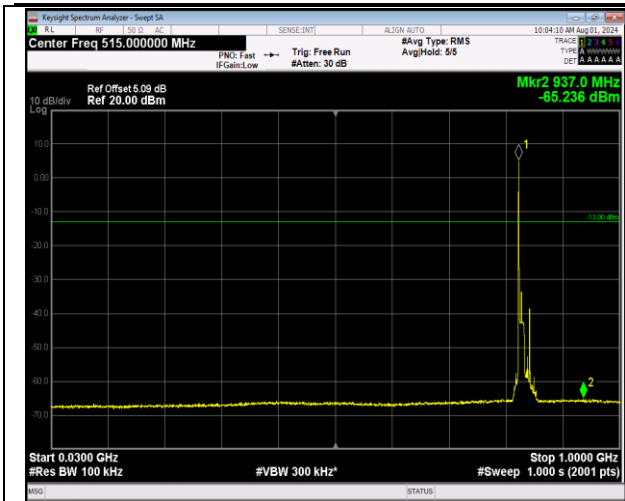
5-5-10MHz-10MHz-64QAM-64QAM-20476-20575-1RB#0 -1RB#49-30~1000MHz-PASS
