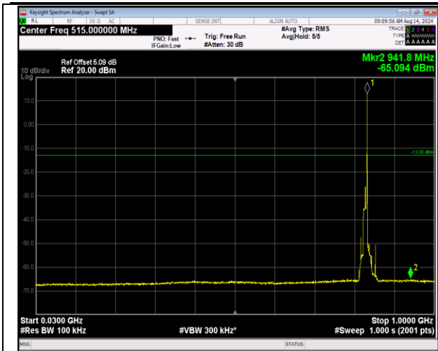
5-5-10MHz-10MHz-16QAM-16QAM-20476-20575-1RB#4 9-0RB#0-30~1000MHz-PASS
