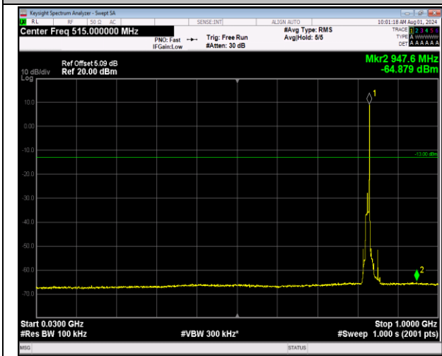
5-5-10MHz-10MHz-64QAM-64QAM-20450-20549-1RB#4 9-0RB#0-30~1000MHz-PASS
