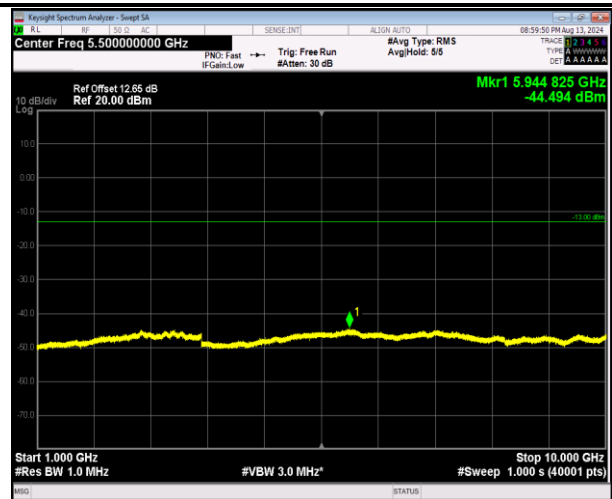
5-5-5MHz-3MHz-16QAM-16QAM-20510-20549-1RB#24-0RB#0-1000~10000MHz-PASS
