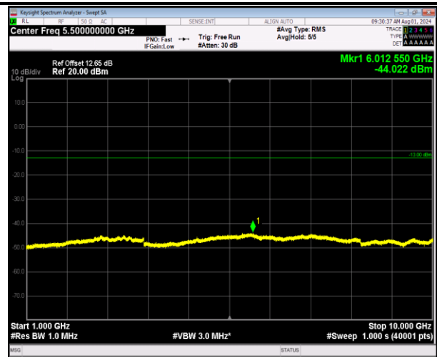
5-5-5MHz-3MHz-64QAM-64QAM-20425-20464-1RB#0-1RB #15-1000~10000MHz-PASS
