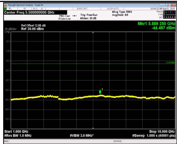
5-5-10MHz-10MHz-64QAM-64QAM-20476-20575-1RB#0-1 RB#49-1000~10000MHz-PASS
