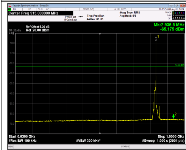
5-5-10MHz-10MHz-64QAM-64QAM-20476-20575-1RB#4 9-0RB#0-30~1000MHz-PASS
