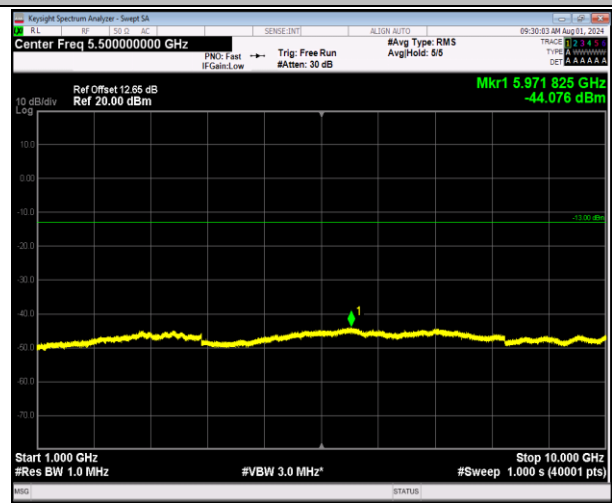
5-5-5MHz-3MHz-64QAM-64QAM-20425-20464-1RB#24-0R B#0-1000~10000MHz-PASS
