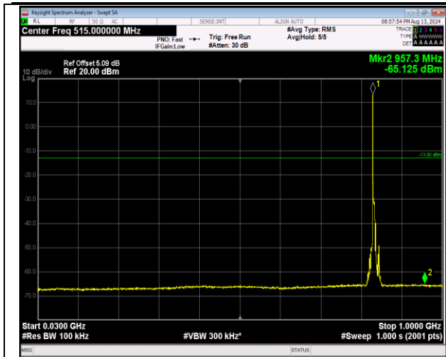
5-5-MHz-3MHz-QPSK-QPSK-20510-20549-1RB#0-0RB #0-30~1000MHz-PASS
