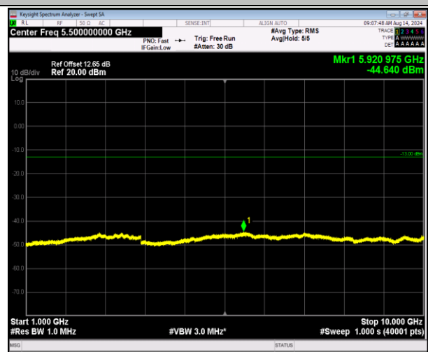
5-5-10MHz-10MHz-16QAM-16QAM-20450-20549-50RB#0- 50RB#0-1000~10000MHz-PASS
