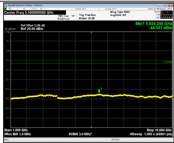
5-5-10MHz-10MHz-64QAM-64QAM-20450-20549-1RB#49- 0RB#0-1000~10000MHz-PASS
