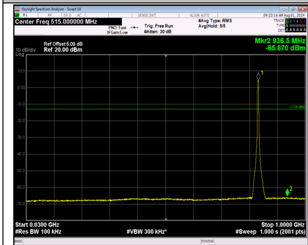
5-5-5MHz-3MHz-64QAM-64QAM-20510-20549-25RB#0-0- 15RB#0-30~1000MHz-PASS
