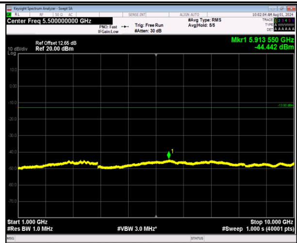
5-5-10MHz-10MHz-64QAM-64QAM-20450-20549-1RB#0-1 RB#49-1000~10000MHz-PASS
