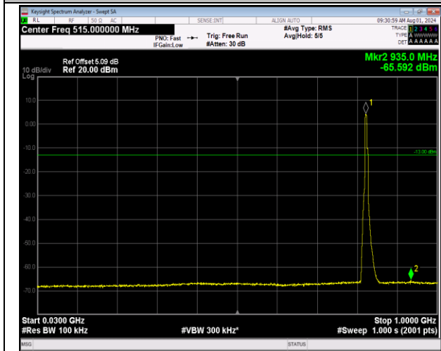
5-5-5MHz-3MHz-64QAM-64QAM-20425-20464-25RB#0-0- 15RB#0-30~1000MHz-PASS
