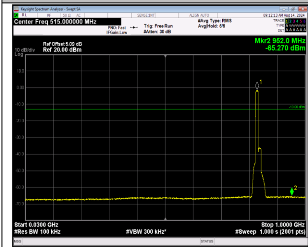
5-5-10MHz-10MHz-16QAM-16QAM-20476-20575-50RB#- 0-50RB#0-30~1000MHz-PASS
