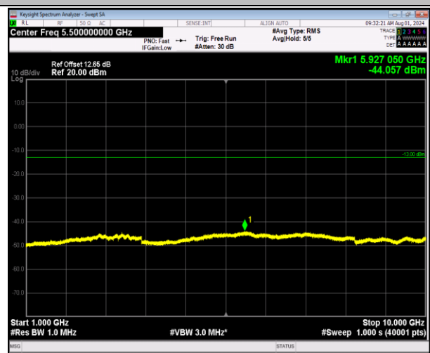
5-5-5MHz-3MHz-64QAM-64QAM-20510-20549-1RB#24-0R B#0-1000~10000MHz-PASS
