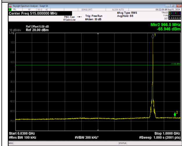
5-5-5MHz-3MHz-64QAM-64QAM-20510-20549-1RB#24- 0RB#0-30~1000MHz-PASS
