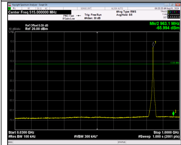
5-5-5MHz-3MHz-64QAM-64QAM-20595-20634-25RB#0-0 15RB#0-30~1000MHz-PASS
