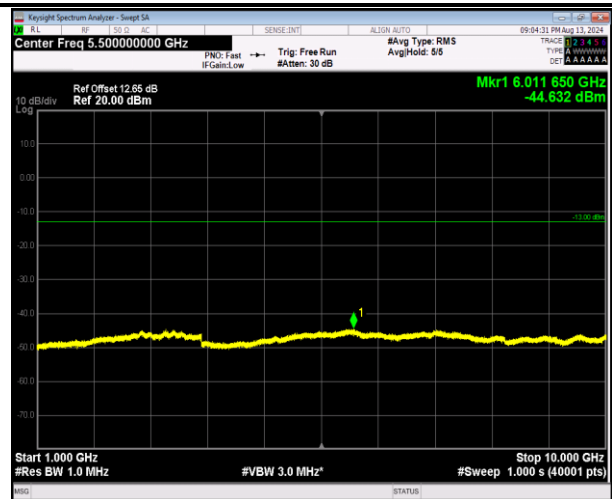
5-5-5MHz-3MHz-16QAM-16QAM-20595-20634-1RB#24-0RB#0-1000~10000MHz-PASS
