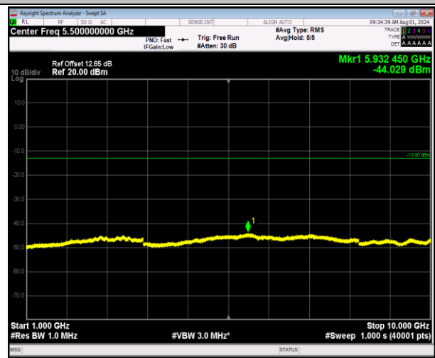
5-5-5MHz-3MHz-64QAM-64QAM-20595-20634-1RB#24-0R B#0-1000~10000MHz-PASS
