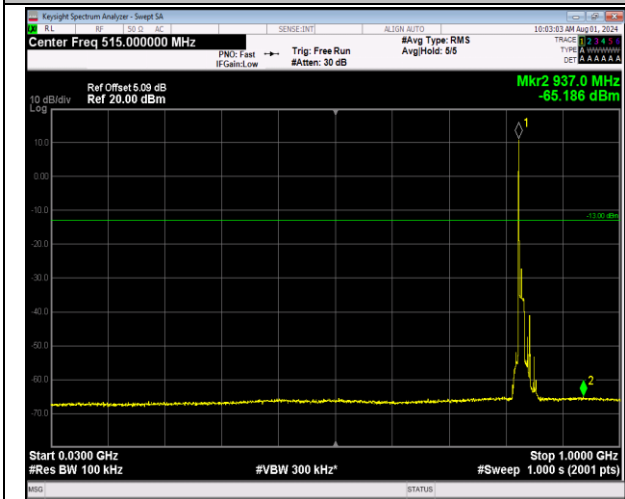
5-5-10MHz-10MHz-64QAM-64QAM-20476-20575-1RB#0 -0RB#0-30~1000MHz-PASS
