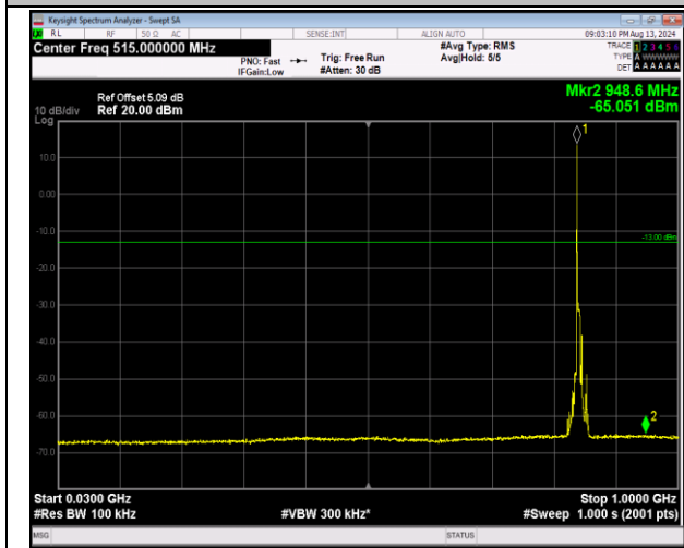
5-5-5MHz-3MHz-16QAM-16QAM-20595-20634-1RB#0-0 RB#0-30~1000MHz-PASS
