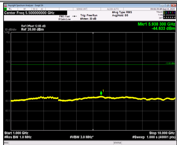
5-5-10MHz-10MHz-16QAM-16QAM-20450-20549-1RB#0-1RB#49-1000~10000MHz-PASS
