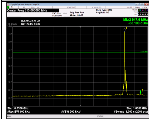
5-5-MHz-3MHz-QPSK-QPSK-20510-20549-1RB#0-1RB #15-30~1000MHz-PASS
