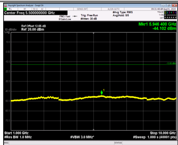
5-5-5MHz-3MHz-64QAM-64QAM-20510-20549-1RB#0-0RB#0-1000~10000MHz-PASS
