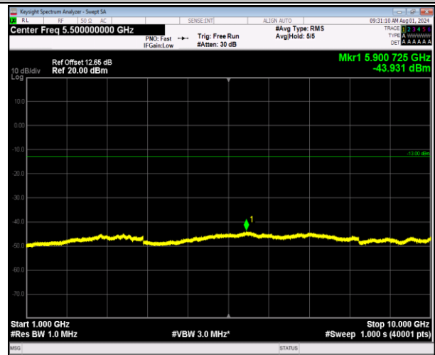
5-5-5MHz-3MHz-64QAM-64QAM-20425-20464-25RB#0-15 RB#0-1000~10000MHz-PASS
