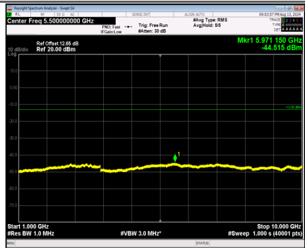
5-5-5MHz-3MHz-QPSK-QPSK-20595-20634-1RB#24-0RB# 0-1000~10000MHz-PASS
