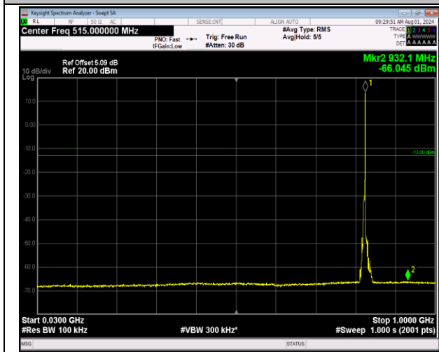
5-5-5MHz-3MHz-64QAM-64QAM-20425-20464-1RB#24- 0RB#0-30~1000MHz-PASS
