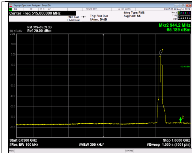
5-5-10MHz-10MHz-QPSK-QPSK-20450-20549-50RB#0-50RB#0-30~1000MHz-PASS
