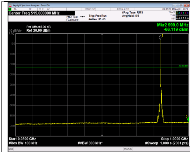
5-5-5MHz-3MHz-64QAM-64QAM-20595-20634-1RB#0-1 RB#15-30~1000MHz-PASS
