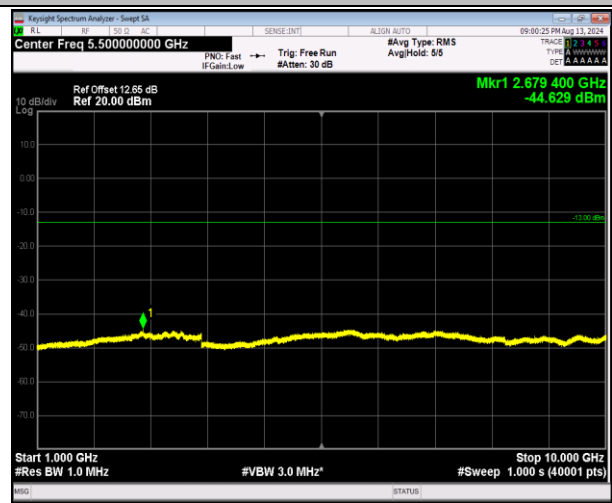
5-5-MHz-3MHz-QPSK-QPSK-20510-20549-1RB#0-1RB#1 5-1000~10000MHz-PASS
