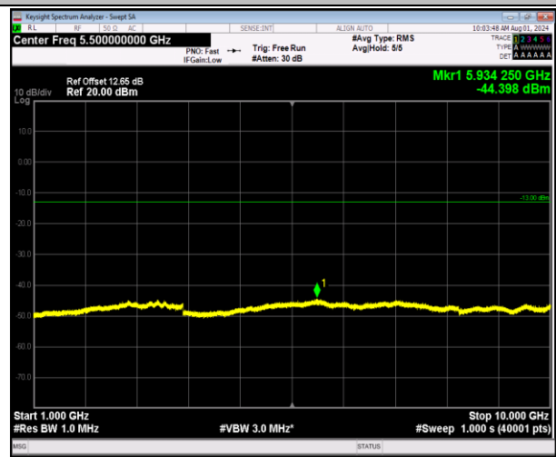
5-5-10MHz-10MHz-64QAM-64QAM-20476-20575-1RB#49- 0RB#0-1000~10000MHz-PASS
