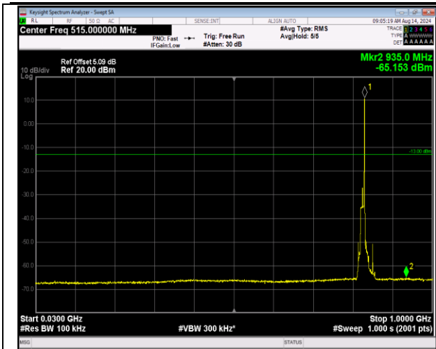
5-5-10MHz-10MHz-16QAM-16QAM-20450-20549-1RB#4 9-0RB#0-30~1000MHz-PASS
