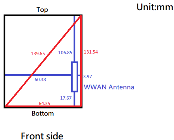
Fig.18 Antenna position of EUT (WWAN)
