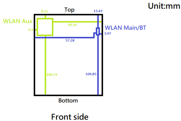
Fig.17 Antenna position of EUT (WLAN)
