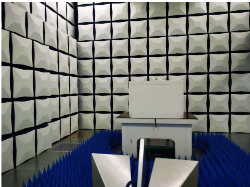
Photograph 2: Set-up for Radiated Emission, above 1GHz
