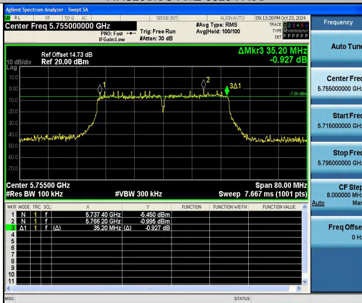
11AC40SISO-Ant2-5755-PASS
