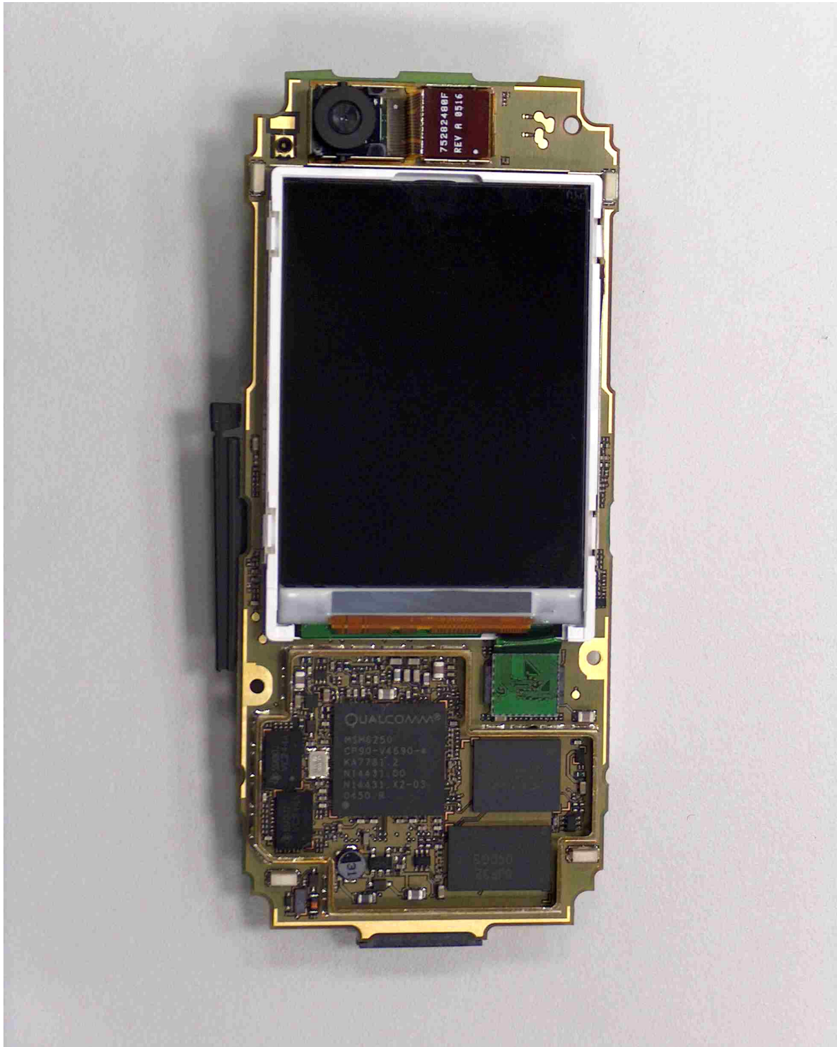
Figure 6 SXG75 PCB Front View Shields Removed
