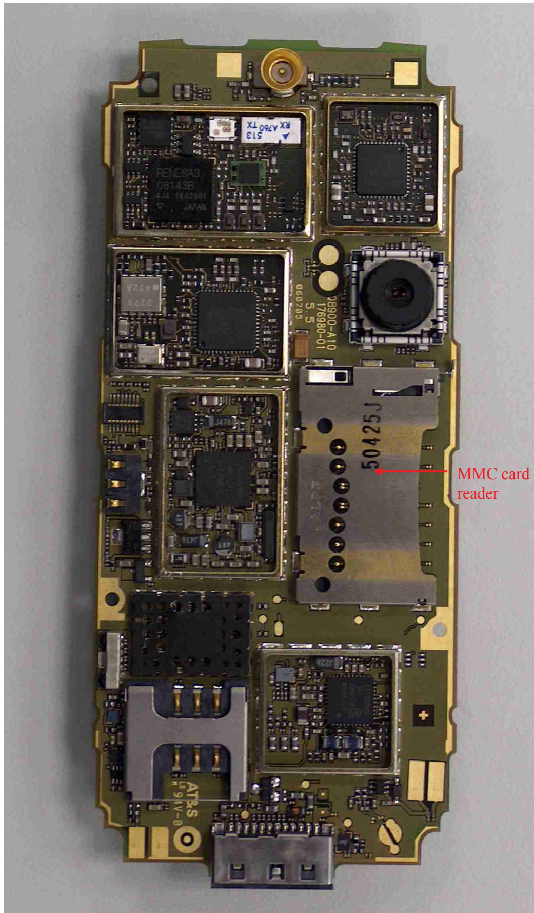
Figure 7 SXG75 PCB Back View Shields Removed
