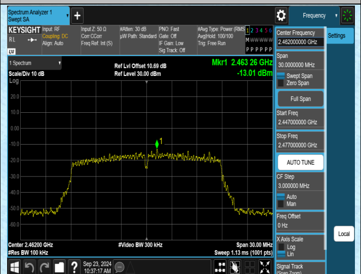
11N20MIMO-Ant2-2462-0~Reference-PASS
