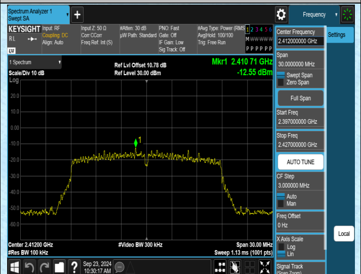
11N20MIMO-Ant2-2412-0~Reference-PASS
