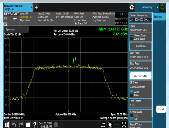
11N20SISO-Ant2-2412-0~Reference-PASS
