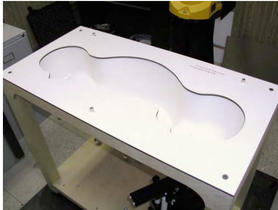
Figure 3-2 SAM Phantom
