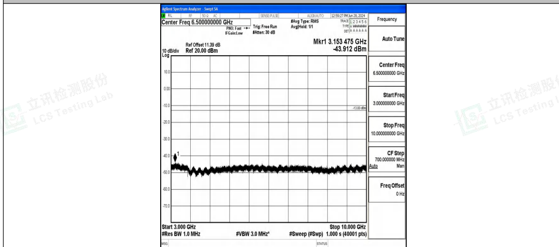
Band12_10MHz_16QAM_23095_1RB#0_3000~10000_3000~10000
