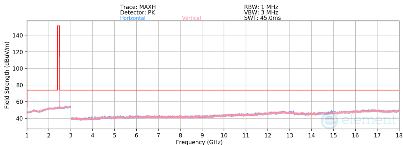
Plot 7-86. Radiated Spurious Emissions 1-18GHz Antenna WF2b (1Mbps ePA – Ch. 39)
