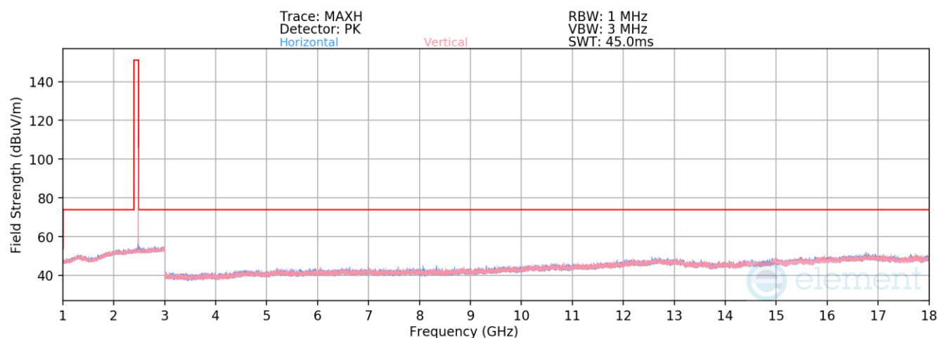
Plot 7-83. Radiated Spurious Emissions 1-18GHz Antenna WF7b (1Mbps ePA – Ch. 39)
