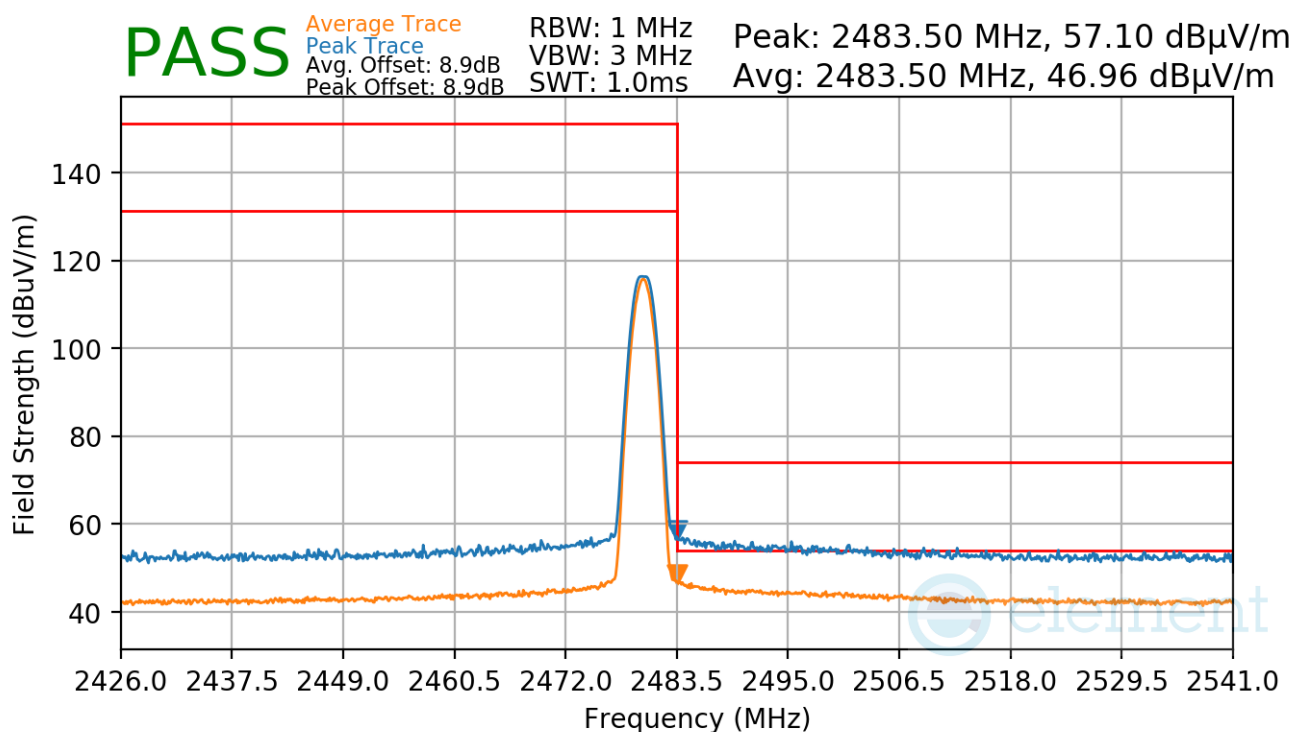
Plot 7-96. Radiated Restricted Upper Band Edge Measurement Antenna WF2b (Average & Peak)
