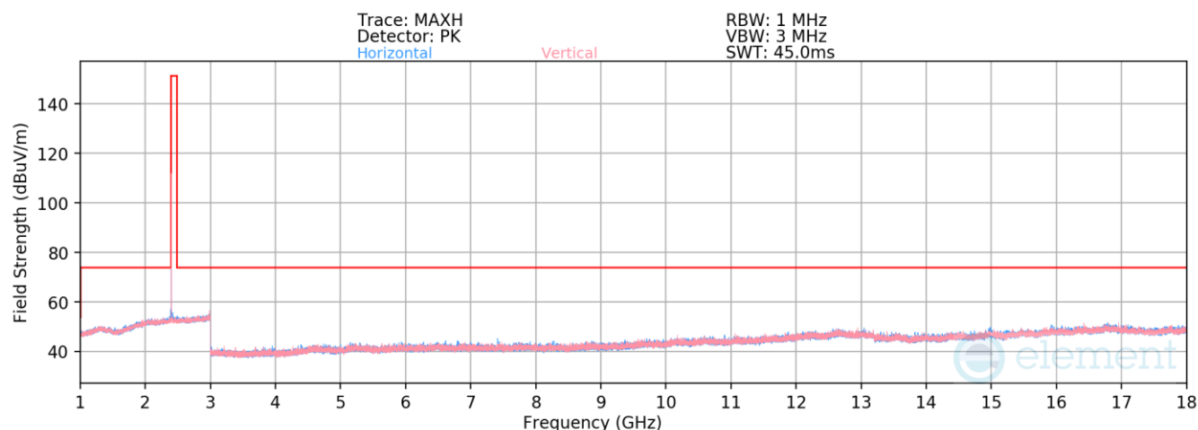
Plot 7-87. Radiated Spurious Emissions 1-18GHz TxBF (1Mbps, ePA – Ch. 0)
